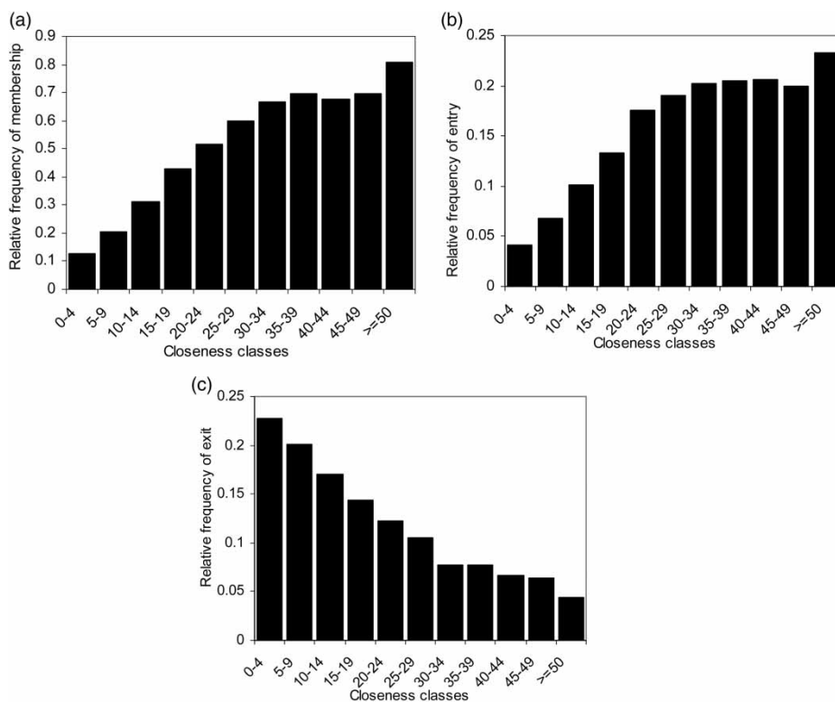
Fig. 4. Probabilities of membership (a), entry (b) and exit (c)
