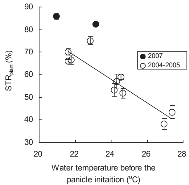
Fig. 3. Relationship between low temperature-induced sterility based on the whole plant ( STR_{plant} ) and water temperature during vegetative growth (from transplanting to panicle initiation). Data in 2004-2005 was obtained from the results of Shimono et al. (2007c) where the sterility of rice cultivar 'Sasanishiki' was induced by cool water during reproductive growth (19.5°C, 30 cm in depth, for about two months until the all panicles had emerged above water level) and fertilizer was supplied at N=0.6 g, P_2O_5=12 g, K_2O=0.8 g per pot. Regression line was drawn for the data of 2004-2005 ( y=-5.1732x+182.14 , R^2=0.830 , P<0.001 ). Bars indicate standard errors ( n=6 (2007) or 4 (2004-2005)).
