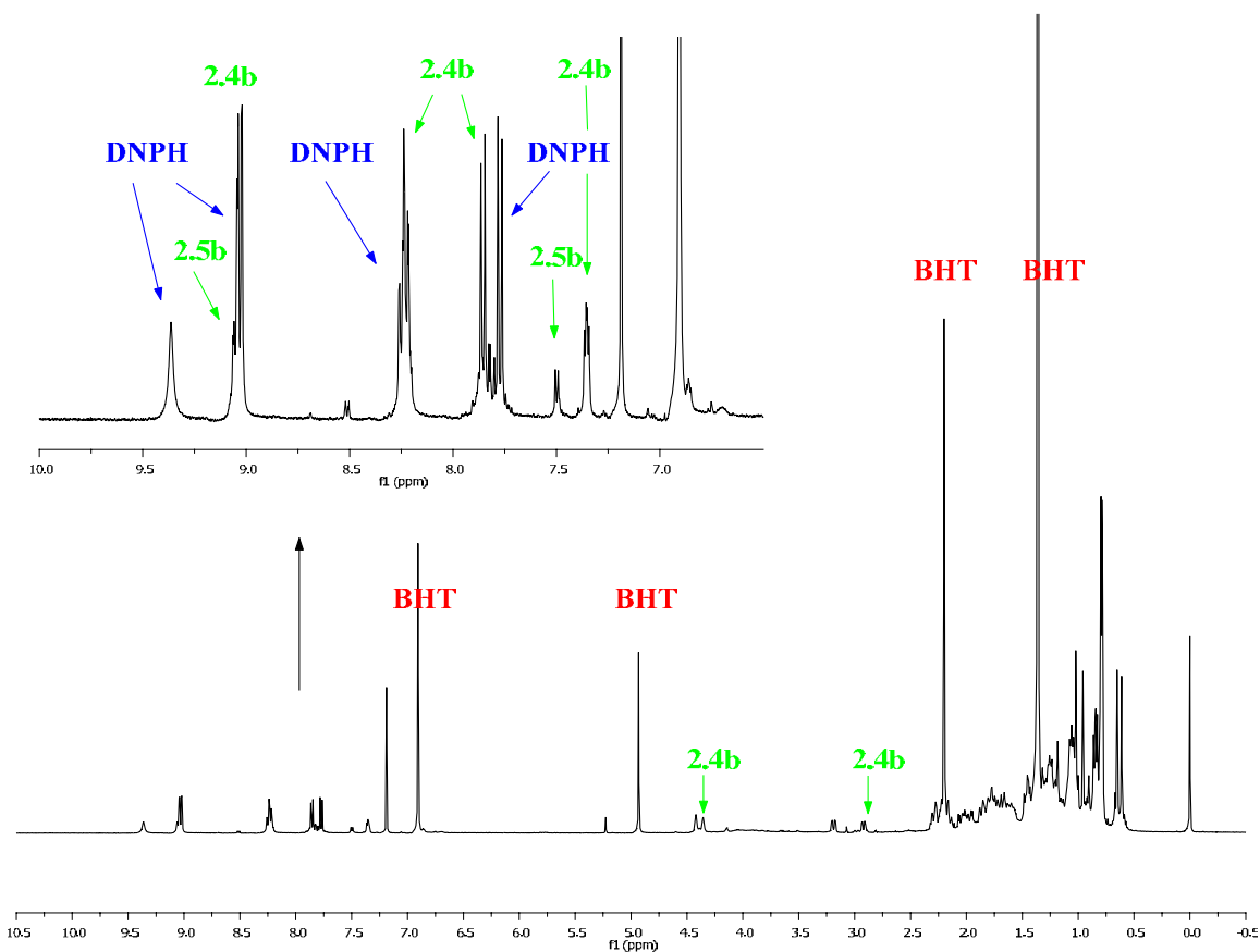
Figure 2.13. 1 H-NMR spectrum of the mixture of 2.4b and 2.5b in CDCl 3 2 hours after subjecting 2.4a to the DNP H derivatization conditions followed by work-up. Obtained at 500 MHz with chemical shifts reported in ppm relative to TMS.
