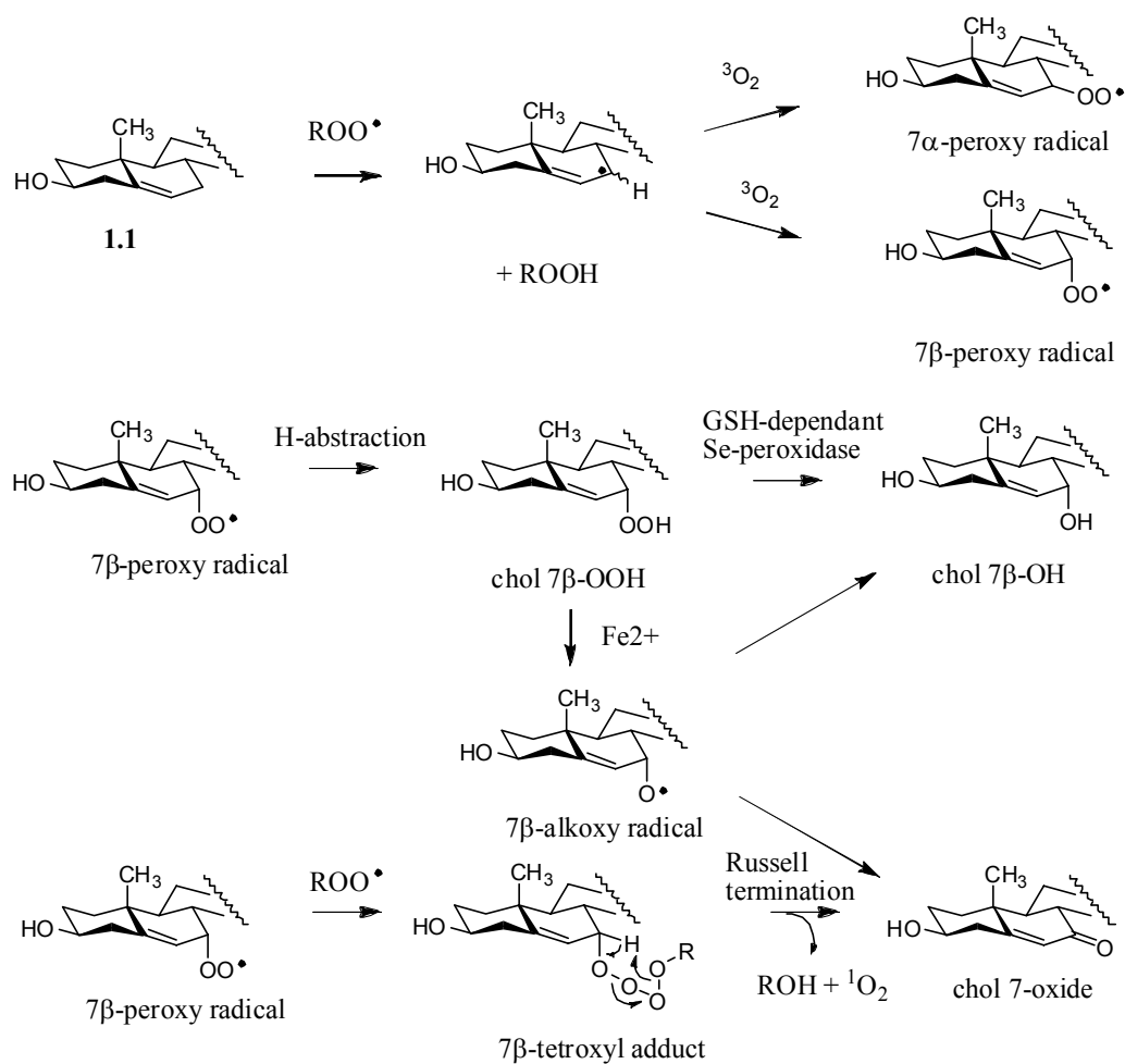
Scheme 1.6. Primary cholesterol autoxidation products formed in vivo . The C and D ring are not shown for clarity.
