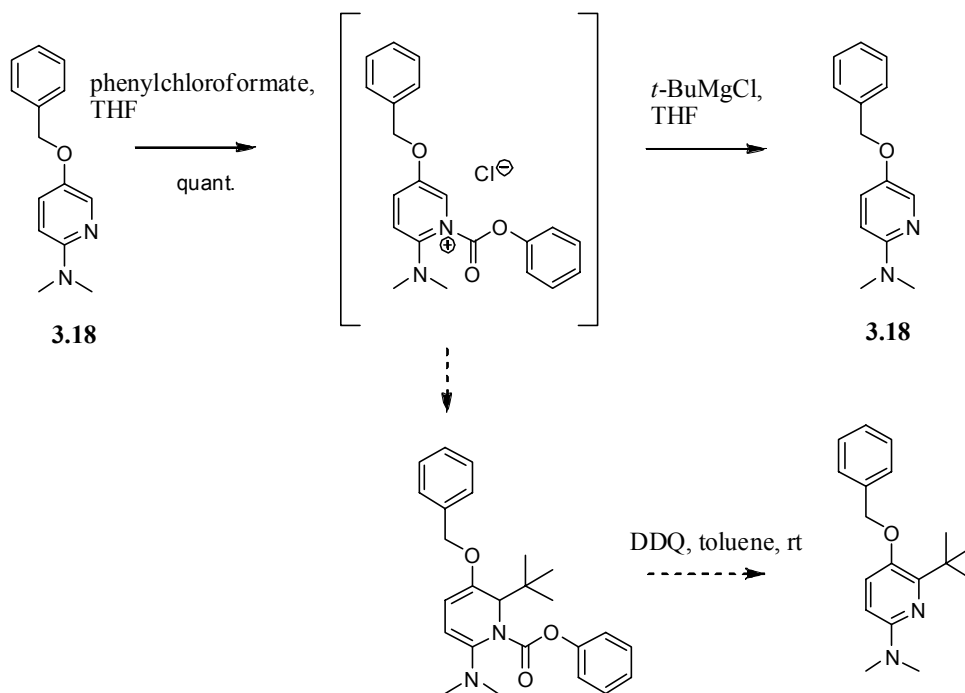
Scheme 3.25. Alkylation attempt and subsequent re-aromatization of 4- tert -butyl-3-(benzyloxy)pyridine-1(4H)-carboxylate.
