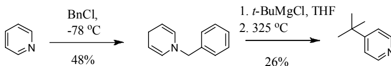
Scheme 3.11. Alkylation of pyridine with Grignard reagent via the N-benzyl dihydropyridine according to literature procedure.
