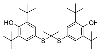
Probucol
