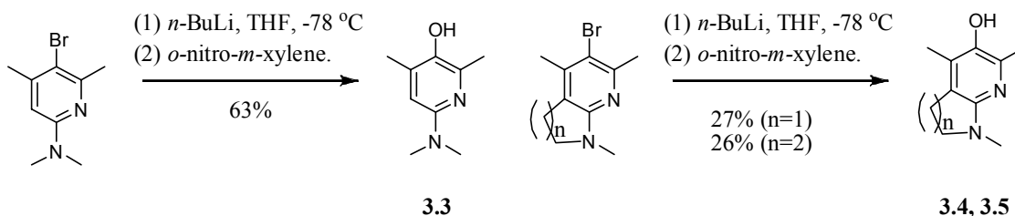
Scheme 3.8. 3-Pyridinols prepared by lithium/halogen exchange from the corresponding pyridyl bromide followed by oxidation with a nitroarene.
