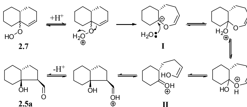
Scheme 2.8. The proposed mechanism of Hock cleavage of cholesterol 5 \alpha -OOH in non-participating solvents. Substituents are omitted on both the A and B ring of cholesterol for clarity.
