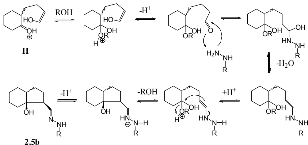
Scheme 2.10. Hock cleavage of 2.7 under DNPH derivatization conditions. Formation of oxocarbenium II , capture by alcoholic solvent, subsequent DNPH derivatization and closing acid catalyzed closing of the enamine resulting in 2.5b .
