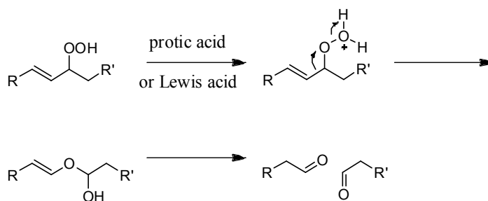
Scheme 2.6. \beta -Fragmentation of an alkoxy derived formal allylic hydroperoxide.
