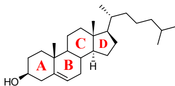
Cholesterol 1.1
