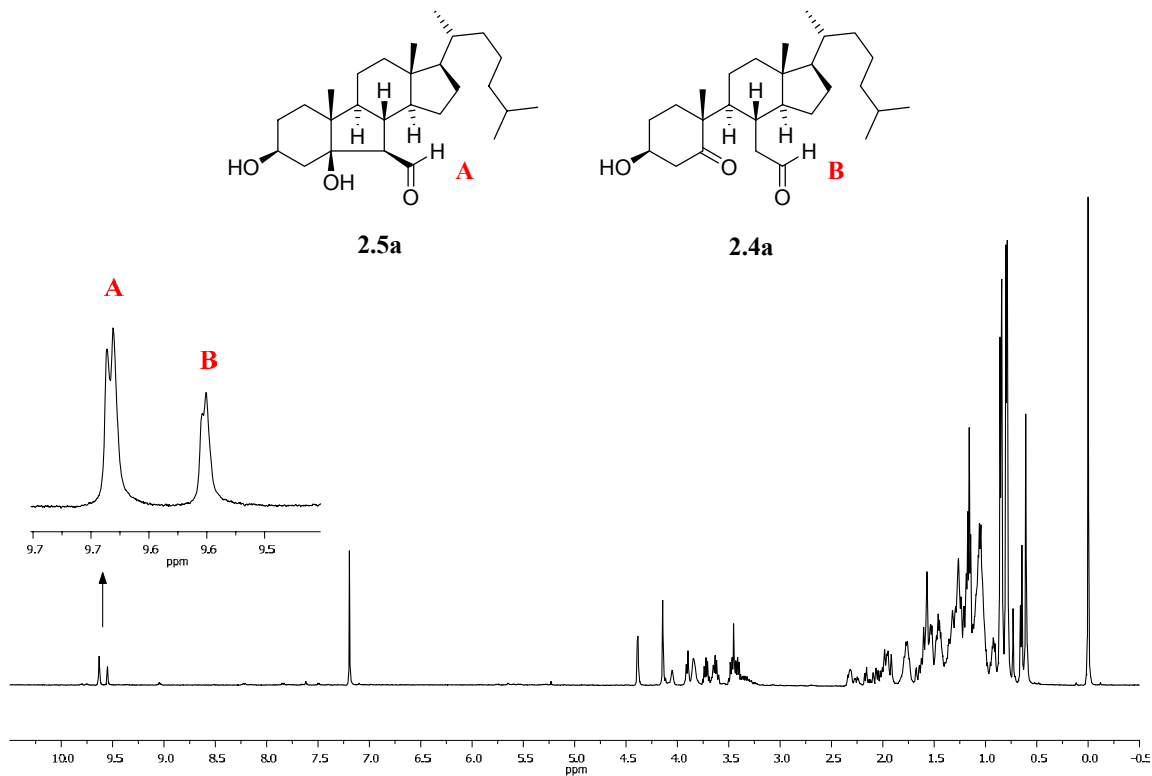
Figure 2.4. ^1\text{H-NMR} spectrum of the reaction products obtained from treatment of 2.7 with HCl (conc.) in EtOH, analyzed after workup. Obtained at 500 MHz in \text{CDCl}_3 with chemical shifts reported in ppm relative to TMS.
