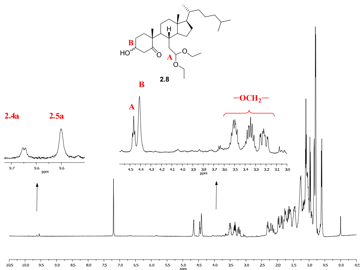
Figure 2.5. ^1\text{H-NMR} spectrum of 2.8 , the acetal derived from 2.4a , in \text{CDCl}_3 . Note that some 2.5a is formed due to aldolization of 2.4a upon acetalization. Obtained at 500 MHz with chemical shifts reported in ppm relative to TMS.
