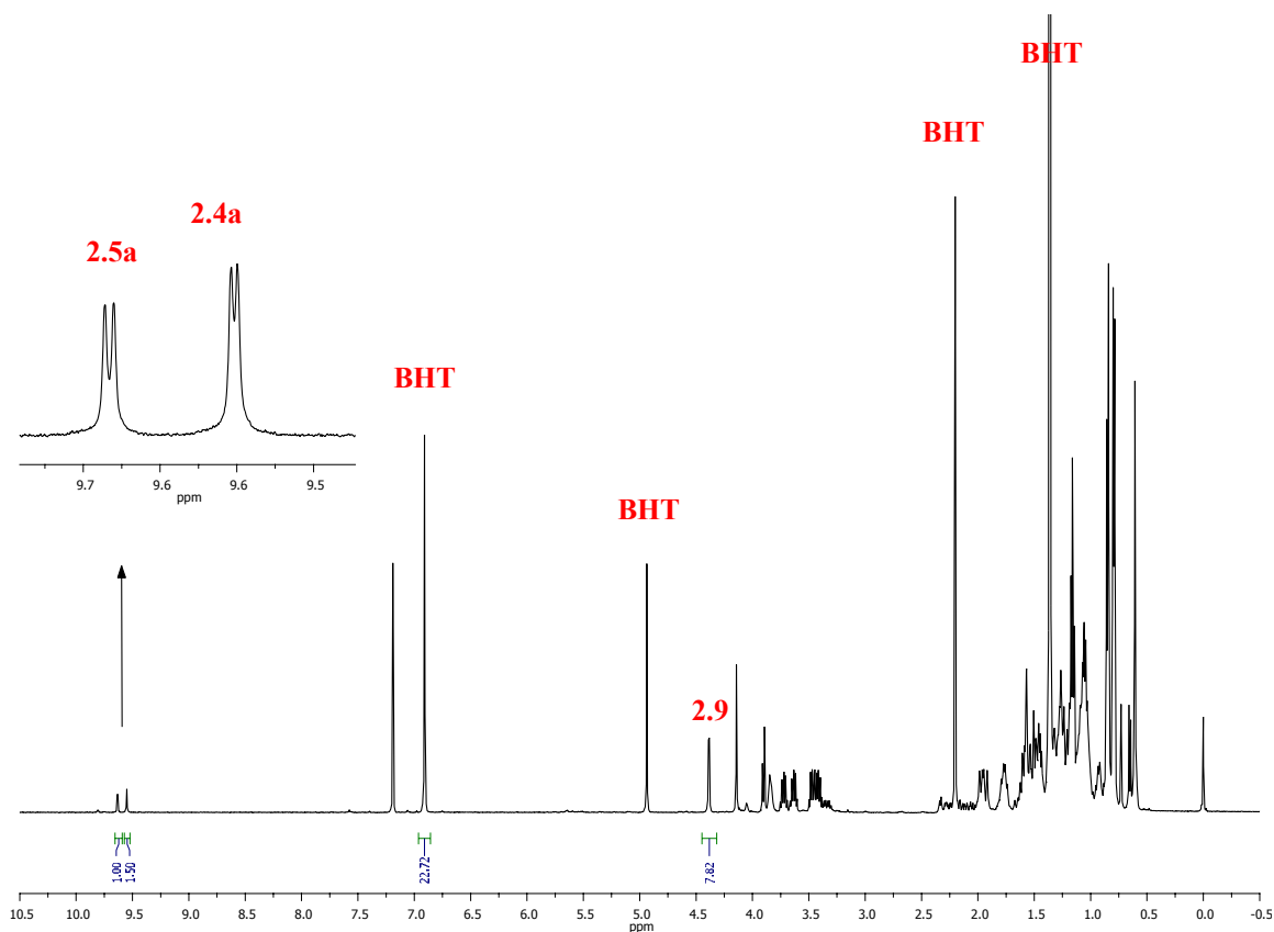
Figure 2.7. ^1\text{H-NMR} spectrum of the mixture of 2.4a , 2.5a and 2.9a formed upon treatment of 2.7 with HCl in EtOH. Obtained at 500 MHz with chemical shifts reported in ppm relative to TMS.
