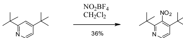
Scheme 3.10. Nitration of the 3 position in 2,4-di- tert -butylpyridine.
