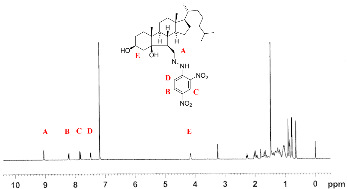
Figure 2.14. 1 H-NMR spectrum of authentic DNPH derivatized secosterol 2.4b . Obtained at 500 MHz with chemical shifts reported in ppm relative to TMS.
