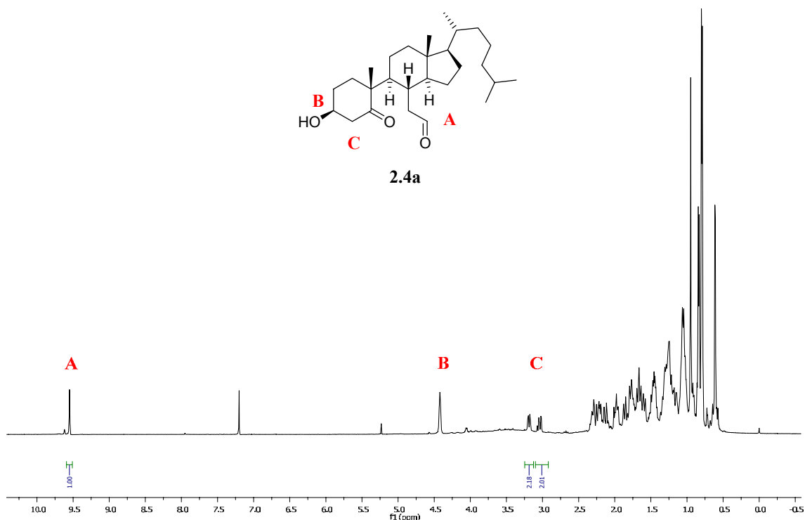
Figure 2.3. 1 H-NMR spectrum of the cholesterol 5,6-secosterol 2.4a in CDCl 3 . Obtained at 500 MHz with chemical shifts reported in ppm relative to TMS. Note that some 2.5a is formed due to aldolization of 2.4a in the NMR sample.
