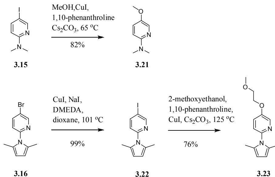
Scheme 3.24. O-alkyl ethers of 6-amino-3-pyridinol derivatives synthesized by Ullmann coupling and used as starting materials for alkylation chemistry.
