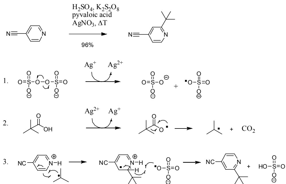
Scheme 3.13. A typical example of the radical alkylation chemistry of pyridines as developed by Minisci and co-workers. Here the t -butylation of 4-cyanopyridine is shown.
