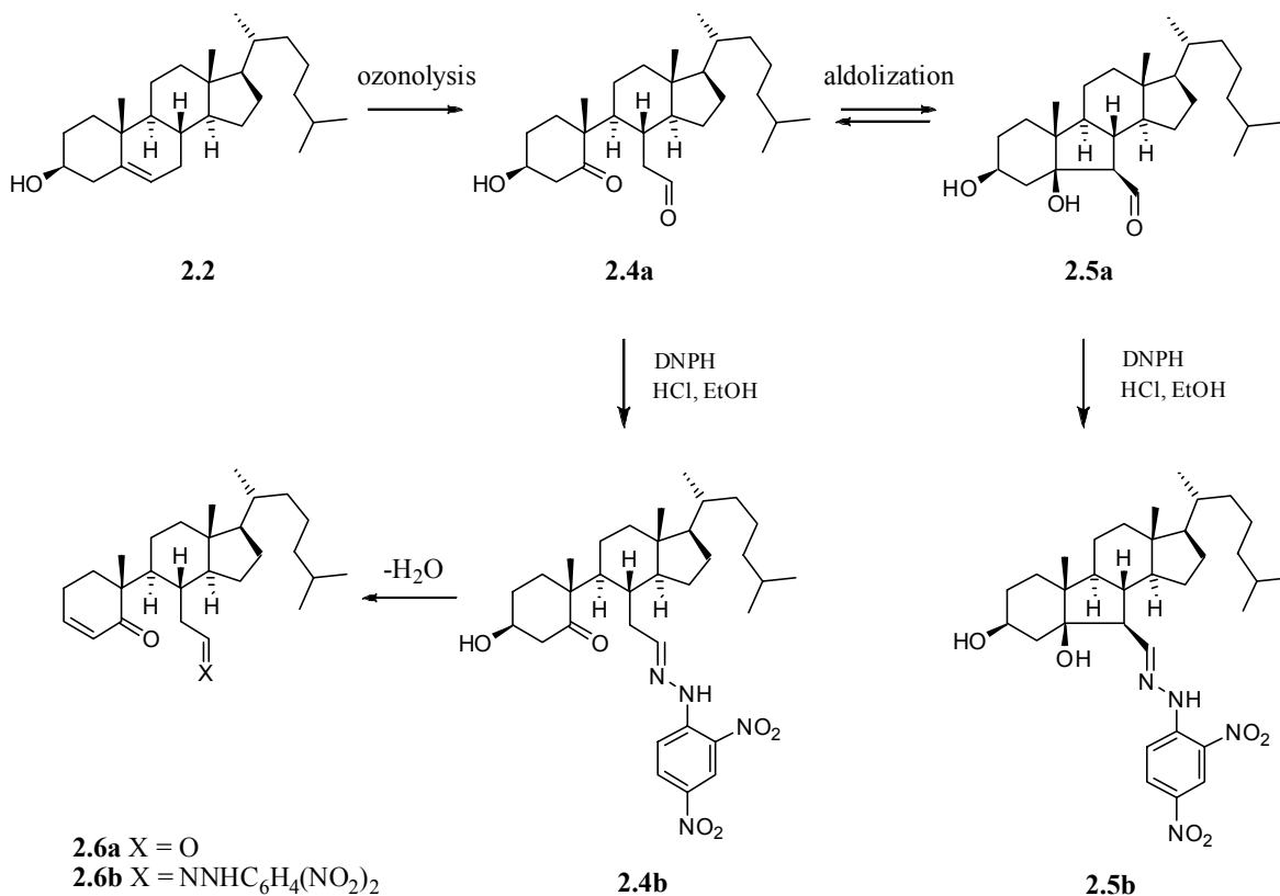
Scheme 2.3. Cholesterol ozonolysis products and their DNPH derivatives.
