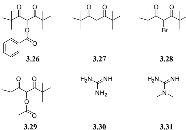
Scheme 3.30. Compounds used as reagents for the condensation reactions to form pyridiminol 3.6a or 3.6b .
