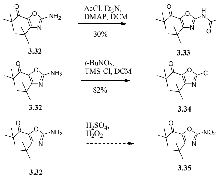
Scheme 3.33. Acetylation, chloro-diazotization and oxidation of oxazole 3.32 .
