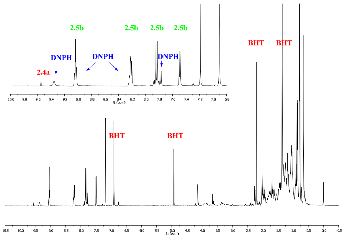
Figure 2.12. ^1\text{H-NMR} spectrum of the mixture of 2.4a and 2.5b in \text{CDCl}_3 2 hours after subjecting 2.7 to the DNPH derivatization conditions followed by work-up. Obtained at 500 MHz with chemical shifts reported in ppm relative to TMS.
