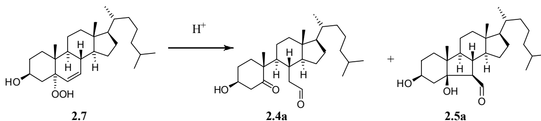
Scheme 2.4. Cholesterol 5 \alpha -hydroperoxide upon reaction with acid forms aldehydes 2.4a and 2.5a
