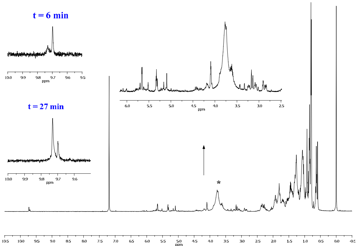
Figure 2.17. 1 H-NMR spectrum of chol 7α-OOH in CDCl 3 following treatment with TFA (2.7 mM). Insets show aldehydes peaks distribution at t = 6 minutes and t = 27 minutes. Obtained at 500 MHz with chemical shifts reported in ppm relative to TMS. (* = H 2 O).
