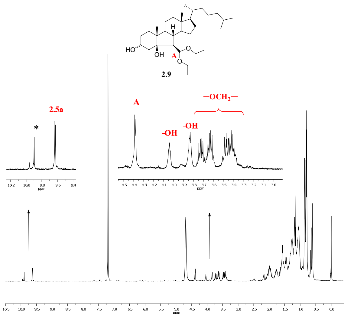
Figure 2.6. ^1\text{H-NMR} spectrum of 2.9 , the acetal derived from 2.5a in \text{CDCl}_3 . Note that some dehydration product (*) is formed on treatment of 2.5a with acid for acetalization (confirmed by LC/MS vide infra ). Spectrum obtained at 500 MHz with chemical shifts reported in ppm relative to TMS.
