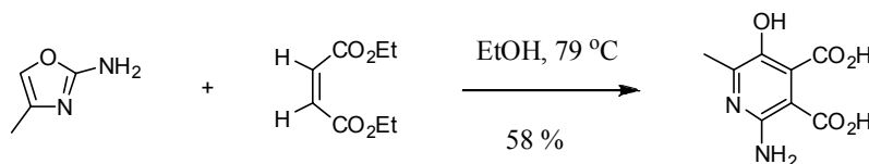
Scheme 3.5. The reaction of 2-amino-5-methyloxazole with diethylmaleate to form 2-amino-5-hydroxy-6-methylpyridine-3,4-dicarboxylic acid.
