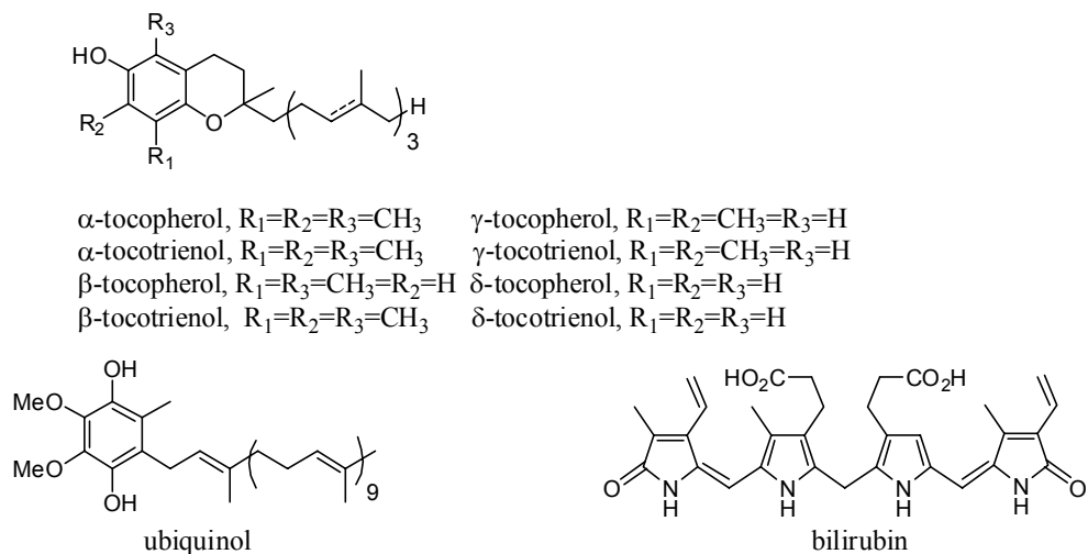
Scheme 1.11. Several different lipophilic antioxidants present in low density lipoprotein particles in human serum.
