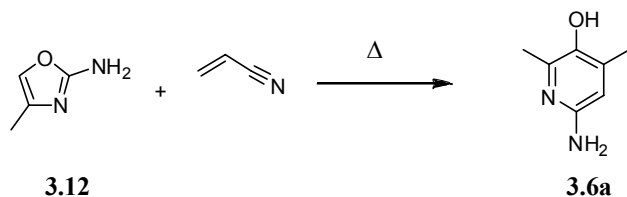
Scheme 3.21. Desired reaction of model oxazole 3.12 .
