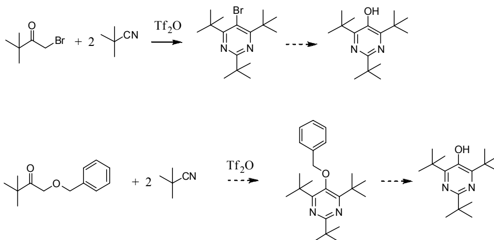
Scheme 3.19. Synthetic routes to access tri- tert -butylated pyrimidinol starting with termolecular synthesis of the pyrimidine ring system.
