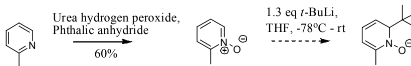
Scheme 3.27. The synthesis of picoline N-oxide followed by alkylation attempt using t -butyllithium.
