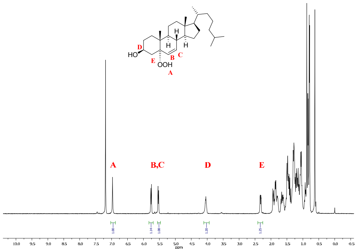
Figure 2.1. ^1\text{H-NMR} spectrum of cholesterol 5\alpha -hydroperoxide in \text{CDCl}_3 . Obtained at 500 MHz with chemical shifts reported in ppm relative to tetramethylsilane (TMS).
