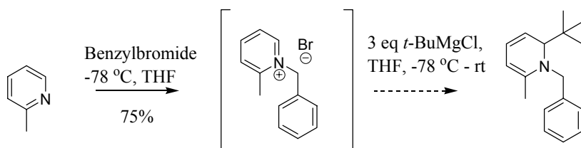
Scheme 3.26. Turning picoline into its benzyl quaternary ammonium salt followed by alkylation attempt with Grignard reagent.
