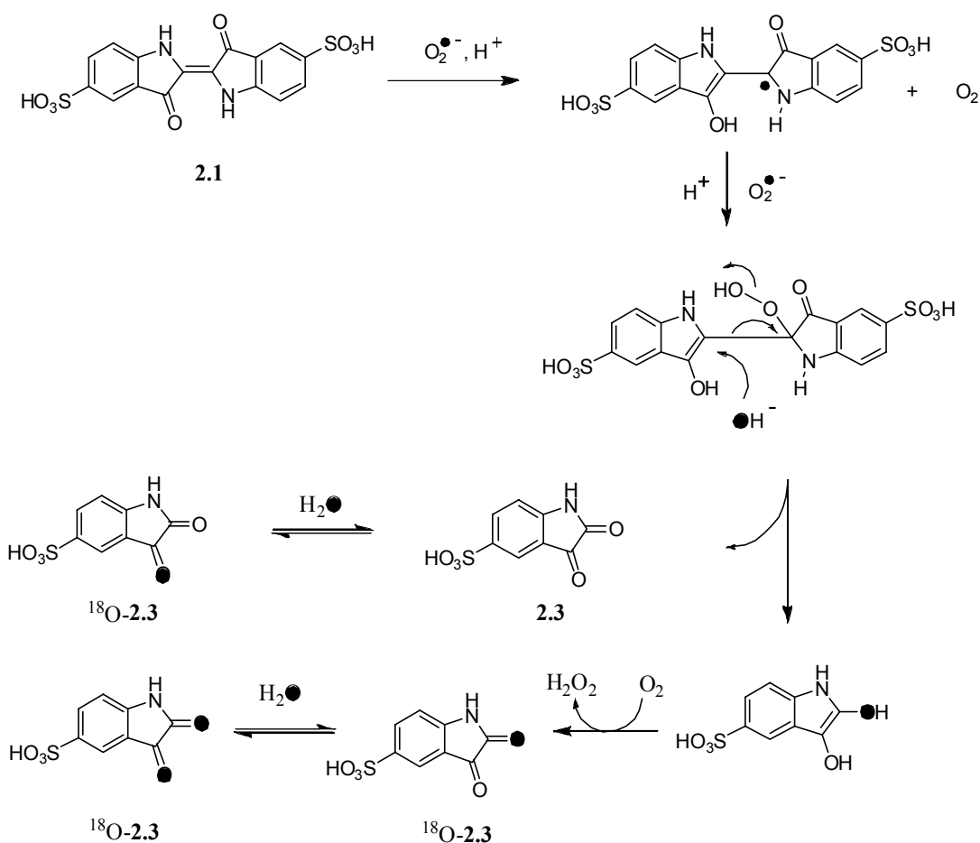
Scheme 2.13. The reaction of superoxide with indigo carmine as proposed by Winterbourn and co-workers. 30
