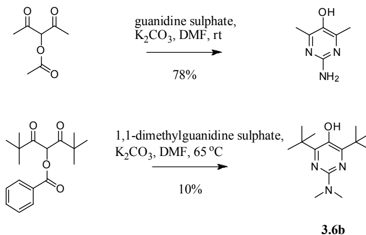
Scheme 3.15. An example of the condensation of a \beta -diketone with an urea to form a substituted pyrimidinol.
