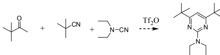
Scheme 3.20. Envisioned reaction using diethylcyanamide to introduce an amine moiety at the 2-position of a tert -butylated pyrimidine ring system.
