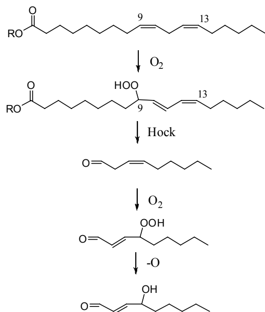
Scheme 1.10. Hock fragmentation of 9-hydroperoxide octadecanoic acid, on the primary linoleate autoxidation products, to give 4-hydro( peroxy)nonenal.
