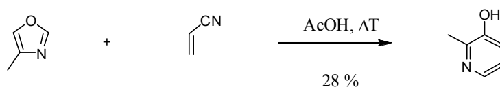
Scheme 3.4. Example of the pyridinol synthesis as performed by Naito and co-workers.
