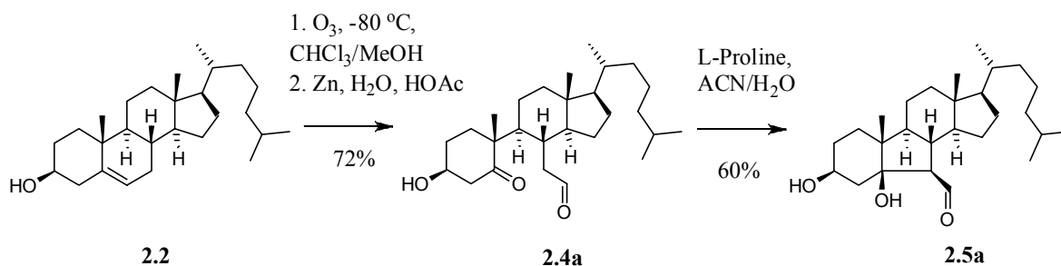
Scheme 2.5. Preparation of authentic 2.4a via ozonolysis of cholesterol and L-proline catalyzed intramolecular aldolization to yield 2.5a .
