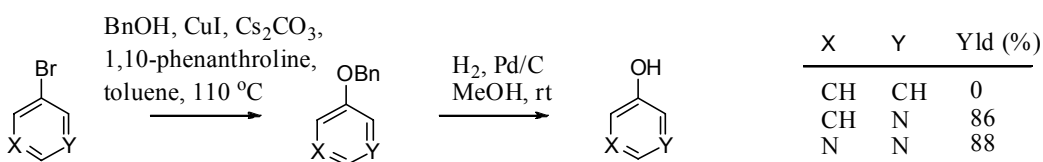
Scheme 3.9. 3-Pyridinols prepared by benzyloxylation of the corresponding pyridyl bromide followed by catalytic hydrogenation.
