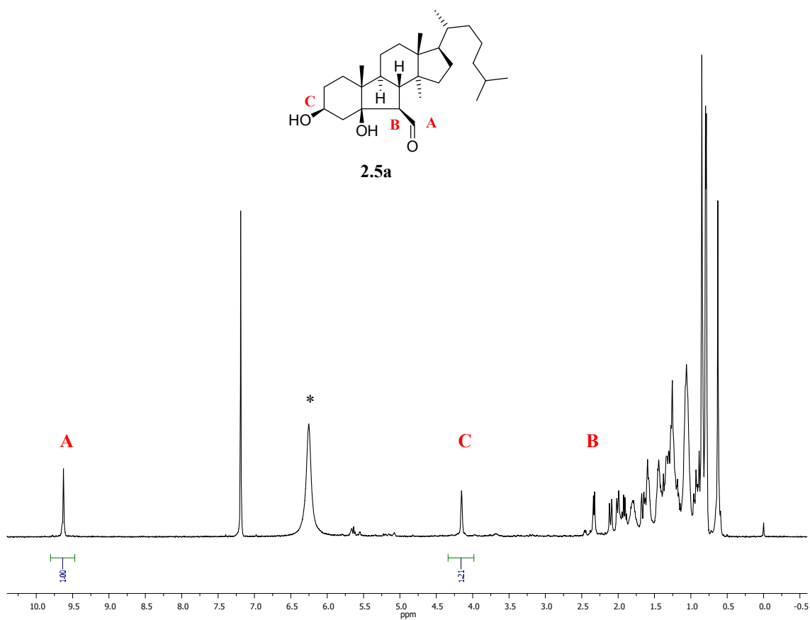
Figure 2.2. 1 H-NMR spectrum of 2.7 in CDCl 3 following treatment with a drop of TFA. Obtained at 500 MHz with chemical shifts reported in ppm relative to TMS. (* = H 2 O).
