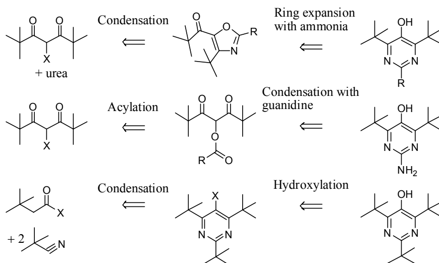
Scheme 3.14. Retrosynthetic pathways to access 2,4-di- tert -butyl-3-pyrimidinols.
