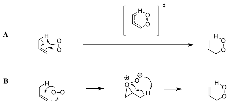
Scheme 1.5. A; Classical mechanism of the reaction of singlet oxygen with an allylic substrate through a pericyclic ene reaction mechanism. B; Modern step-wise (no intermediate) mechanism based on KIE mechanistic studies. Both pathways show the allylic hydroperoxide product with migration of the double bond. 34
