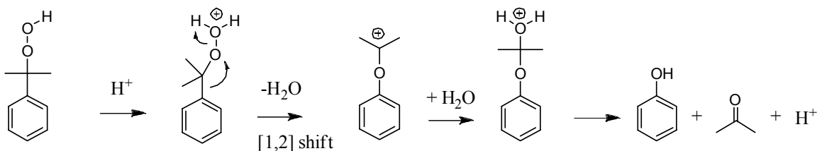
Scheme 1.9. Industrial synthesis of phenol and acetone from cumene hydroperoxide by acid-catalyzed Hock fragmentation.
