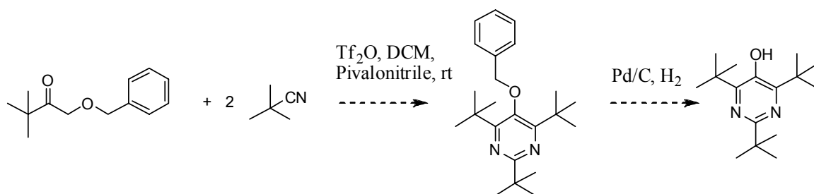
Scheme 3.36. Termolecular synthesis of the tert -butyl pyrimidine ring system with the benzyl ether in place.
