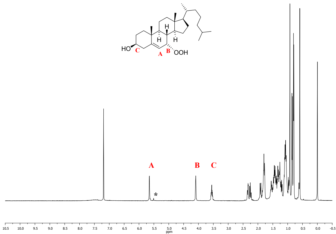
Figure 2.16. 1 H-NMR spectrum of cholesterol 7 \alpha -OOH in CDCl 3 . Obtained at 500 MHz with chemical shifts reported in ppm relative to TMS. (*Trace amount of chol 7 \beta -OOH).
