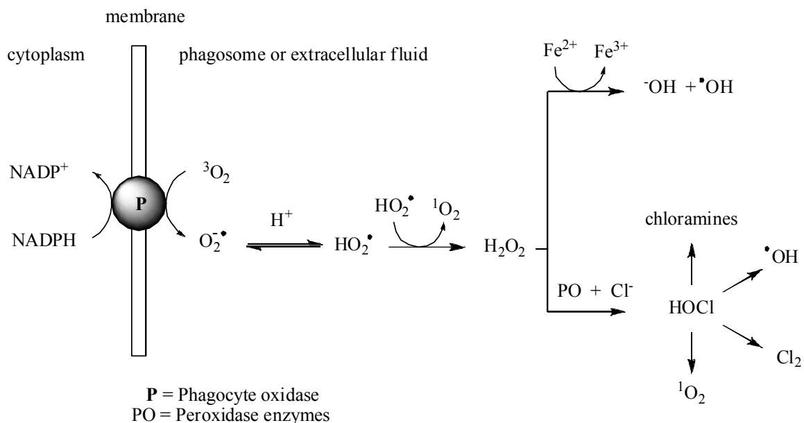
Scheme 2.1. The generation of ROS by phagocytes as part of the immune response.
