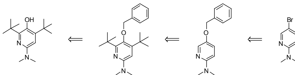
Scheme 3.12. Alkylation sequence envisioned with introduction of the hydroxyl group as protected benzyl ether in the first step.
