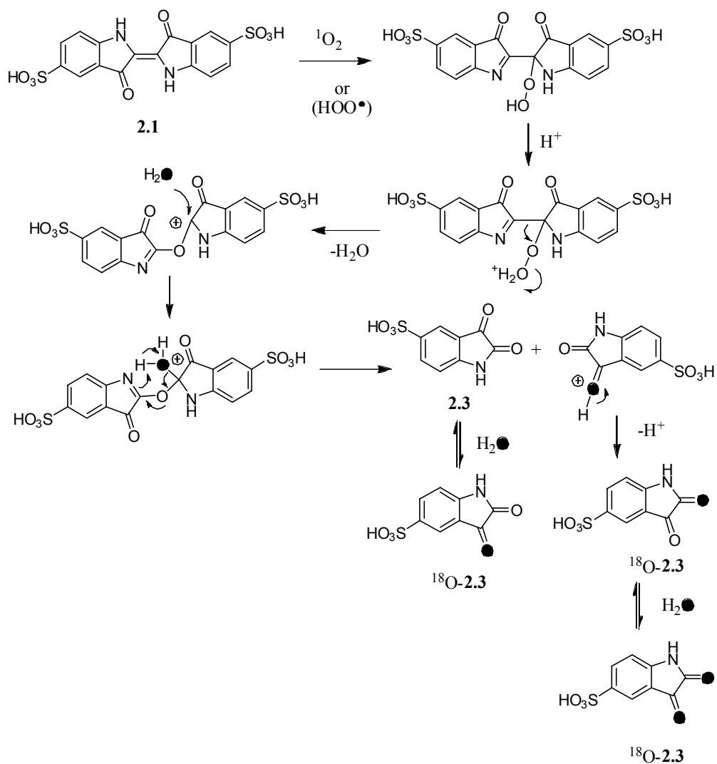
Scheme 2.14. Proposed cleavage of indigo carmine with singlet oxygen via Hock cleavage.
