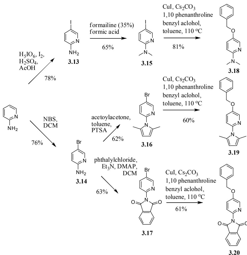
Scheme 3.22. O-Benzyl ethers of 2-amino-5-pyridinol derivatives synthesized by Ullmann coupling and used as starting materials for attempted alkylations.
