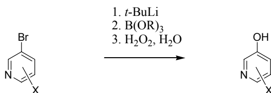
Scheme 3.7. Typical method of converting a pyridyl bromide to pyridyl alcohol.
