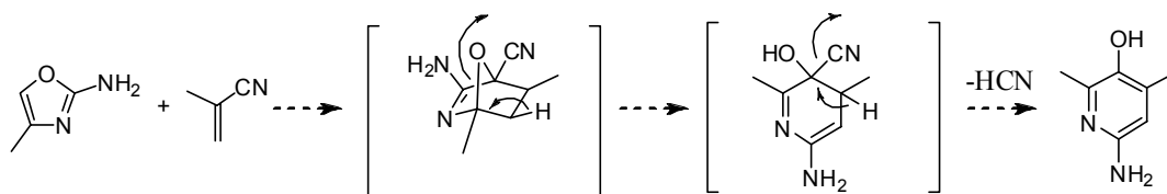
Scheme 3.6. Proposed Hetero Diels Alder reaction of 2-amino-5-methyloxazole with methacrylonitrile resulting in 6-amino-2,4-dimethyl-3-pyridinol.
