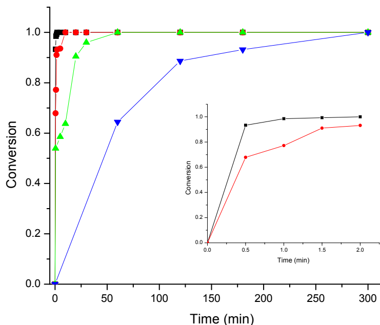
Figure 2.8. Conversion of cholesterol 5\alpha -OOH (4,8 mmol/ml in EtOH) to 2.4a and 2.5a as a function of time at different concentrations of HCl (■, 0.1 M; ●, 0.01 M; ▲, 0.001 M; ▼, 0.0001 M).
