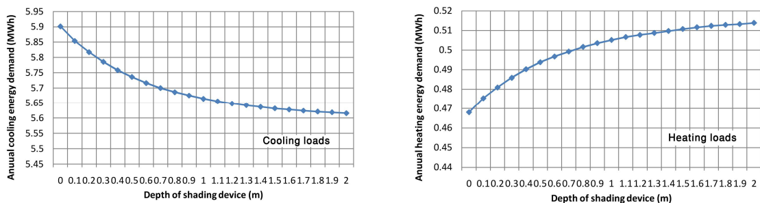
Fig. 5.12 : The total annual heating and cooling energy for west façade at different horizontal device depth Building model - BY IES VE
