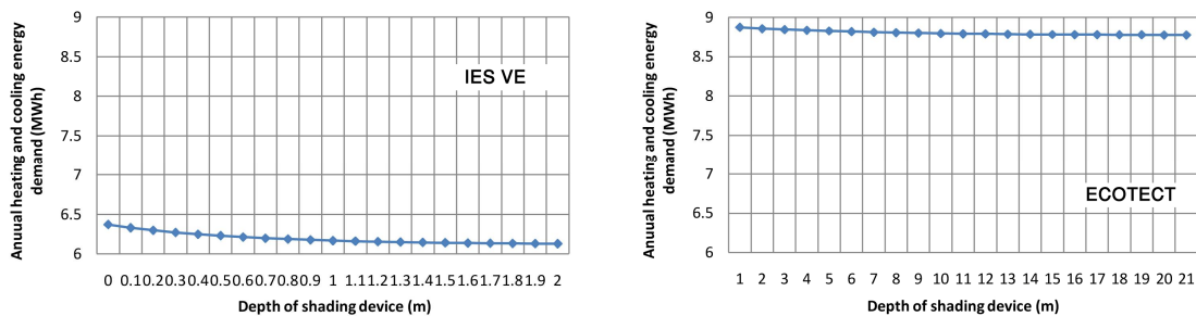
Fig. 5.13 : The overall annual heating and cooling energy for west façade at different horizontal device depth for Building model
