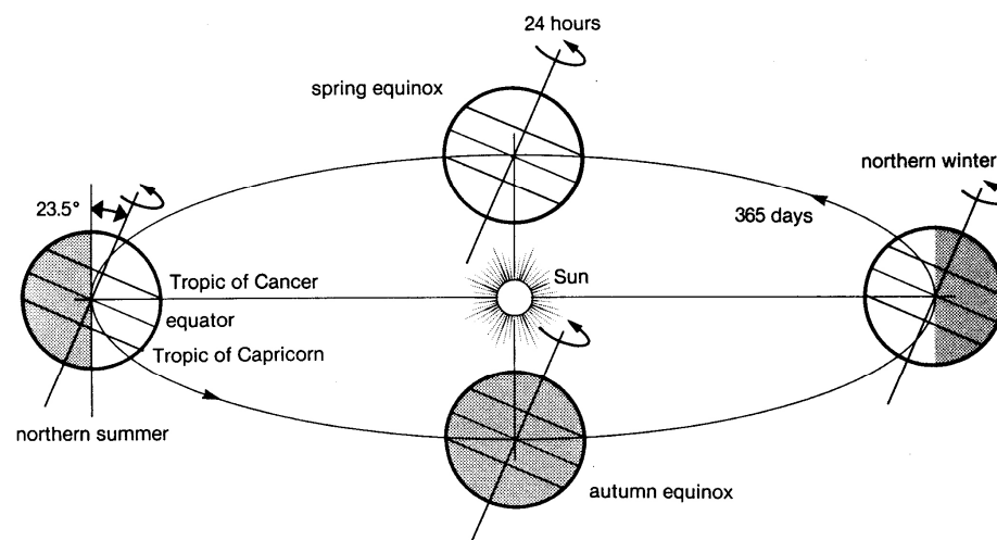
Fig. 3.9 : Sun-earth movement Source : (Baker, 1987)
