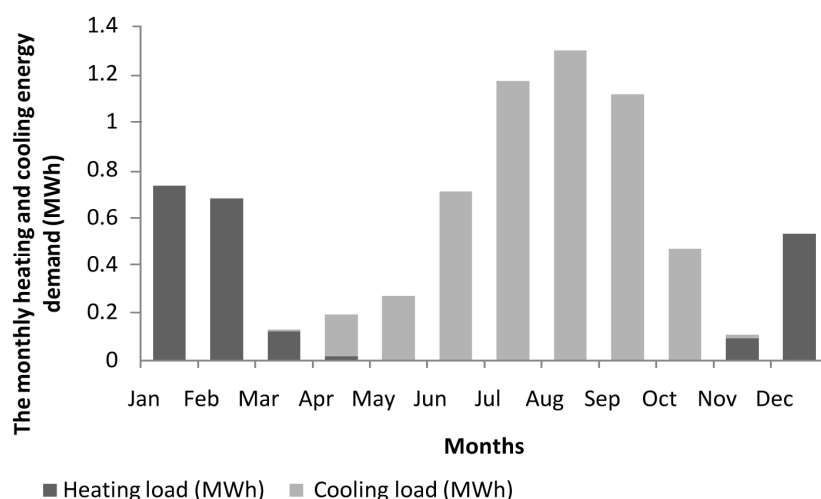
Fig. 5.1 : The monthly heating and cooling energy demands without shading devices Building model - BY ECOTECT
