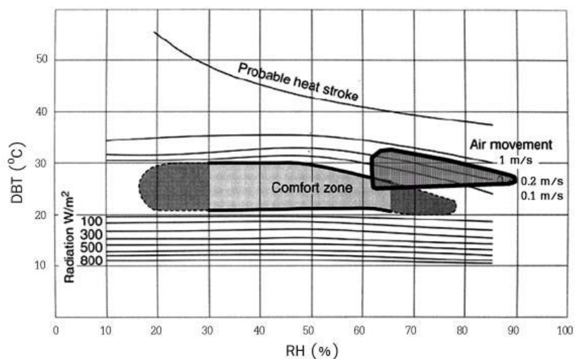
Fig. 2.8 : Olgyay’s bioclimatic chart modified for hot humid climates. The new comfort zone is shown on the right of the original one
