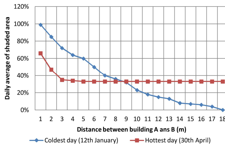
Fig. 5.23: The impact of changing distance (X) on average shaded area ECOTECT
