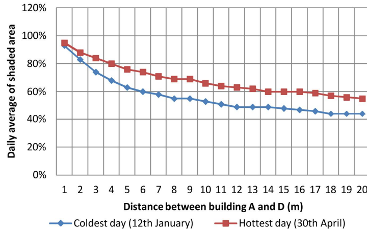
Fig. 5.25: The impact of changing distance (Z) on average shaded area ECOTECT
