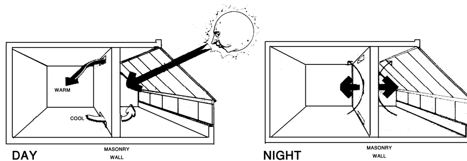
Fig. 2.19 : Indirect gain – attached sunspace Source : (Mazria, 1979)
