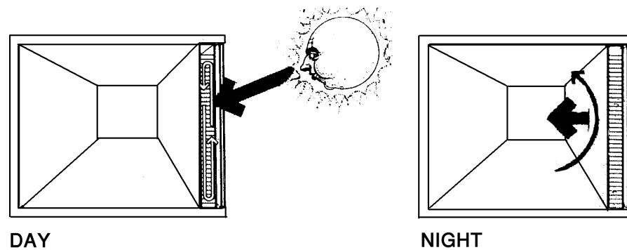
Fig. 2.18 : Indirect gain – water thermal storage wall Source : (Mazria, 1979)
