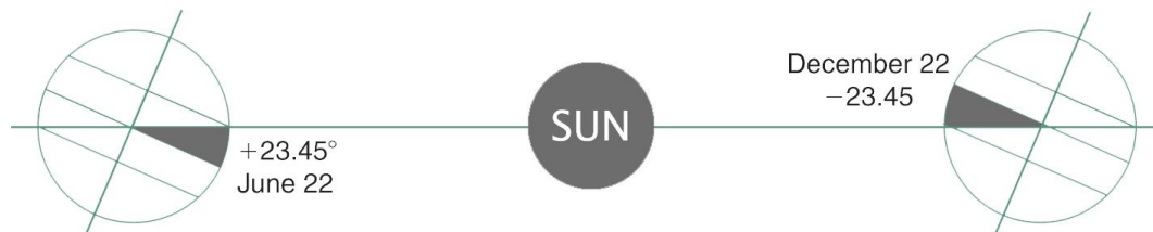
Fig. 3.10 : Two-dimension section of the earth's orbit Source : (Szokolay, 2004)
