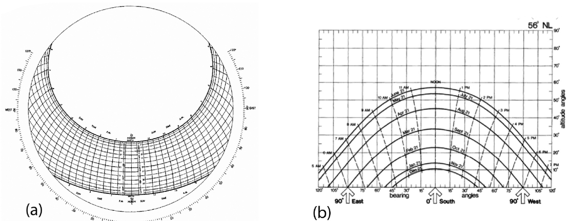
Fig. 3.21 : (a) Solar path diagram used by the Olgyays and (b) used by Mazria Source : (Dubois, 2000)
