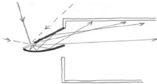
Figure 2.14: Light-guiding shade (LGS)
