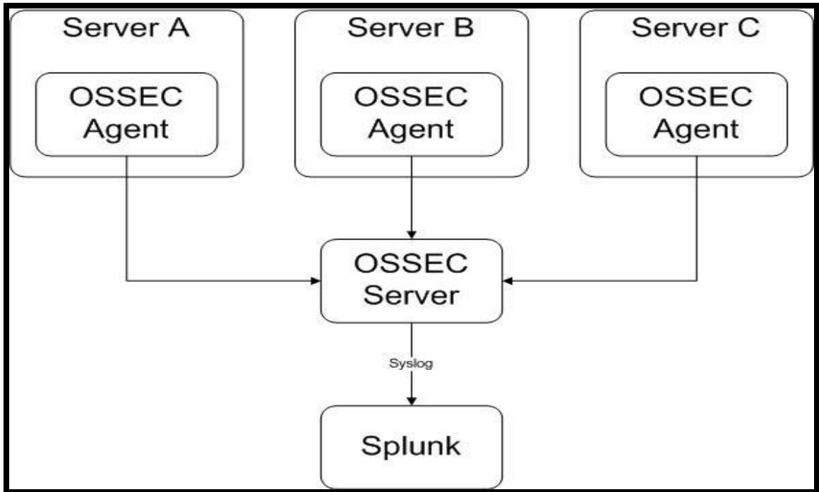
Figure 5.13: Splunk integration with OSSEC.
