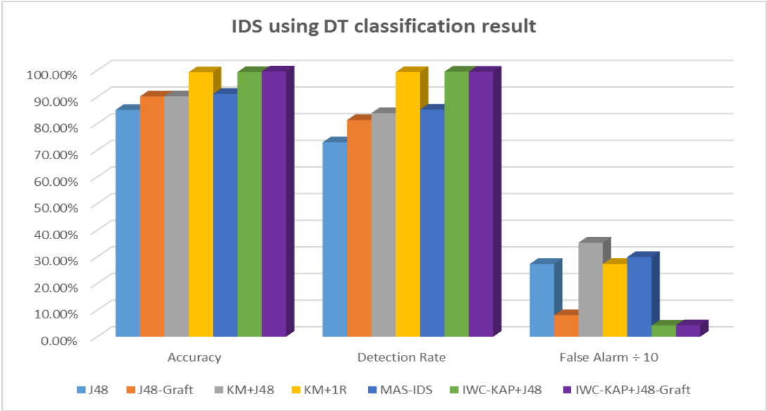
Figure 4.8 IDS using DT classification result
