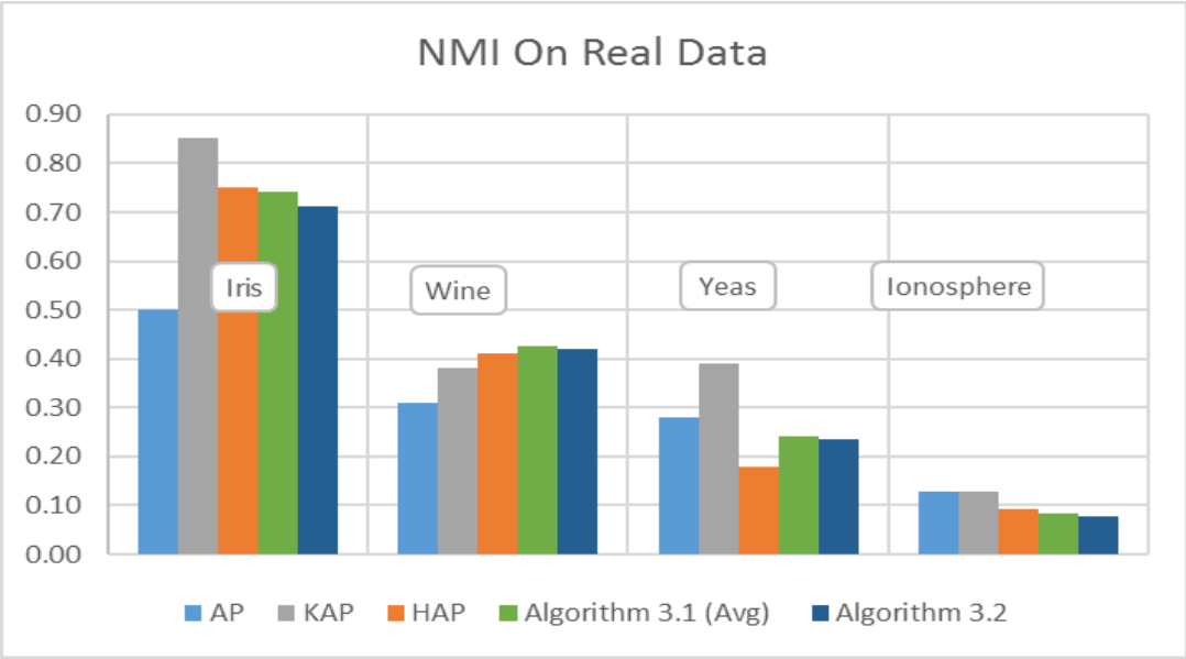
Figure 4.3 NMI of IWC-KAP Vs. AP, KAP, and HAP in real data set.
