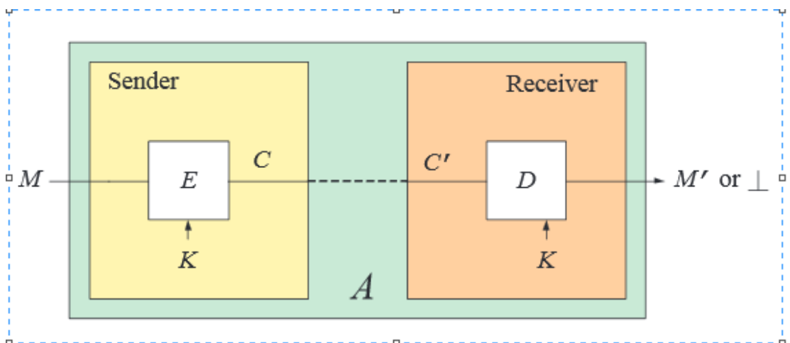
Figure 4.1 An authenticated-encryption
