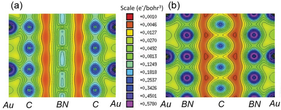
Figure 6.9 The valence charge density contours of (a) ABA-stacked graphene/BN/graphene, and (b) ABA-stacked BN/graphene/BN trilayers coupled with gold contacts.
