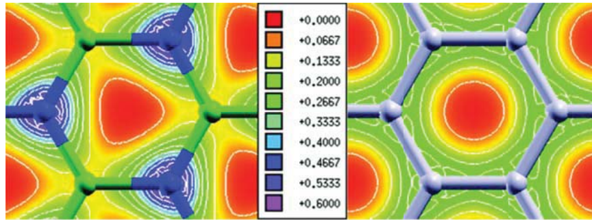
Figure 5.4 The valence band charge density contours of BN (left) and graphene (right) of the graphene/BN bilayer. The central panel shows the scale of charge density, in unit of e/\text{Bohr}^3 .
