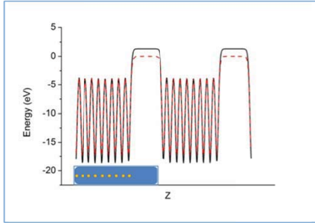
Figure 2.5 Nine layers of gold and vacuum fill in the unit cell, as shown in the insert. The z direction is along gold 111. The planer averaged VH (solid) and VNA (dashed) is plotted along z direction. Two unit cells are included in the plotting. The blue insert represents one repeating cell of the calculated model.
