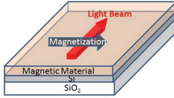
Fig. 1. Geometry of the slab waveguide structure under consideration
