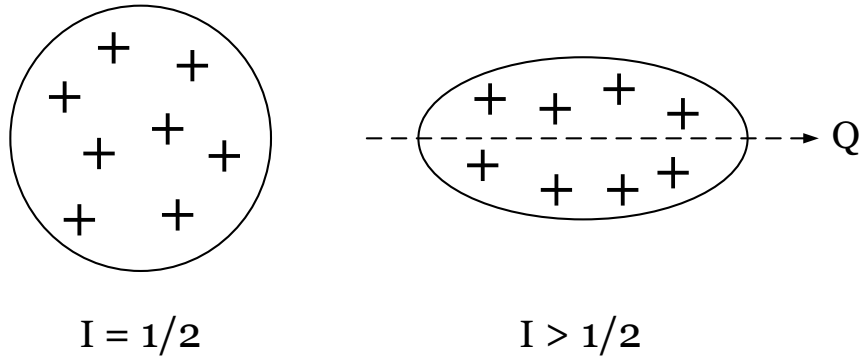
Figure 2.4: The charge distribution of nuclei with I = 1/2 and I > 1/2
