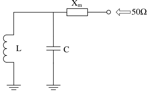
Figure 3.4: The NQR probe with 50Ω matching network
