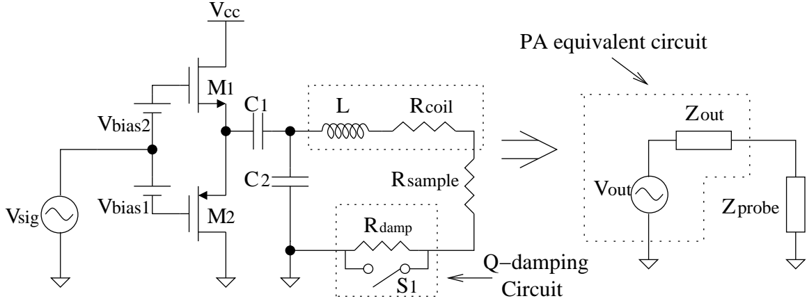
Figure 4.3: A class-AB type PA with a parallel LC matched RF probe and the equivalent circuit.
