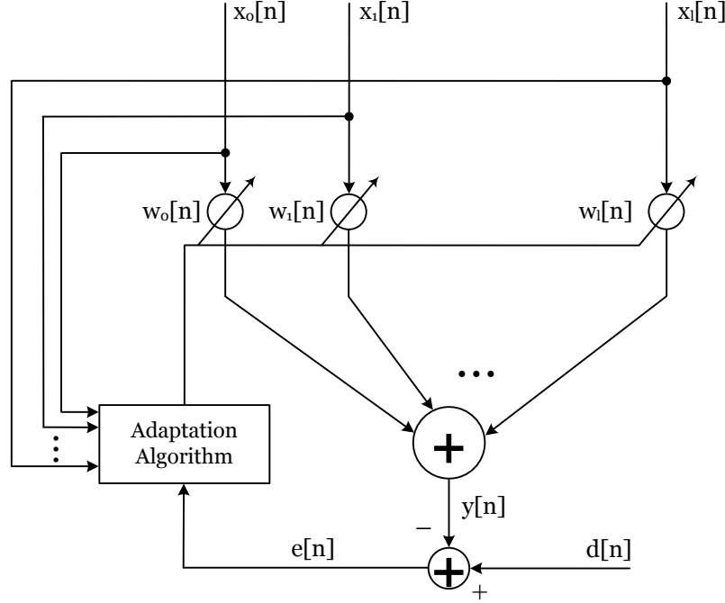
Figure 7.2: The adaptive spacial filter
