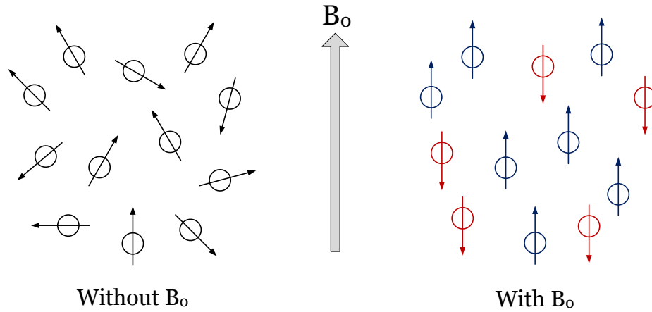
Figure 2.1: Magnetic dipole moments distribution with and without \mathbf{B}_0
