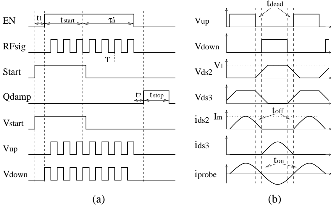
Figure 4.5: (a) Control signals and gate driving signals of the proposed PA circuit. (b) V_{gs} , V_{ds} and i_{ds} of M_2 and M_3 when f = f_o and t_{on} = t_{off} = t_{dead} .
