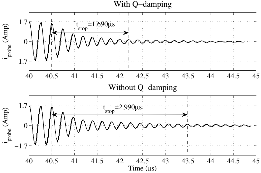
Figure 4.11: t_{\text{stop}} with and without Q-damping function.
