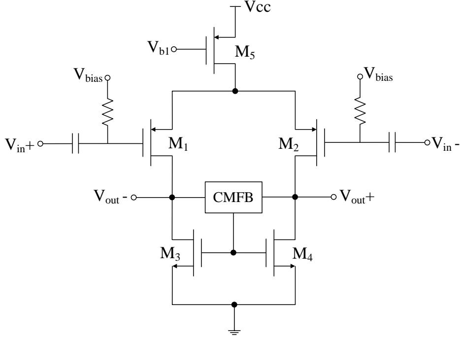
Figure 6.3: A differential low-noise amplifier
