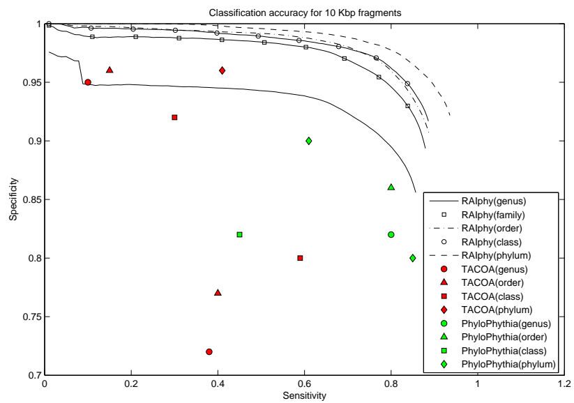
Figure 6.13: Sensitivity-specificity operating characteristics curves for RAIphy determined with 10 Kbp fragments using the dataset obtained from RefSeq database. The accuracy values for TACO and PhyloPythia are also illustrated for the same test data.
