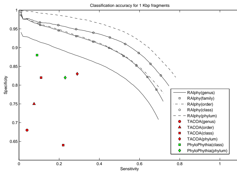
Figure 6.12: Sensitivity-specificity operating characteristics curves for RAIphy determined with 1 Kbp fragments using the dataset obtained from the RefSeq database. The accuracy values for TACO and PhyloPythia are also illustrated for the same test data.
