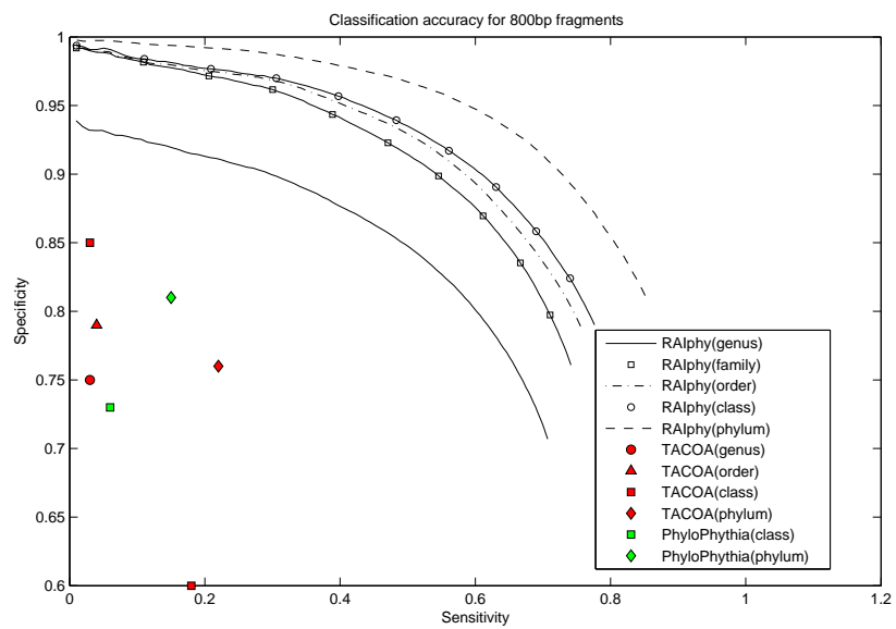
Figure 6.11: Sensitivity-specificity operating characteristics curves for RAIphy determined with 800 bp fragments using the dataset obtained from the RefSeq database. The accuracy values for TACO and PhyloPythia are also illustrated for the same test data
