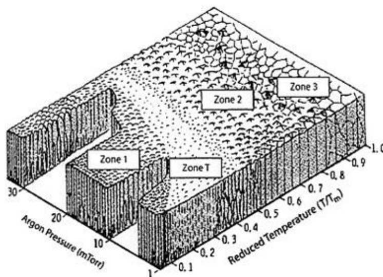
FIG. 2.5. Diagram of thin film zone structures. After Ref. 2.41.
