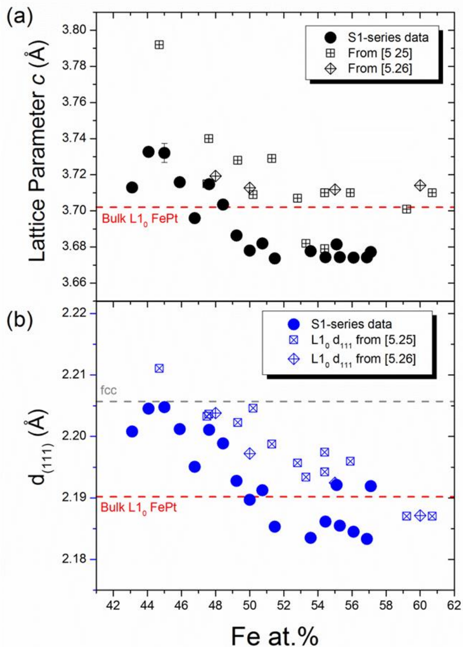
FIG. 4.3. (a) Lattice parameter c variations with stoichiometry. Red dashed line denotes the c -lattice parameter for bulk equiatomic L_{10} FePt. (b) Variations in lattice spacing determined from (111) XRD peak with stoichiometry. Grey dashed and red dashed lines denote the (111) d -space for equiatomic fcc and L_{10} bulk FePt, respectively.
