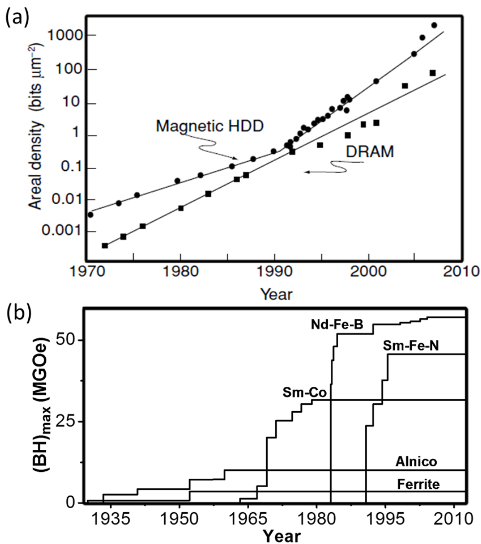
FIG. 1.1. Tracking the progress of magnetic material technologies: a) shows the improvements in areal density of magnetic recording ( 1 \text{ bit } \mu\text{m}^{-2} = 0.645 \text{ Gbit/in}^2 ) along with parallel progress in solid-state memory (DRAM); b) shows advancements in the strength of permanent magnets by the common metric of energy product, (BH)_{\text{max}} ( 100 \text{ kJ/m}^3 = 12.57 \text{ MGOe} ). Part (a) after Ref. 1.1.
