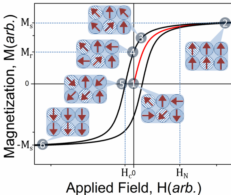
FIG. 2.1. Example of M(H) hysteresis loop, including diagrams of a six-grain proxy magnetic system for six different magnetization states along the hysteresis loop. See text for details.
