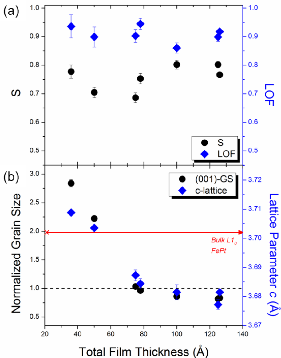
FIG. 4.15. Trends of S and LOF (a), and normalized grain size and c-lattice parameter (b), both with respect to total film thickness. The c-lattice parameter for bulk L1_0 FePt is included as the solid red line in (b). The dashed grey line marks a normalized grain size equal to the nominal film thickness.
