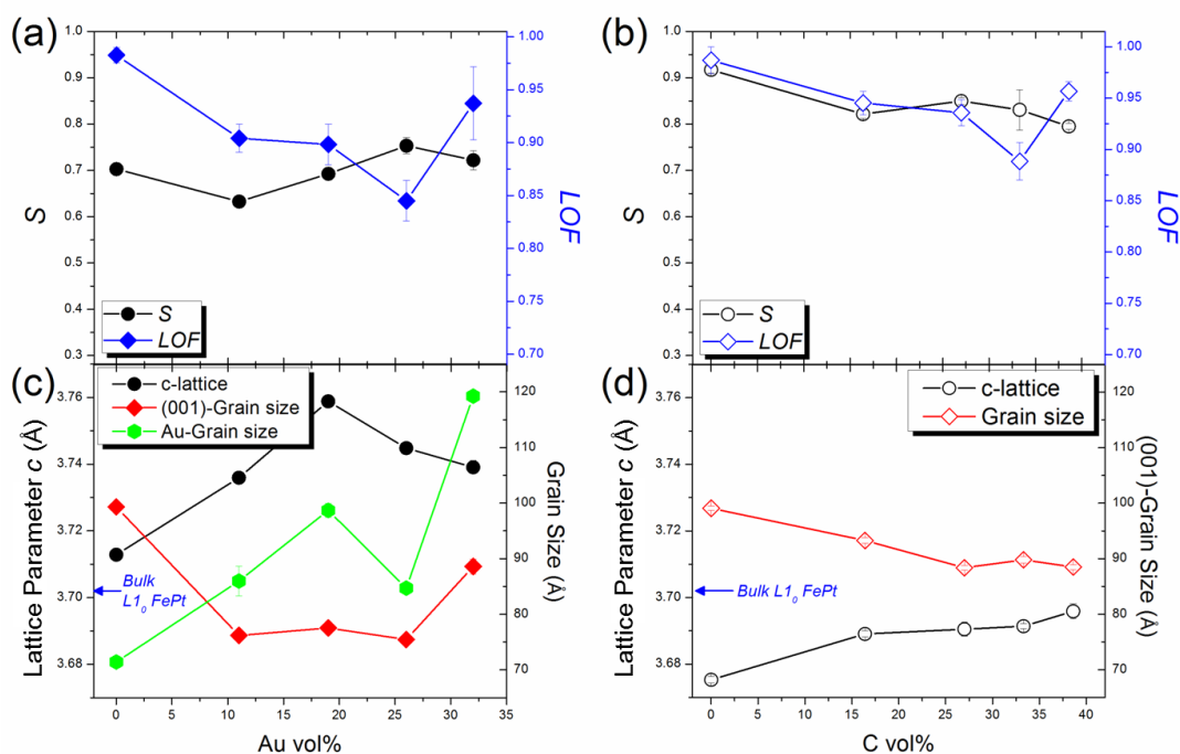
FIG. 5.18. Properties of composite FePt:Au and FePt:C films: S and LOF in (a) and (b) and c -lattice parameter and relevant grain sizes in (c) and (d).
