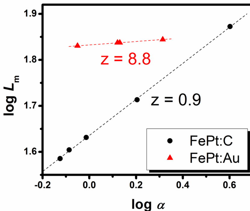
FIG. 5.22. Relationship between correlation length L_m and loop slope \alpha . This double-logarithmic plot is used to determine the parameter z .
