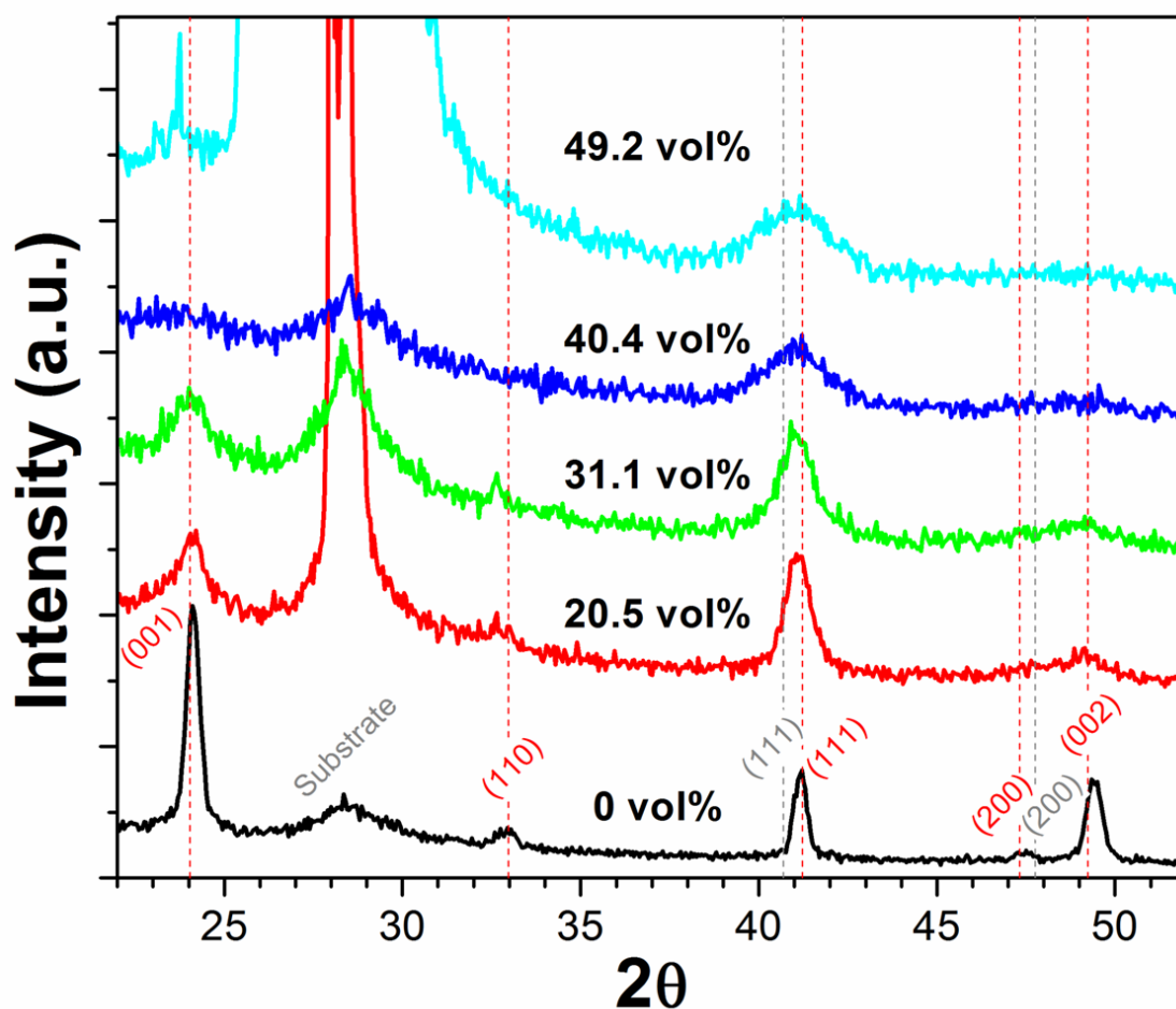
FIG. 5.9. XRD spectra of the AlO5 film series.
