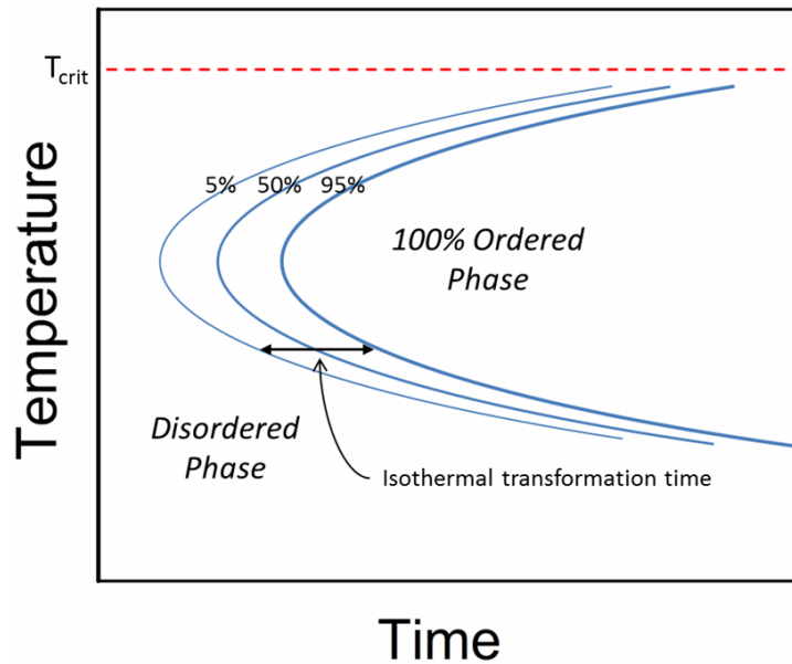
FIG. 2.6. Example TTT diagram. Percentages indicate degree of ordering achievable along those particular curves.
