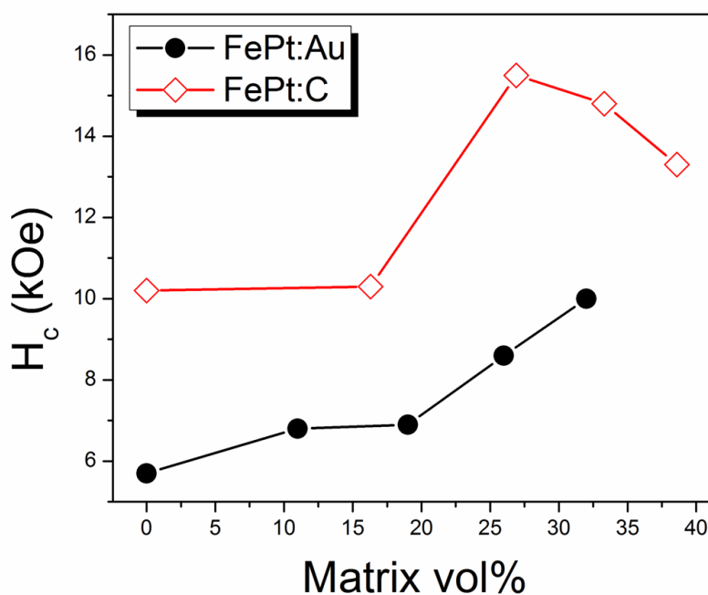
FIG. 5.19. Perpendicular coercivity trends for FePt:Au and FePt:C films with varying matrix concentrations.
