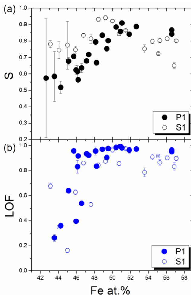
FIG. 4.23. S (a) and LOF (b) estimated for series P1 films versus Fe concentration. Data from series S1 are included for comparison.
