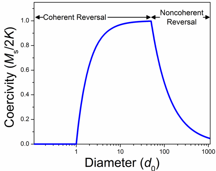
FIG. 2.4. Schematic of coercivity dependence on particle size. Plotted using expressions from Ref. 2.6. Real systems exhibit a less drastic drop in coercivity for increasing particle size across the transition between reversal types.
