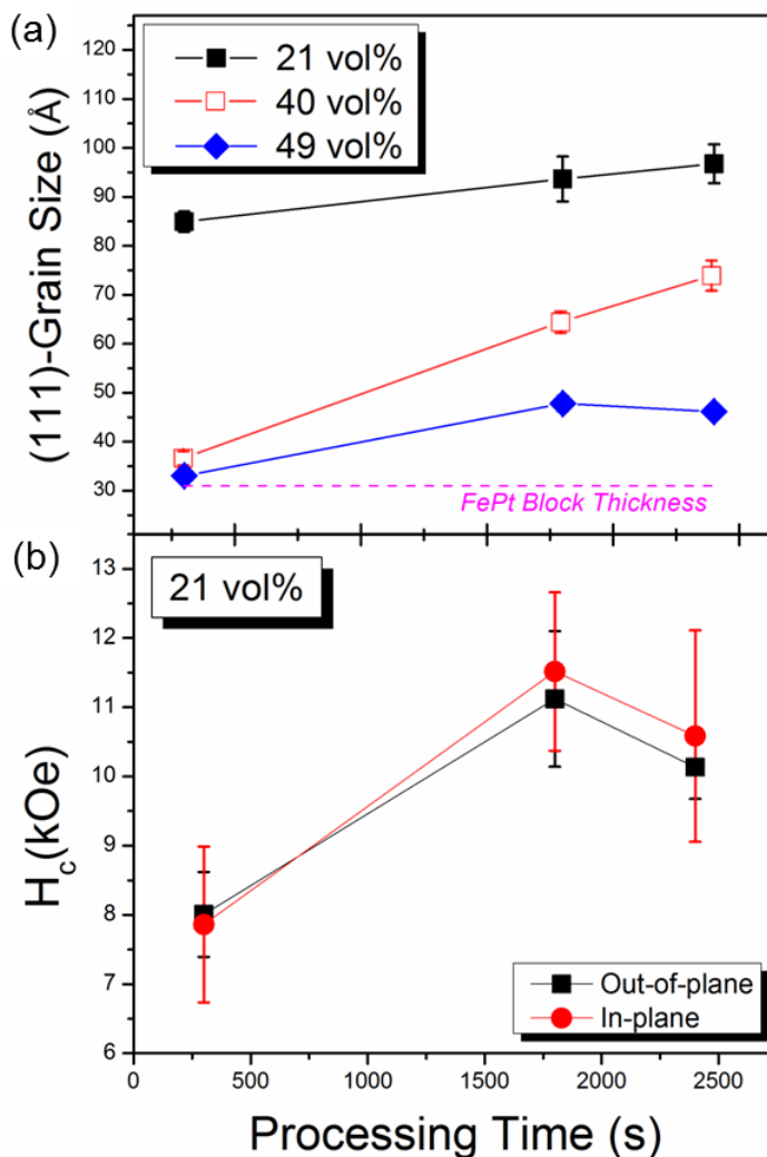
FIG. 5.16. Part (a) shows (111)-grain sizes of select AIO5 samples for longer annealing times. Part (b) shows trend of in- and out-of-plane coercivities of the 21 vol% AIO5 film for increased annealing times.
