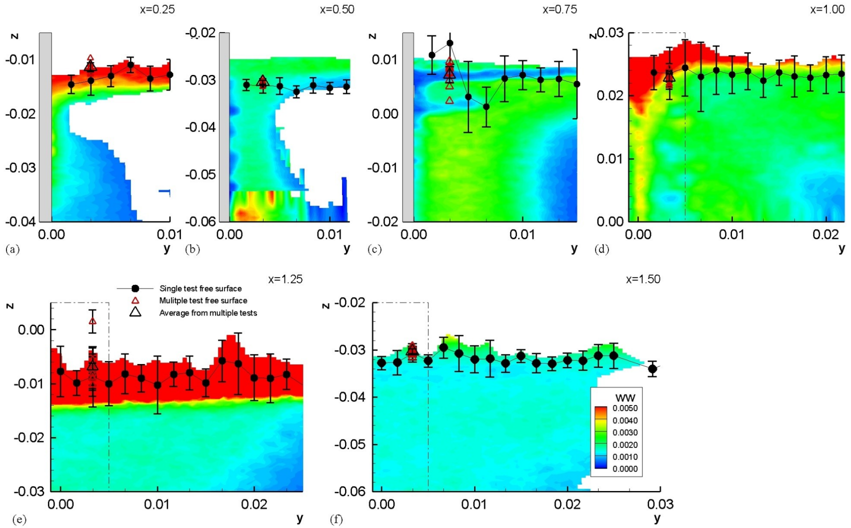
Figure 90: Juncture region w contours, Ak = 0.21
