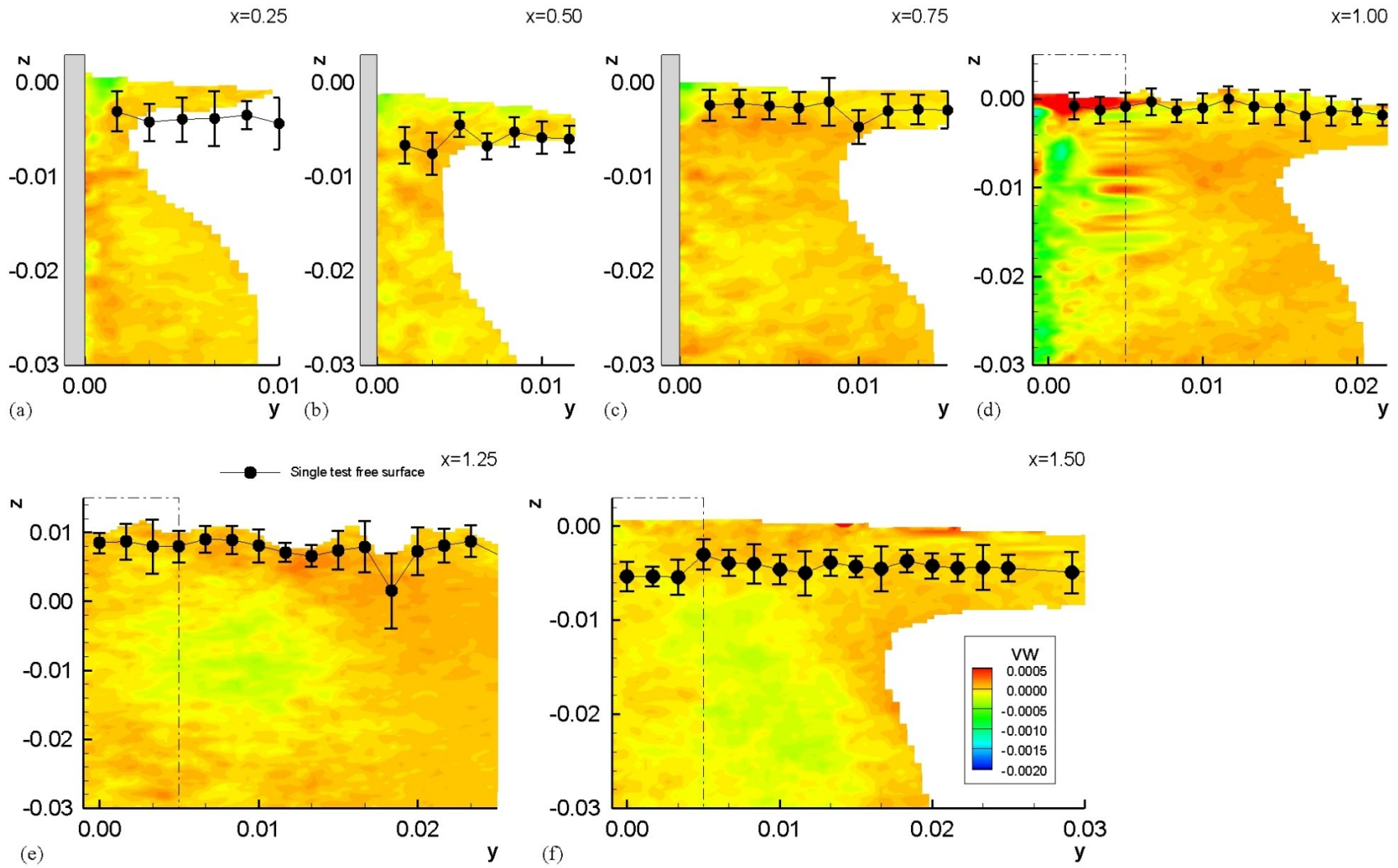
Figure 82: Juncture region vw contours, Ak = 0
