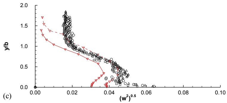
Figure 65: Underlying turbulent flow boundary layer data for x = 1.00 , Ak = 0
