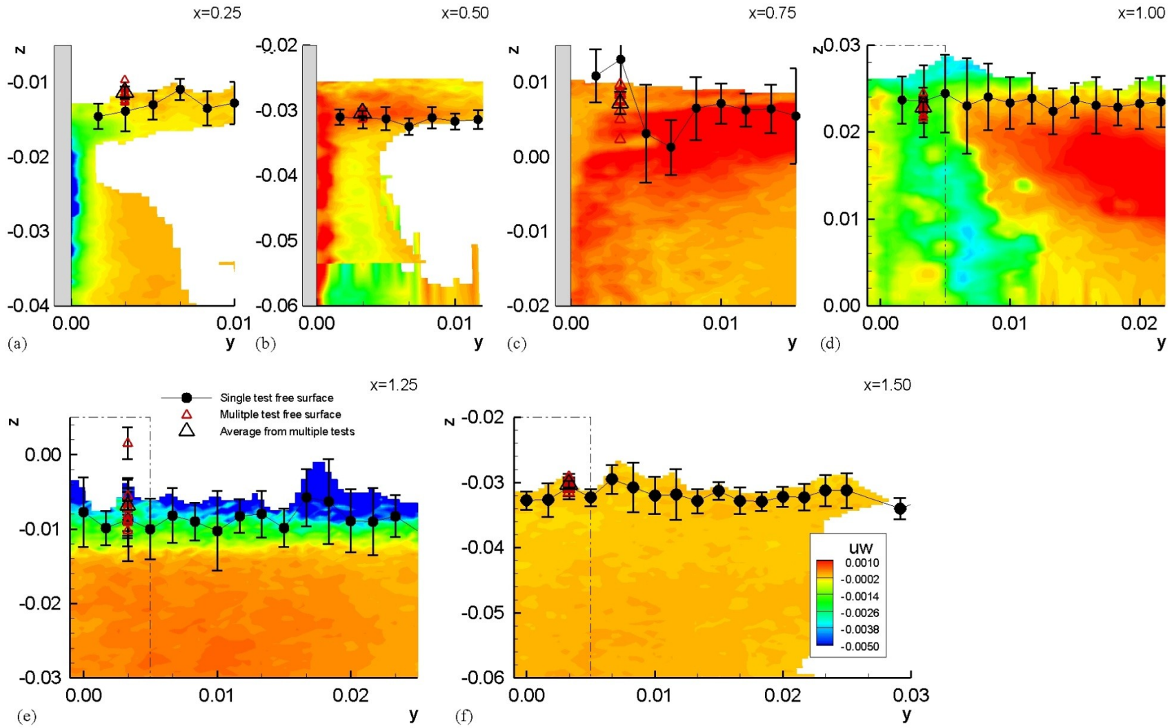
Figure 92: Junction region uw contours, Ak = 0.21
