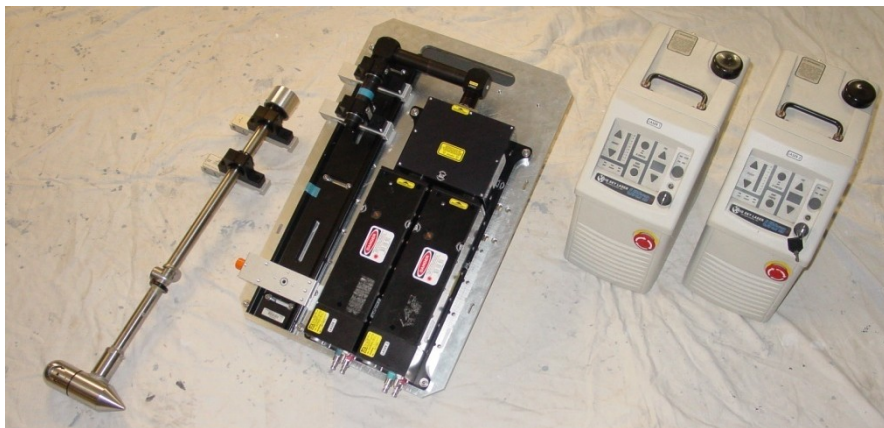
Figure 6: SPIV equipment showing (a) cameras and (b) laser assemblies
