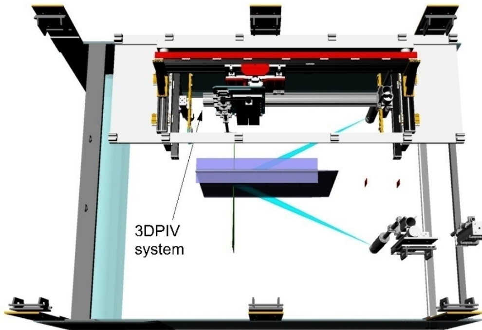
Figure 8: Overhead view of experimental setup for flow field measurements
