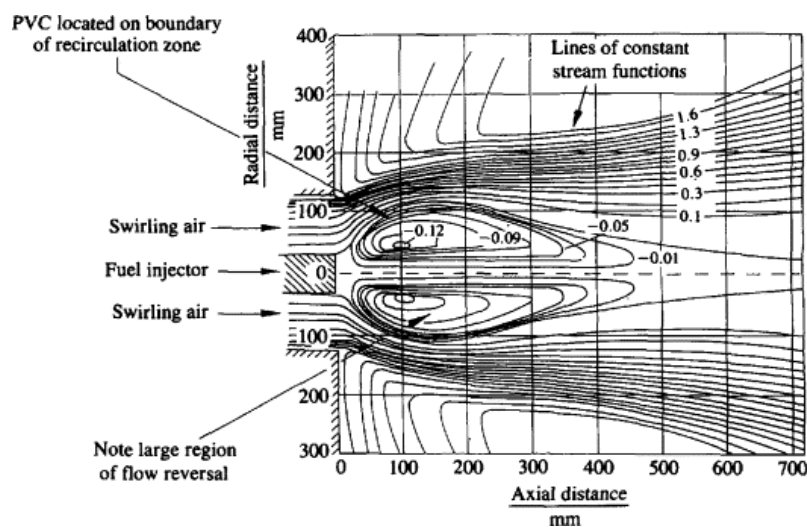
Figure 2.9 Stream line and PVC location of a swirl burner swirl number 1.57
