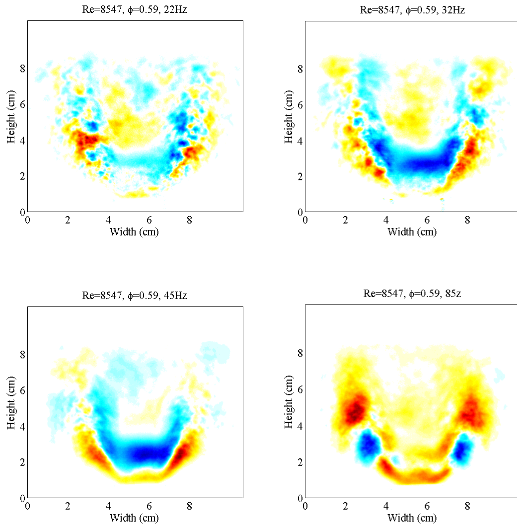
Figure 4. 7 Rayleigh Index Maps for Re=8547 ( f=22,32,45,85Hz )
