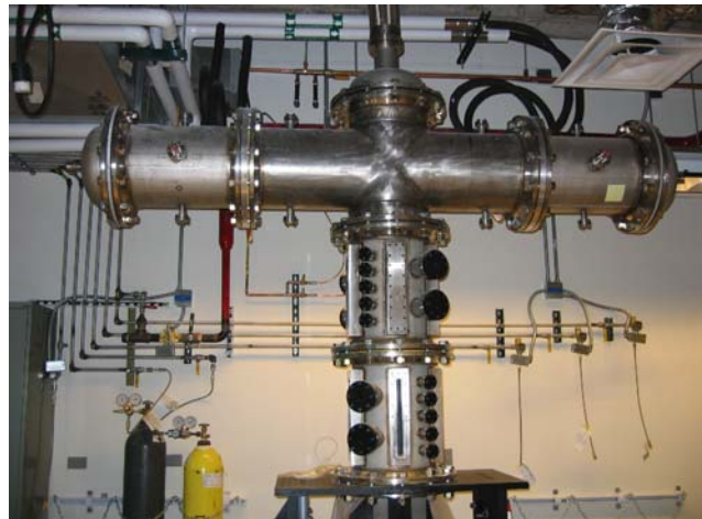
Figure 3.2 Acoustic chamber
