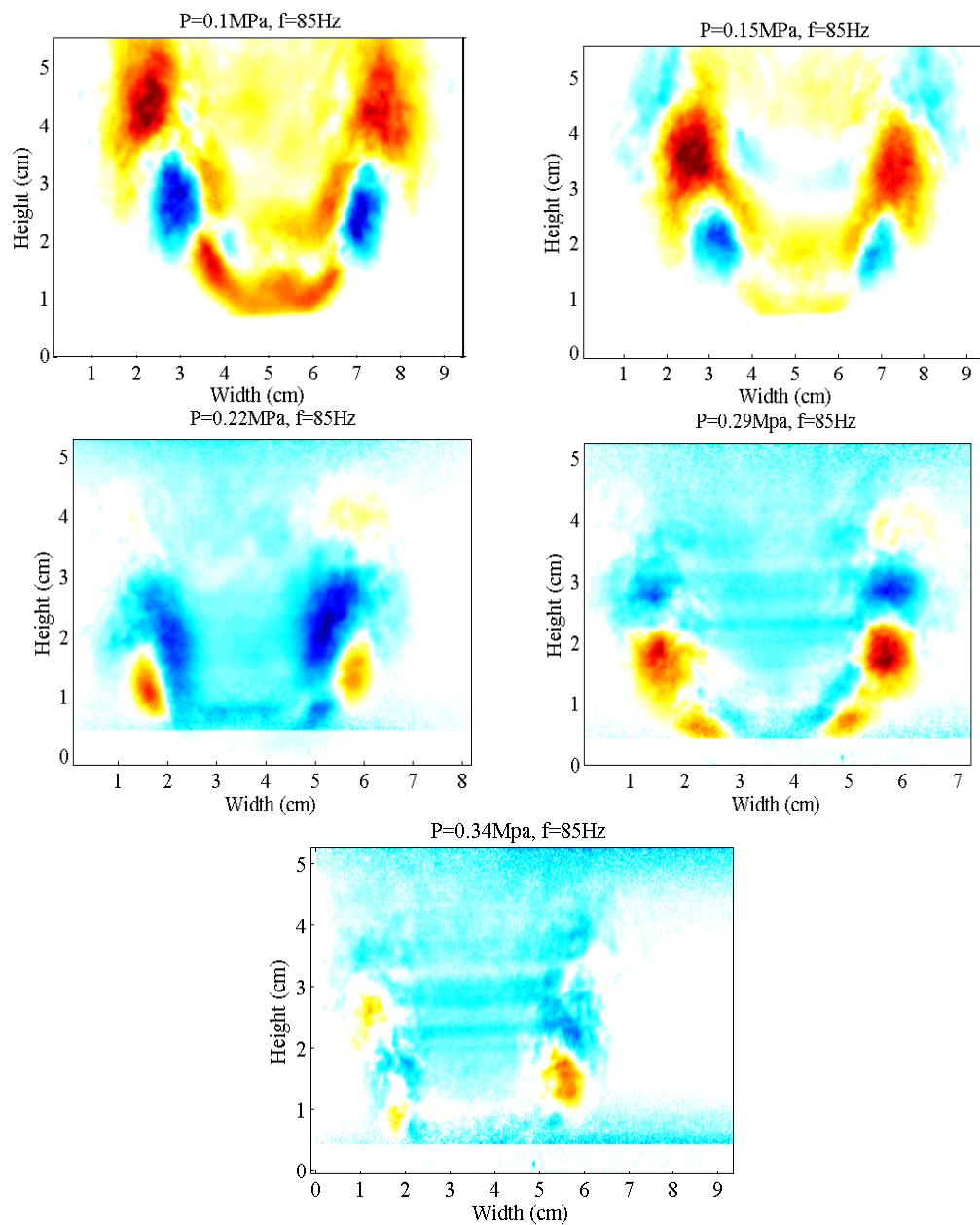
Figure 5.14 Rayleigh Index distribution at 85Hz ( \text{Re}=8547 , \Phi=0.6 )
