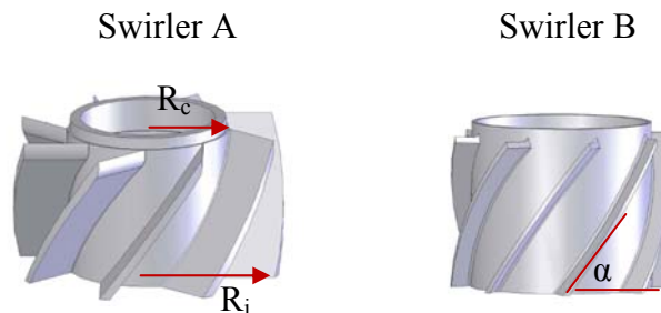
Figure 6.1 Images of the two burners
