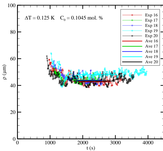
Figure 3.4: Tip radius measurement as a function of time.
