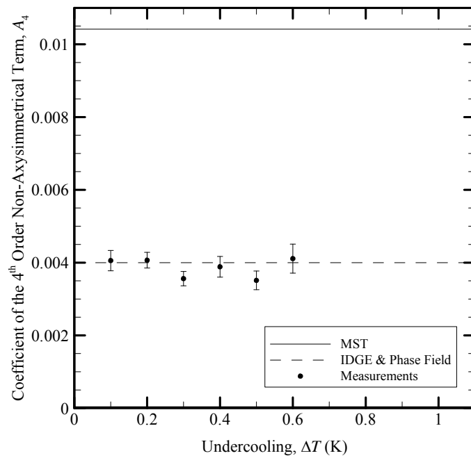
Figure 4.8: Tip radius measurements as a function of the undercooling for almost pure SCN ( C_0 = 0.0086 mol. %).
