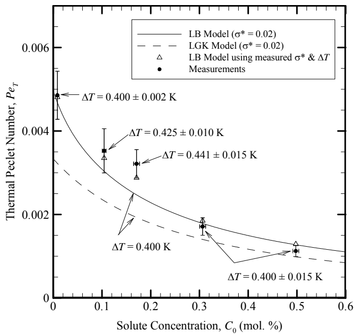
Figure 4.20: Measurements of the thermal Peclet number as a function of the solute concentration for SCN-Acetone alloys.
