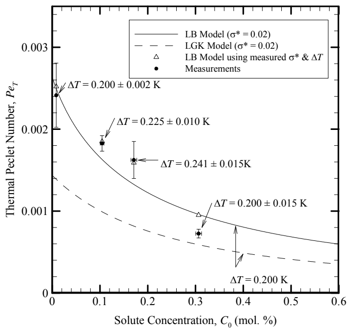
Figure 4.19: Measurements of the thermal Peclet number as a function of the solute concentration for SCN-Acetone alloys.
