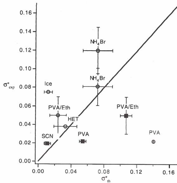
Figure 2.7: Comparison of the MST predictions and experimental benchmarks in terms of the selection parameter [96].
