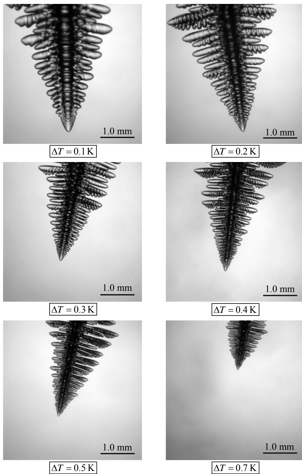
Figure 4.13: Micrographs of SCN-ACE dendrites ( C_0 = 0.1710 \text{ mol. \%} ).
