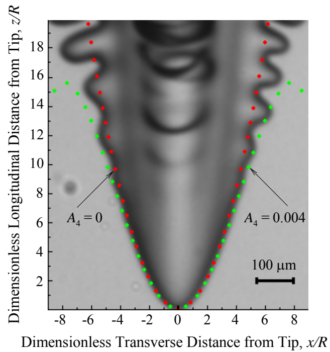
Figure 4.6: Verification of the MST for almost pure SCN ( C_0 = 0.0086 mol.% & \Delta T = 0.300 K)
