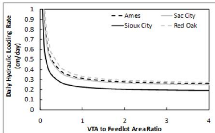
Figure 3. Predicted average daily hydraulic loading rate versus the vegetative treatment area to feedlot ratio. Feedlot runoff calculated using a curve number of 91 for the feedlot.
