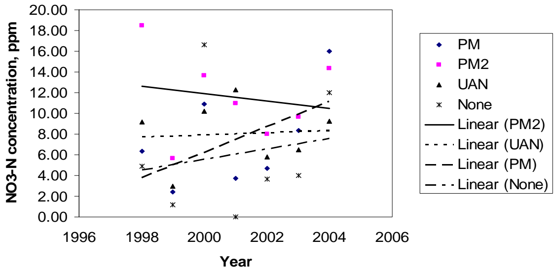
Figure 7b. Temporal variability \text{NO}_3\text{-N} concentration in the top soil layer (15-30 cm) as a function of fertilizer types for Fall soil test (1998-2004)
