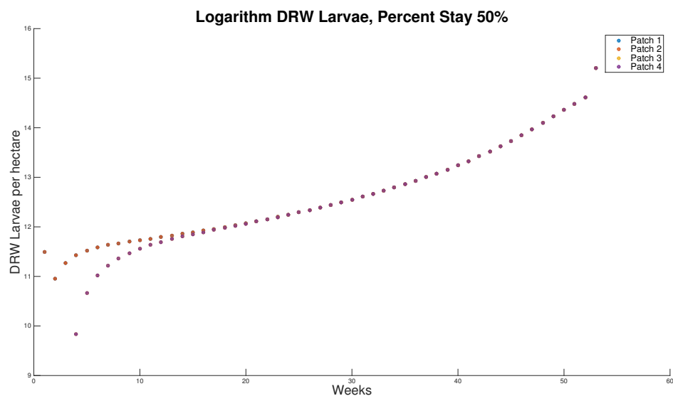
Figure 7.32: Logarithm of number of DRW larvae to apply when \delta = .999 and initial populations 200000 for p = .5 , associated with figure 7.31
