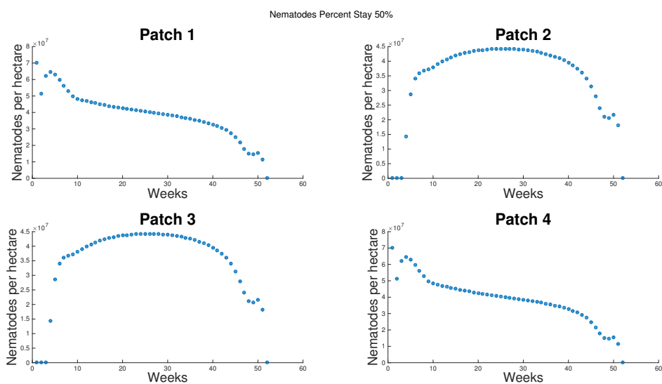
Figure 7.18: Using the Forward-Backward Sweep we calculate the number of nematodes to apply when \delta = .99 and initial populations 200000 for p = .5 .
