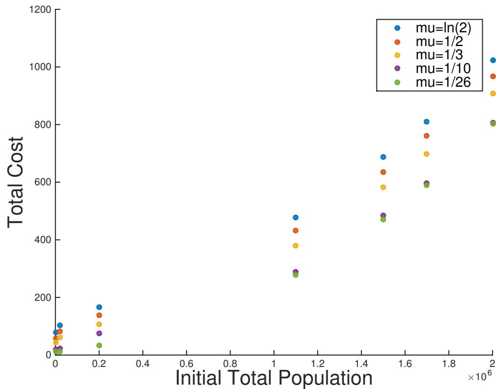
Figure 4.23: The Total Cost, or value of J , which corresponds to all the initial populations, \mu values and nematodes applications from Figure 4.22.
