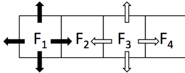
Figure 7.1: Four Connected Patches: Note any patch is connected to the patches next to it. Specifically consider patch F_1 which is connected to patch F_2 . Note the black arrows from F_1 demonstrate how the adult pest can disperse from the patch, specifically the pest adult can only spread to F_2 and to none of the other patches. Meanwhile, F_3 is attached to F_2 and F_4 and the pest adults in F_3 can spread to F_2 and F_4 along the white arrows but not to F_1 . Note that F_2 spreads to F_1 and F_3 , while F_4 only spreads to F_3 , these patches arrows are not show in the figure.
