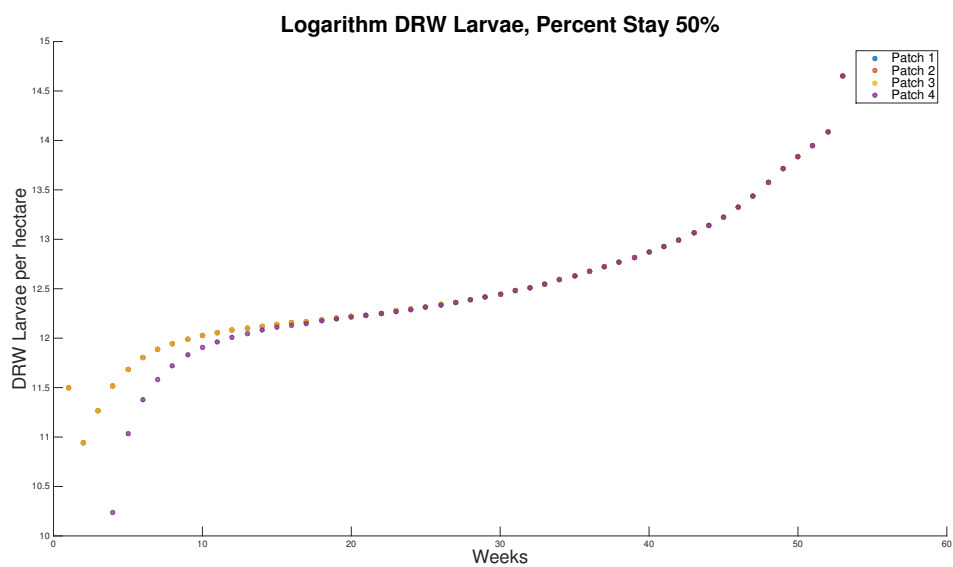
Figure 7.34: Logarithm of number of DRW larvae to apply when \delta = .999 and initial populations 200000 for p = .5 , associated with figure 7.33
