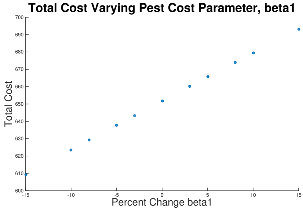
Figure 4.8: For initial population 1100000 we vary the value of \beta_1 by the percents -15, -10, -8, -5, -3, 0, 3, 5, 8, 10, 15. In the figure we display the Total Cost.
