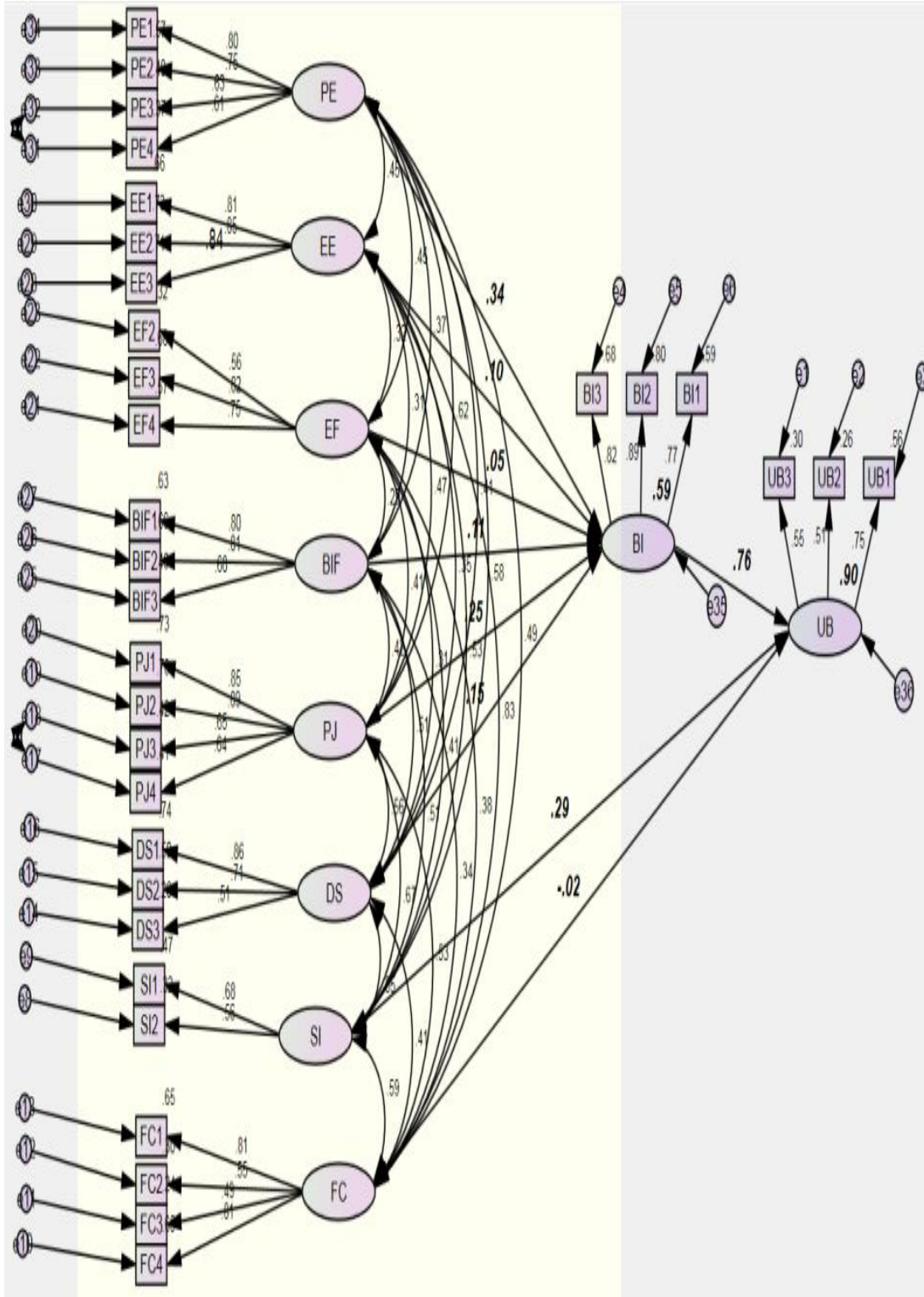
Figure 15: Structural model
