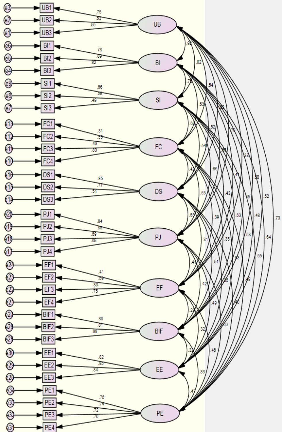
Figure 14: Measurement Model
