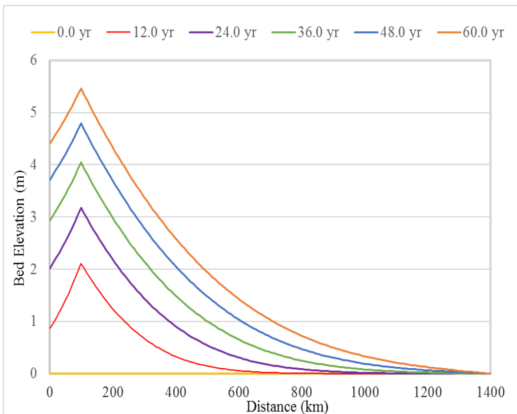
Figure 4.5 Change in Bed Elevation with Pre-Dam Conditions with Channel Narrowing
