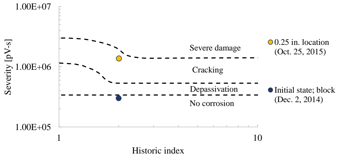
Figure 5.24 Intensity Analysis for broadband sensors on reactor concrete block specimen.
