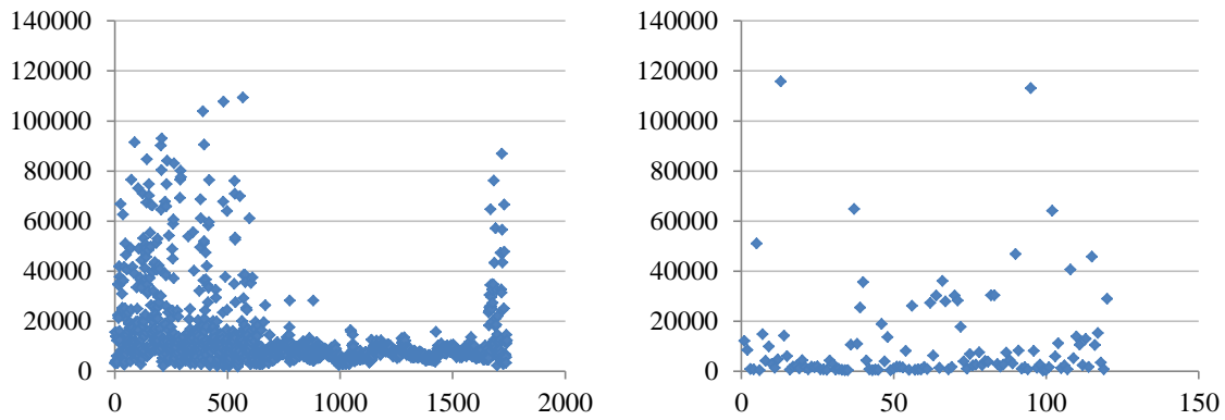
Figure A.9 Values of wavelet based criterion C4 for leakage dataset (left) and corrosion dataset (right).
