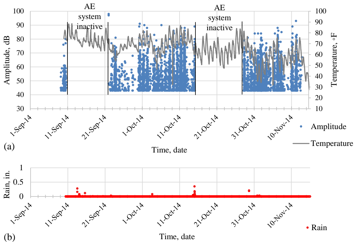
Figure 5.12 (a) Amplitude and temperature versus time for four wireless sensors at +48 level, and (b) rain versus time.
