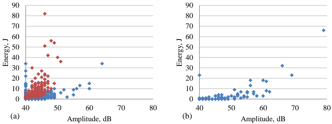
Figure A.6 Energy versus amplitude (hits with rise time higher than 370 \mu -seconds plotted in red): (a) due to leakage, and (b) due to corrosion.
