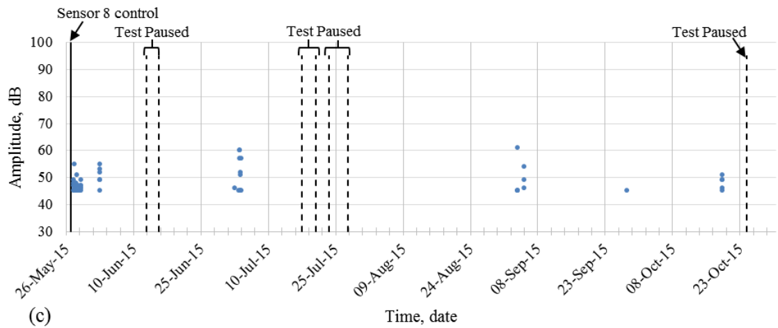
Figure 5.19 AE data recorded from resonant sensors on the reactor concrete block specimen: (a) 1.0 inch concrete cover location, (b) 0.125 inch concrete cover location, and (c) control location.
