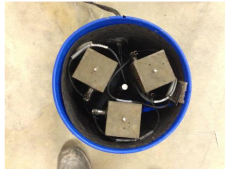
Figure 4.3 Test setup. Controlled temperature chamber (left) and specimens placed in 100% relative humidity buckets (right).
