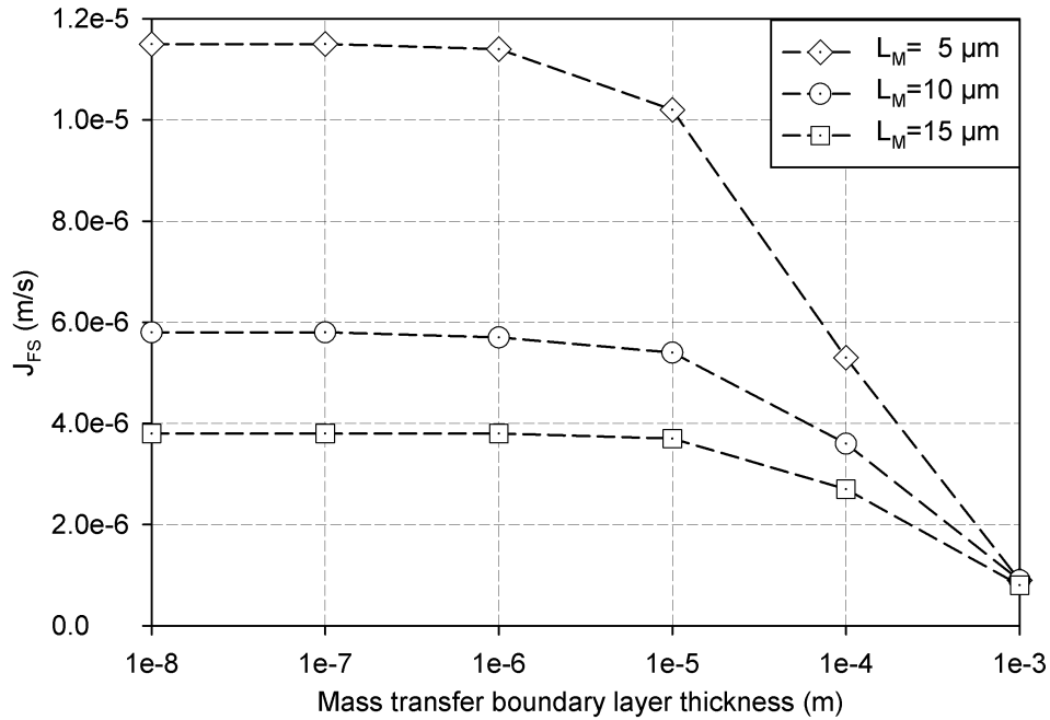
Fig. 4.12 Full-scale water flux as a function of mass transfer boundary layer and membrane thickness.
