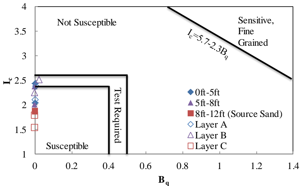
Figure 5.5 CPT-based liquefaction susceptibility chart after Hayati and Andrus (2008a) with data from Fort Dorchester site oriented in E-W direction.
