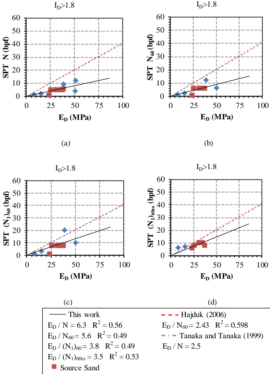
Figure 4.16 SPT-DMT Correlations for Sands at Hollywood Site: a) N vs E_D , b) N_{60} vs E_D , c) (N_1)_{60} vs E_D and d) (N_1)_{60cs} vs E_D
