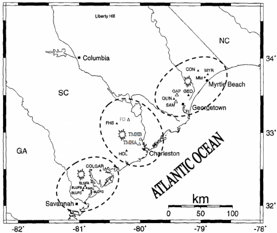
Figure 1.1 Locations of Paleoliquefaction Features in the South Carolina Coastal Plain (after Hu et al. 2002a, as shown in Williamson, 2013)
