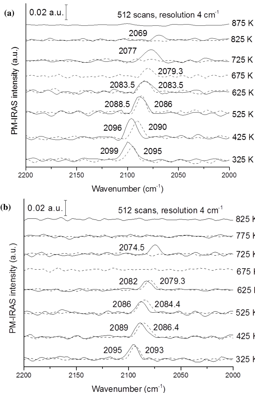
Figure 3.5: IR spectra of CO on Pt(100) at 100 Torr, (a) during first heating (solid line) and cooling (dash line) process (b) during repeated heating-cooling process after (a)
