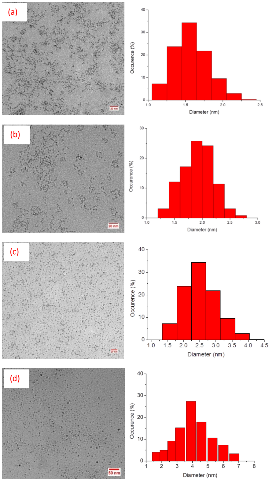
Figure 4.15: TEM images and size distribution of Ru nanoparticles as synthesized with reduction temperature of 180 °C
