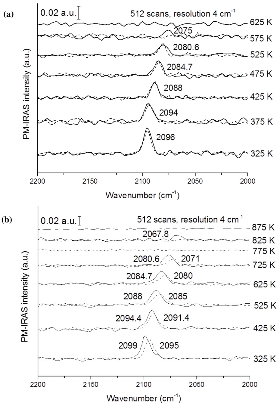
Figure 3.4: IR spectra of CO on Pt(100) during heating (solid line) and cooling (dash line) process at (a) 10^{-4} Torr CO, (b) 2 Torr CO
