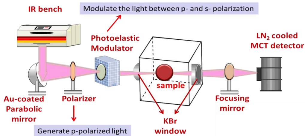
Figure 2.8: Optical view of PM-IRAS system
