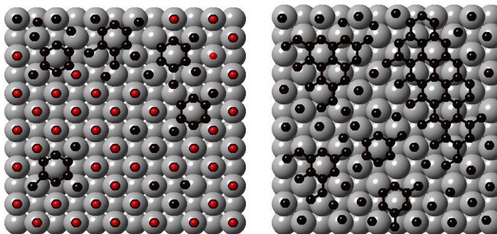
(c) Carbon islands formation
