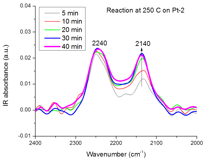
Figure 5.9: The IR spectra of isocyanate and cyanide species during the reaction on Pt-2 at 250 °C until steady state
