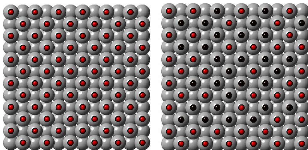
(a) CO-covered Pt(100) surface
