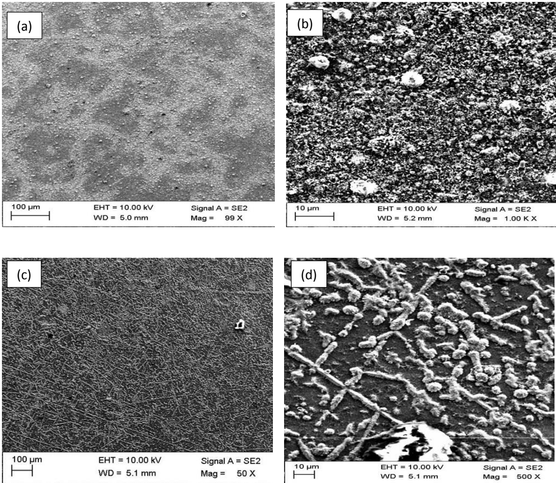
Figure 4.8: SEM images of \alpha\text{-Al}_2\text{O}_3/\text{Inconel} sample before (a)(b) and after (c)(d) ammonia adsorption test in vacuum chamber
