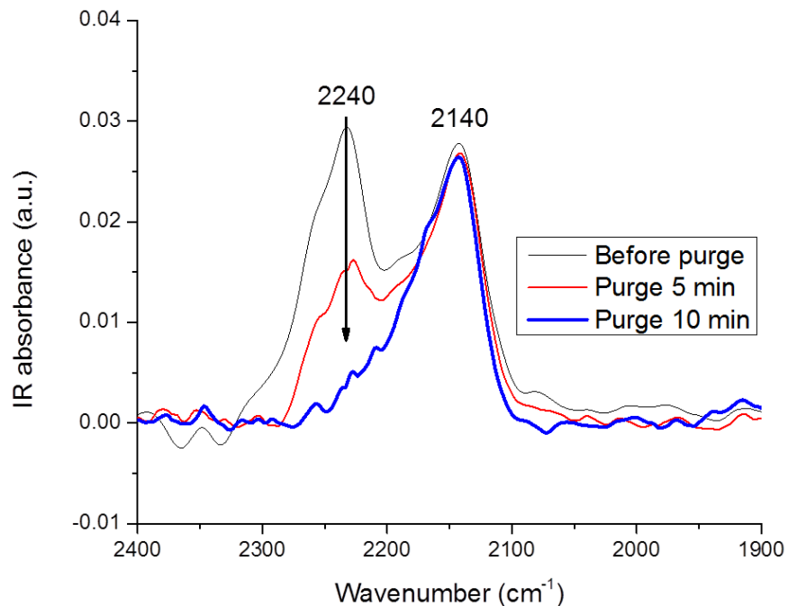
Figure 5.8: The IR spectra of isocyanate (2240 cm -1 ) and cyanide (2140 cm -1 ) species during the purge of 3% O 2 /He after steady state reaction on Pt-2 at 250 °C
