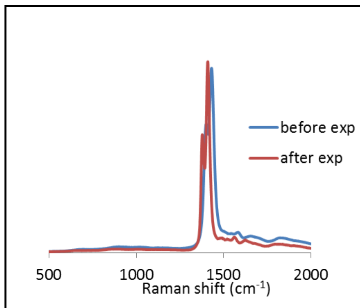
Figure 4.7: Raman spectra of \alpha\text{-Al}_2\text{O}_3/\text{Inconel} sample before and after ammonia adsorption test in vacuum chamber (clear fluorescence signal of \alpha\text{-Al}_2\text{O}_3 on both sample)
