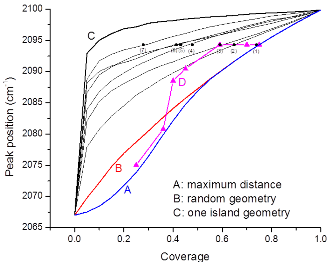
Figure 3.13: Peak position vs. coverage for CO adsorption on clean sample and annealed samples, as well as simulated CO adsorption with different adsorbate geometries. Curve D with triangular data points correspond to different exposure of CO on clean sample from 1 L ( 2075 \text{ cm}^{-1} ) to 1000 L ( 2094 \text{ cm}^{-1} ). Thermal desorption data points (filled circles) correspond to 100 L CO exposure on different samples (1), (3), (4) sample after 775 K annealing for 10 min, 30 min and 1h, respectively; (2), (5) sample after 825 K annealing for 10 min and 30 min; (6), (7) sample after 875 K annealing for 10 min and 30 min. All annealing was operated under 100 Torr CO condition to produce possible carbon deposition on the surface
