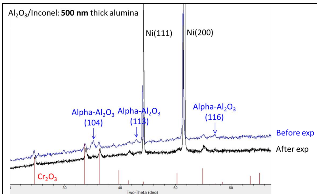
Figure 4.6: XRD pattern of \text{Al}_2\text{O}_3/\text{Inconel} sample before and after the ammonia adsorption experiment in the vacuum chamber (alumina signal attenuated)
