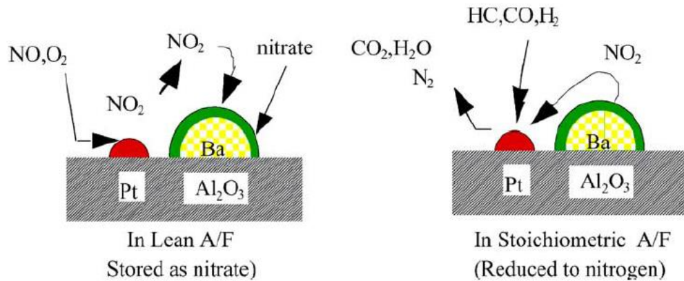
Figure 5.2: Representative schematic of NO x storage-reduction on NSR catalyst [213]
