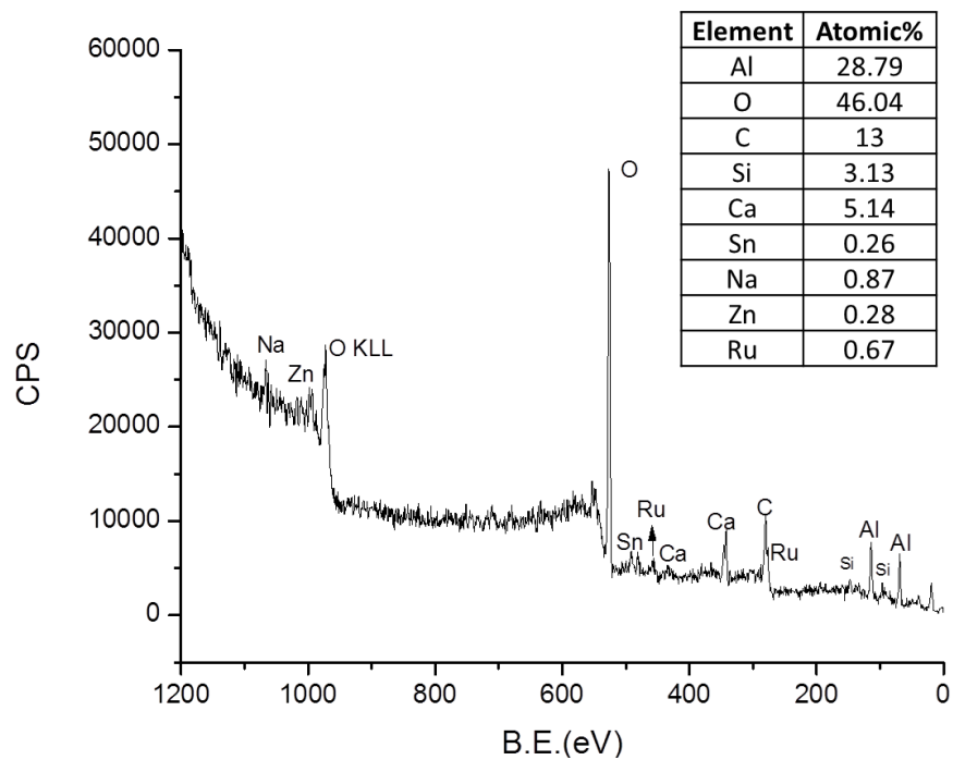
Figure 4.21: XPS spectra of model supported catalyst Ru/Al 2 O 3
