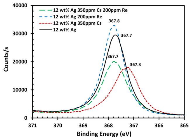
Figure 4.8 Ag 3d_{5/2} spectra for (1), 12 wt% Ag/ \alpha - Al_2O_3 , (2), 12 wt% Ag, 350 ppm Cs/ \alpha - Al_2O_3 , (3), 12 wt% Ag, 200 ppm Re/ \alpha - Al_2O_3 , and (4), 12 wt% Ag, 350 ppm Cs, 200 ppm Re/ \alpha - Al_2O_3 after in situ pretreatment in 10% O_2 /balance He at 280 °C for 12 h. Only Ag 3d_{5/2} binding energy shown for purposes of clarity.
