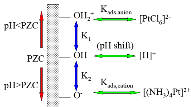
Figure 1.3 Electrostatic adsorption mechanism [24].
