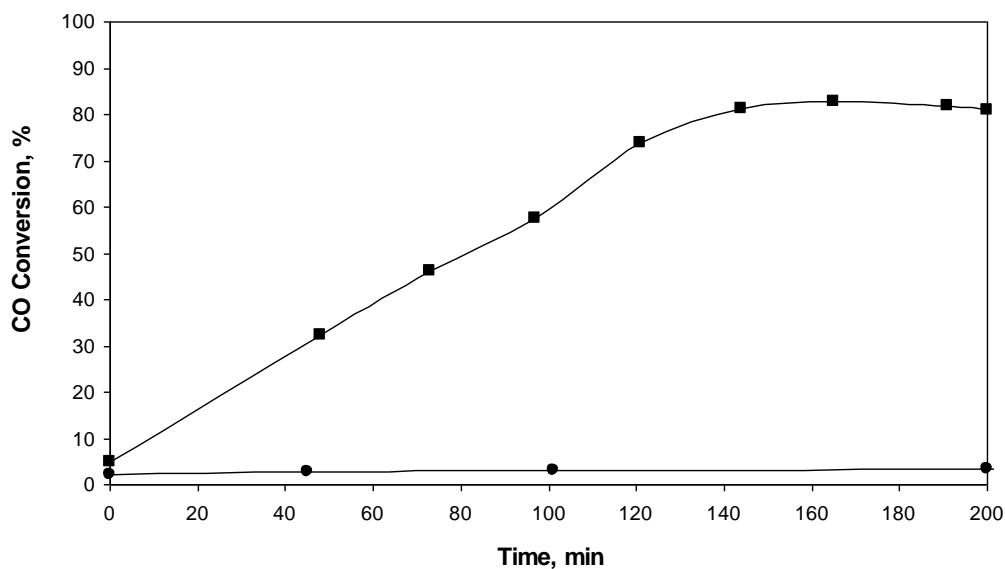
Figure 5.6 CO conversion with time for Rh(CO) 2 /HY30 (●) and Rh(CO) 2 /HY2.6 (■) samples during NO/CO reaction at 1000 ppm NO, 1000 ppm CO, 270 °C.
