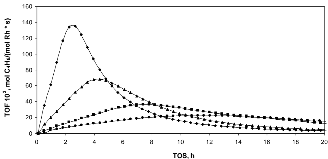
Figure 4.11 Rates (Turn Over Frequencies) of Trans-2-Butene formation with Time on Stream (TOS) for \text{Rh}(\text{CO})_2/\text{HY30} at 608 Torr of \text{H}_2 and different partial pressures of \text{C}_2\text{H}_4 : 38 Torr (●) 76 Torr (■) 114 Torr (▲) 152 Torr (◆).
