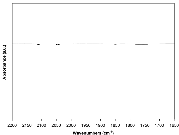
Figure 5.8 FTIR difference spectra in the \nu_{\text{CO}} and \nu_{\text{NO}} regions of Rh(CO) 2 /HY30 sample collected during the reaction 200 min in 1000 ppm NO, 1000 ppm CO at 270 °C.
