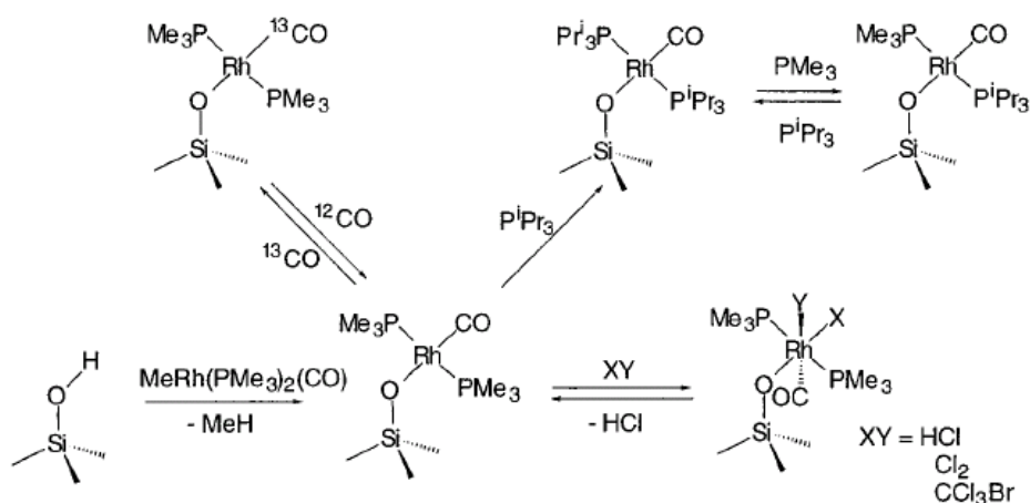
Figure 1.8 Surface chemistry of silica-supported \text{Rh}(\text{P}(\text{CH}_3)_3)_2(\text{CO}) complexes [22].
