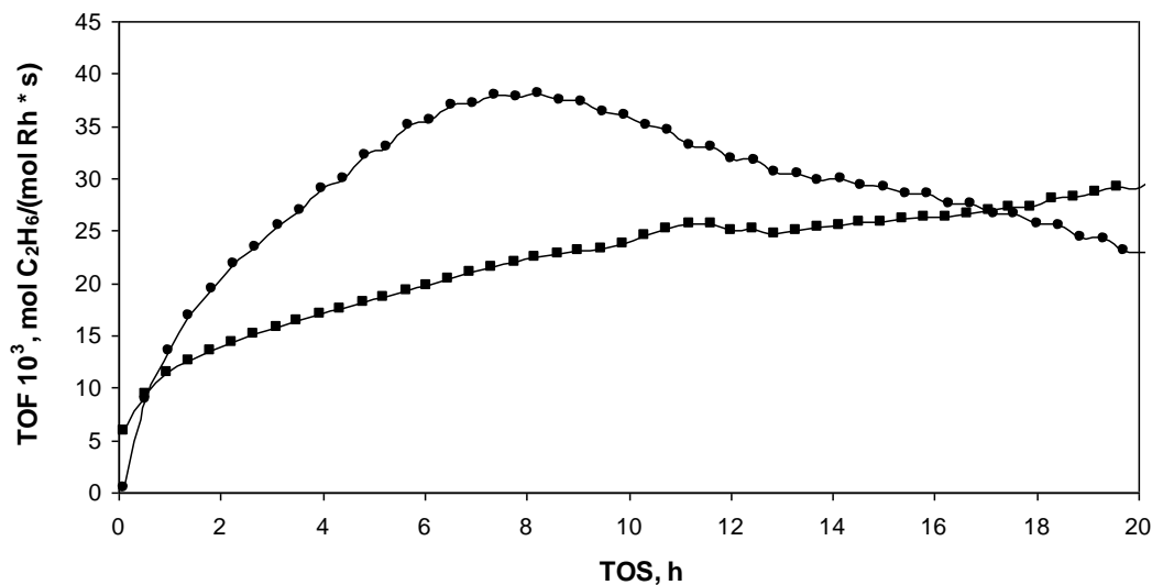
Figure 4.32 Rates (Turn Over Frequencies) of Ethane formation with Time on Stream (TOS) for Rh(CO) 2 /HY30 (●) and Rh(CO) 2 -Au(CN) 2 /HY30 (Rh/Au = 1/1 mol) (■) at 608 Torr of H 2 and 76 Torr of C 2 H 4 .
