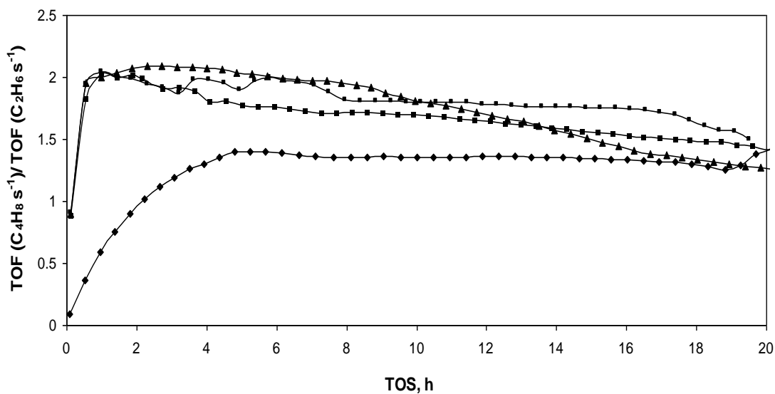
Figure 4.8 Ratio of Ethane and Butenes formation rates with Time on Stream (TOS) for \text{Rh}(\text{CO})_2/\text{HY30} at 76 Torr of \text{C}_2\text{H}_4 and different partial pressures of \text{H}_2 : 76 Torr (●) 228 Torr (■) 380 Torr (▲) 608 Torr (◆).
