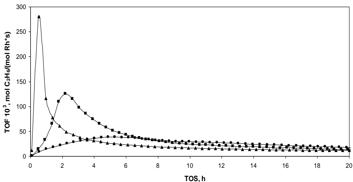
Figure 4.16 Rates (Turn Over Frequencies) of Ethane formation with Time on Stream (TOS) for Rh(CO) 2 /HY30 (●), Rh(CO) 2 /HY15 (■), Rh(CO) 2 /HY2.6 (▲) at 608 Torr of H 2 and 76 Torr of C 2 H 4 .
