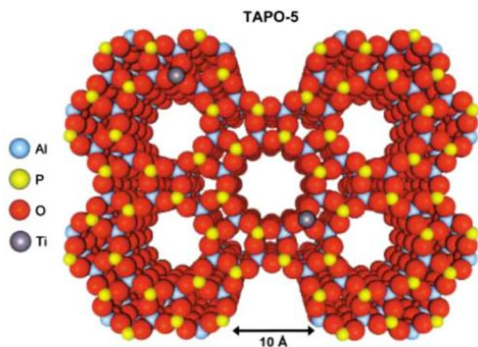
Figure 1.15 The structure of the AIPO-5 catalyst with framework-incorporated Ti^{4+} ions [109,110]
