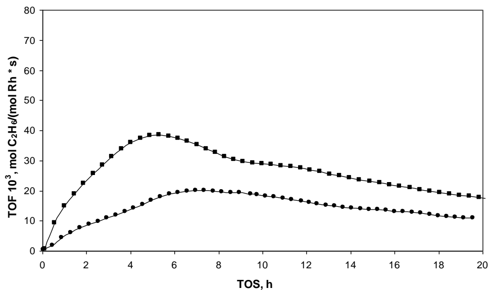
Figure 4.27 Rates (Turn Over Frequencies) of Ethane formation with Time on Stream (TOS) for \text{Rh}(\text{CO})_2/\text{HY30} with 1 % wt Rh (●), 2 % wt Rh (■) at 608 Torr of \text{H}_2 and 76 Torr of \text{C}_2\text{H}_4 .
