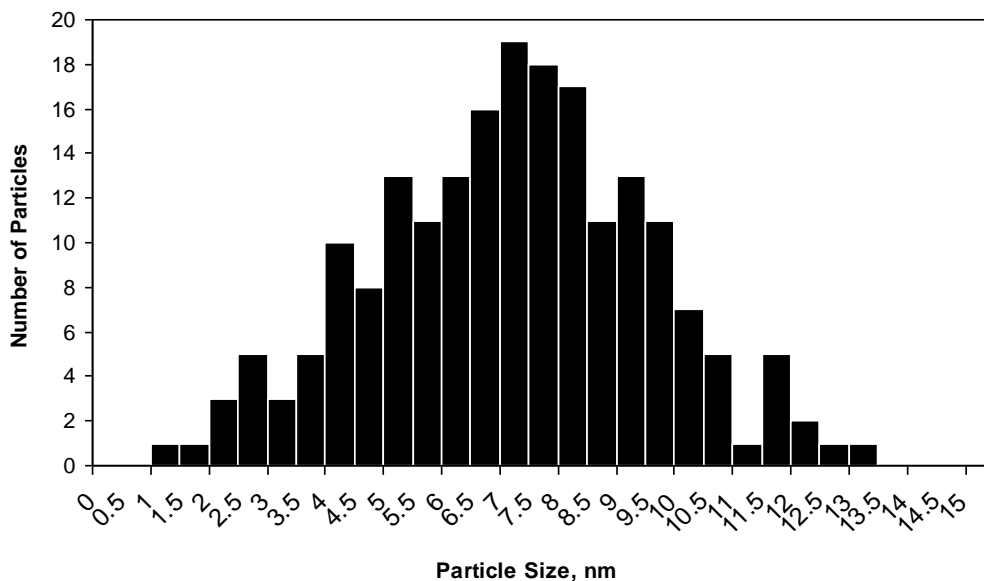
Figure 5.11 Particle size distribution histogram (175 particles counted) obtained from HRTEM measurements of used Rh(CO) 2 /HY2.6 sample (after reaction in 1000 ppm NO, 1000 ppm CO at 270 °C for 200 min).
