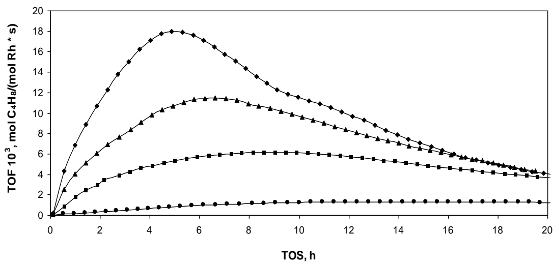
Figure 4.6 Rates (Turn Over Frequencies) of Cis-2-Butene formation with Time on Stream (TOS) for Rh(CO) 2 /HY30 at 76 Torr of C 2 H 4 and different partial pressures of H 2 : 76 Torr (●) 228 Torr (■) 380 Torr (▲) 608 Torr (◆).
