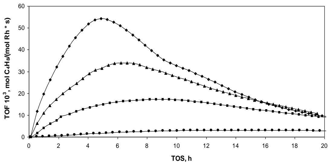
Figure 4.5 Rates (Turn Over Frequencies) of Trans-2-Butene formation with Time on Stream (TOS) for Rh(CO) 2 /HY30 at 76 Torr of C 2 H 4 and different partial pressures of H 2 : 76 Torr (●) 228 Torr (■) 380 Torr (▲) 608 Torr (◆).
