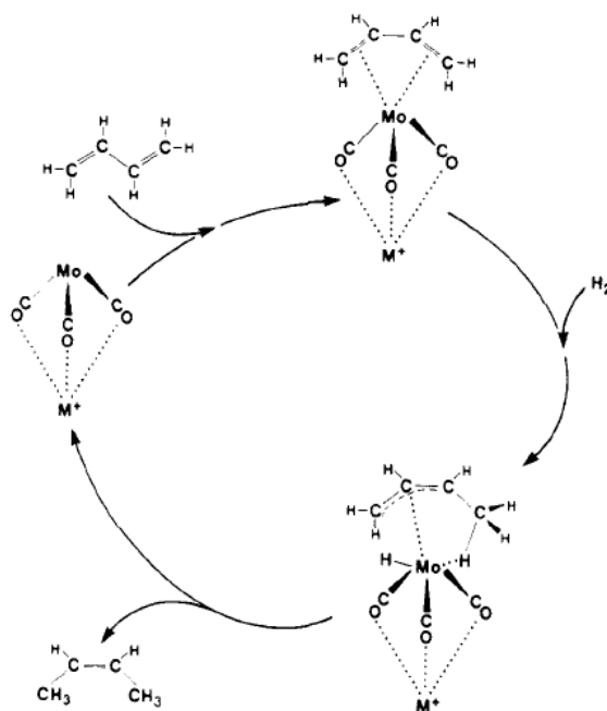
Figure 1.14 Proposed mechanism of 1,3-butadiene to cis-2-butene hydrogenation over Y zeolite-encapsulated \text{Mo}(\text{CO})_3 complexes [92].
