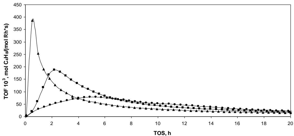
Figure 4.17 Rates (Turn Over Frequencies) of Butenes (Trans-2-butene, Cis-2-butene, Butene-1) formation with Time on Stream (TOS) for \text{Rh}(\text{CO})_2/\text{HY30} ( \bullet ), \text{Rh}(\text{CO})_2/\text{HY15} ( \blacksquare ), \text{Rh}(\text{CO})_2/\text{HY2.6} ( \blacktriangle ) at 608 Torr of \text{H}_2 and 76 Torr of \text{C}_2\text{H}_4 .
