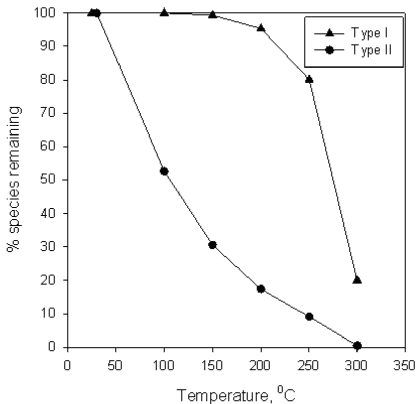
Figure 3.3 Percent of Rh dicarbonyls remaining on the surface of Rh(CO) 2 /HY2.6 during thermal treatments with He at different temperatures: (▲) type I ( \nu_{\text{CO}} at 2117/2053 cm -1 ) and (●) type II ( \nu_{\text{CO}} at 2110/2043 cm -1 ) species.
