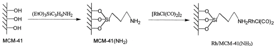
Figure 1.5 Anchoring of \text{RhCl}(\text{CO})_2 complexes on MCM-41 treated with 3-aminopropyltriethoxysilane [15].
