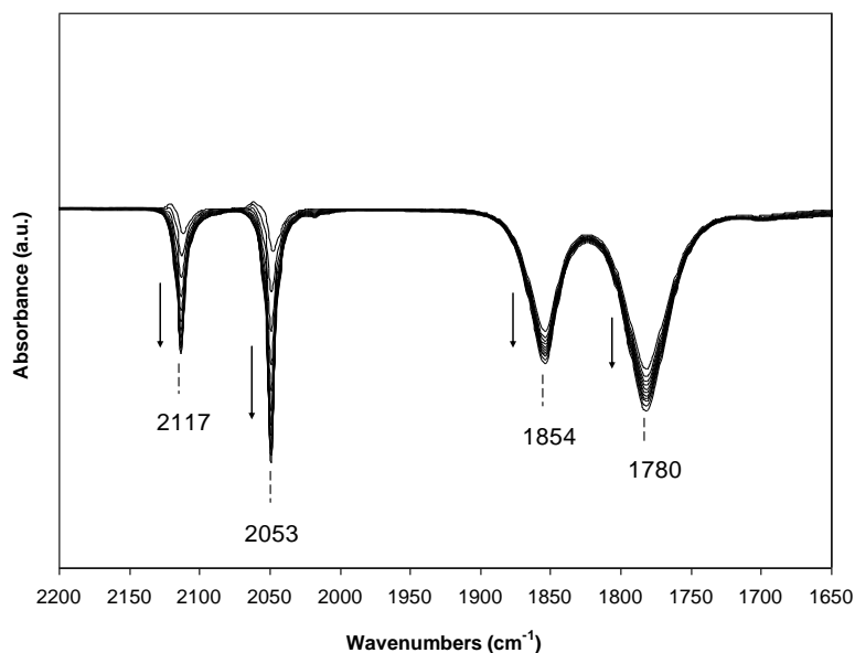
Figure 5.9 FTIR difference spectra in the \nu_{\text{CO}} and \nu_{\text{NO}} regions of Rh(CO) 2 /HY2.6 sample collected during the reaction 200 min in 1000 ppm NO, 1000 ppm CO at 270 °C.
