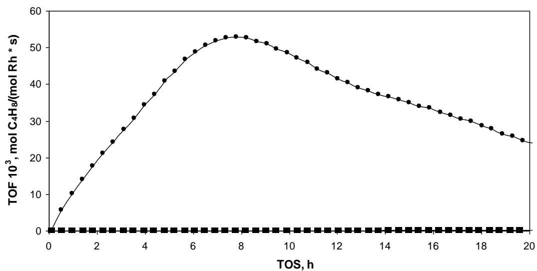
Figure 4.33 Rates (Turn Over Frequencies) of Butenes formation with Time on Stream (TOS) for Rh(CO) 2 /HY30 (●) and Rh(CO) 2 -Au(CN) 2 /HY30 (Rh/Au = 1/1 mol) (■) at 608 Torr of H 2 and 76 Torr of C 2 H 4 .
