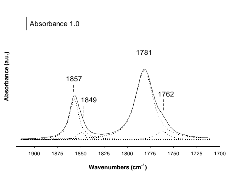
Figure 5.2 FTIR spectrum in the \nu_{\text{NO}} region of \text{Rh}(\text{CO})_2/\text{HY2.6} sample after exposure of 1 % \text{NO}/\text{He} .
