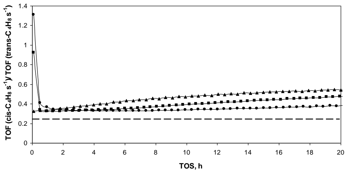
Figure 4.18 Ratio of Cis-2-Butene and Trans-2-Butene formation rates with Time on Stream (TOS) for \text{Rh}(\text{CO})_2/\text{HY30} ( \bullet ), \text{Rh}(\text{CO})_2/\text{HY15} ( \blacksquare ), \text{Rh}(\text{CO})_2/\text{HY2.6} ( \blacktriangle ) at 608 Torr of \text{H}_2 and 76 Torr of \text{C}_2\text{H}_4 .
