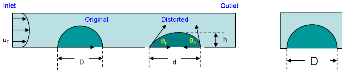
Figure 4.3. Schematic of the drop in the flow channel used in this study.
