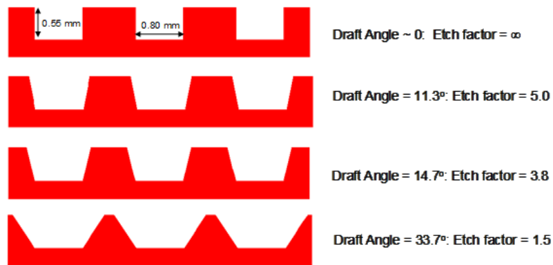
Figure 3.3. Geometries with four different draft angles used in this study. Note that the standard channel shape in this study is ~0 draft angle.
