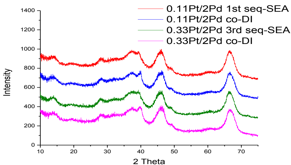
Figure 4.10 XRD patterns of seq-SEA vs co-DI a) Pd@Pt/SiO 2 b) Pt@Pd/A c) Pd@Pt/A
