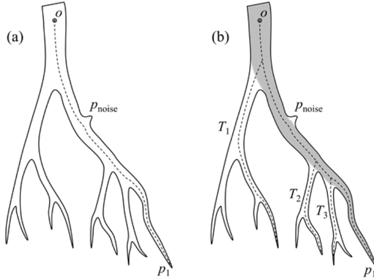
Figure 3 Schematic illustration of the new method. (a) The method starts with the rood point o as the initial skeleton and finds the farthest geodesic point p_1 . This farthest point is connected to the skeleton by a new branch op_1 using a minimum-cost geodesic path. (b) The object volume corresponding to the current skeleton is filled and the next farthest geodesic point p_2 is found and another skeletal branch op_2 is added. It may be noted that the noisy protrusion p_{\text{noise}} does not create any noisy branch even after all meaningful branches are added to the skeleton.
