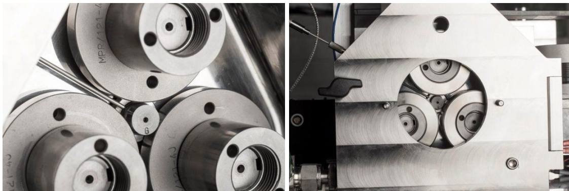
Figure 2. (Left) Positioning of the temperature probe within the MPR (PCS Instruments) test chamber. (Right) Test chamber with the door closed [18].
