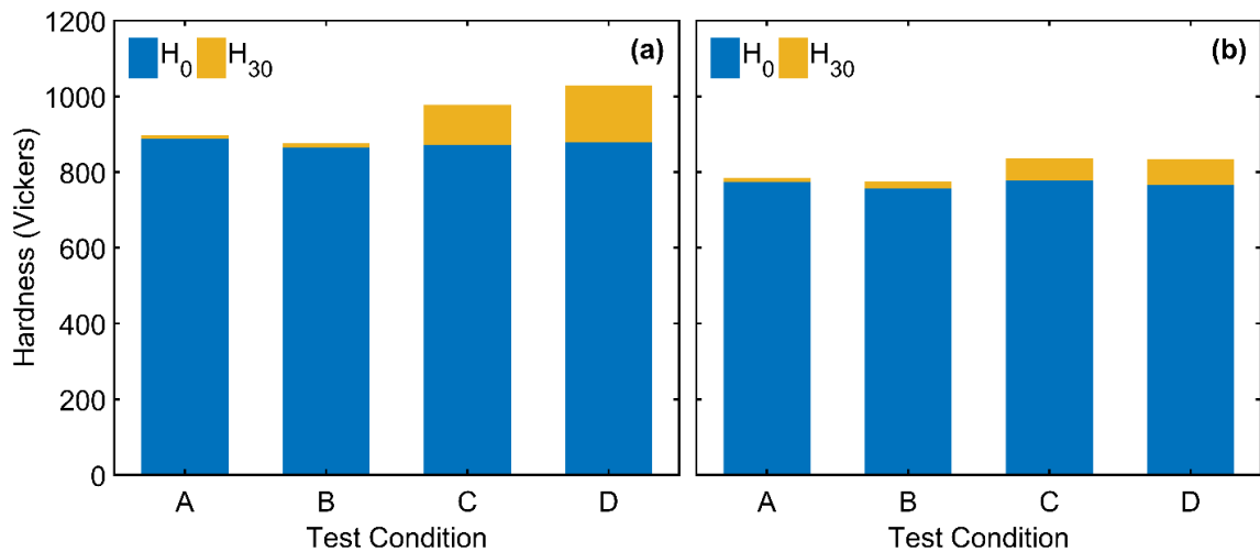
Figure 16. (a) Hardness under conditions A–D measured before testing ( H_0 ) and after running-in for about 22,000 contact cycles or 30 minutes ( H_{30} ) using 50-gf indenter load. (b) Hardness under conditions A–D measured before testing ( H_0 ) and after running-in for about 22,000 contact cycles or 30 minutes ( H_{30} ) using 500-gf indenter load
