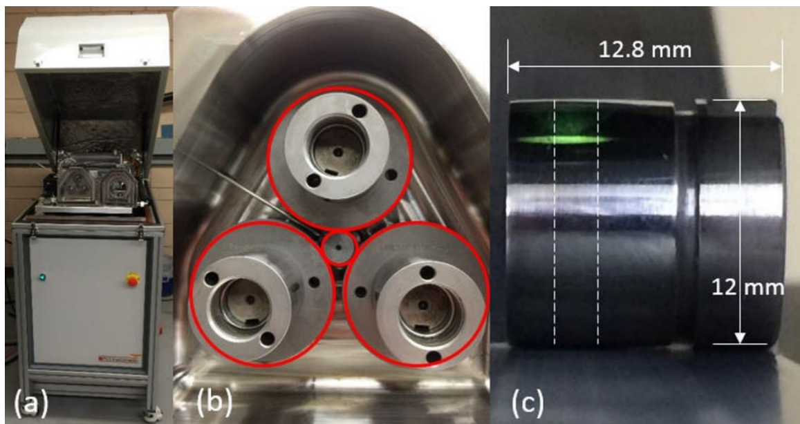
Figure 11. (a) Micro Pitting Rig (MPR) used in this study, (b) test chamber showing the central roller (sample) and three rings, and (c) dimensions of the roller. Dashed lines indicate approximate contact zone.
