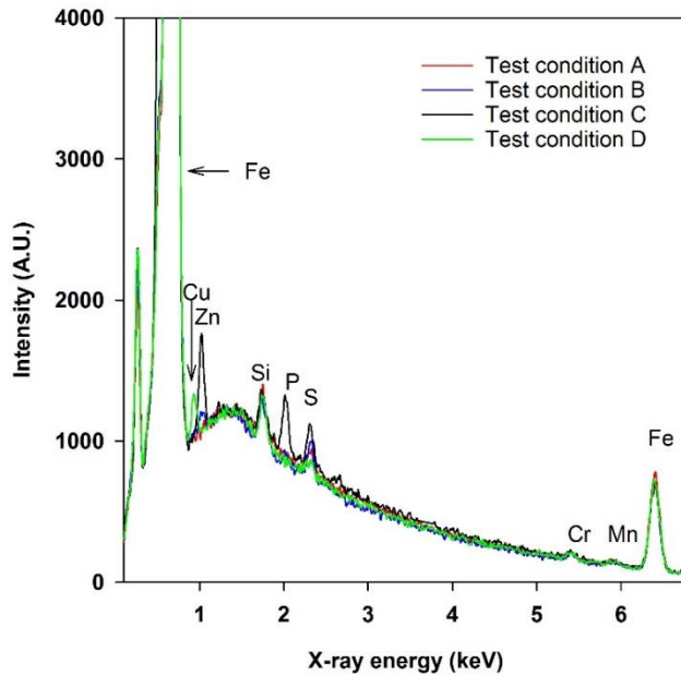
Figure 18. EDS data form inside the wear zone for each of the conditions. Tests used lubricant with ZDDP additive.
