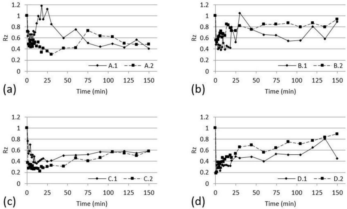
Figure 5. Evolution of normalized Rz for complete test duration for (a) test A replicates, (b) test B replicates, (c) test C replicates, and (d) test D replicates.
