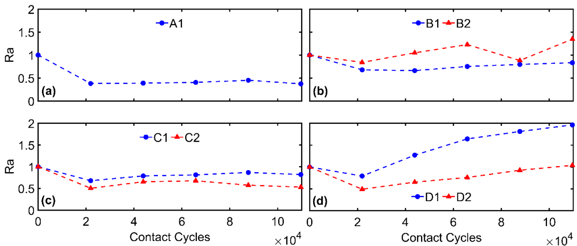
Figure 13. The normalized surface roughness ( R_a ) for conditions A, B, C, and D.
