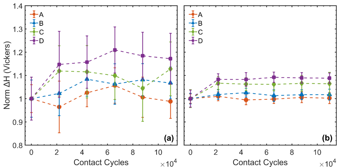
Figure 15. (a) Evolution of hardness under conditions A–D using 50-gf indenter load. (b) Evolution of hardness under conditions A–D using 500-gf indenter load. Error bars represent a 90% confidence interval.
