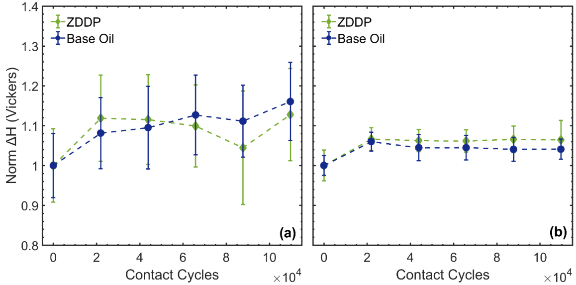
Figure 21. (a) Evolution of hardness under conditions C and E using 50-gf indenter load. (b) Evolution of hardness under conditions C and E using 500-gf indenter load. Error bars represent a 90% confidence interval.
