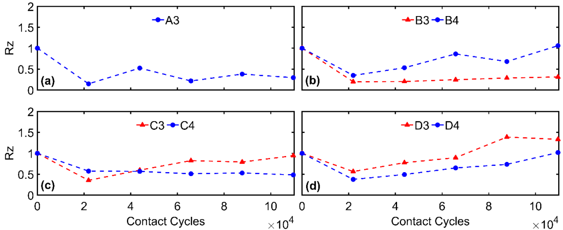
Figure 14. The normalized surface roughness ( R_z ) for conditions A, B, C, and D.
