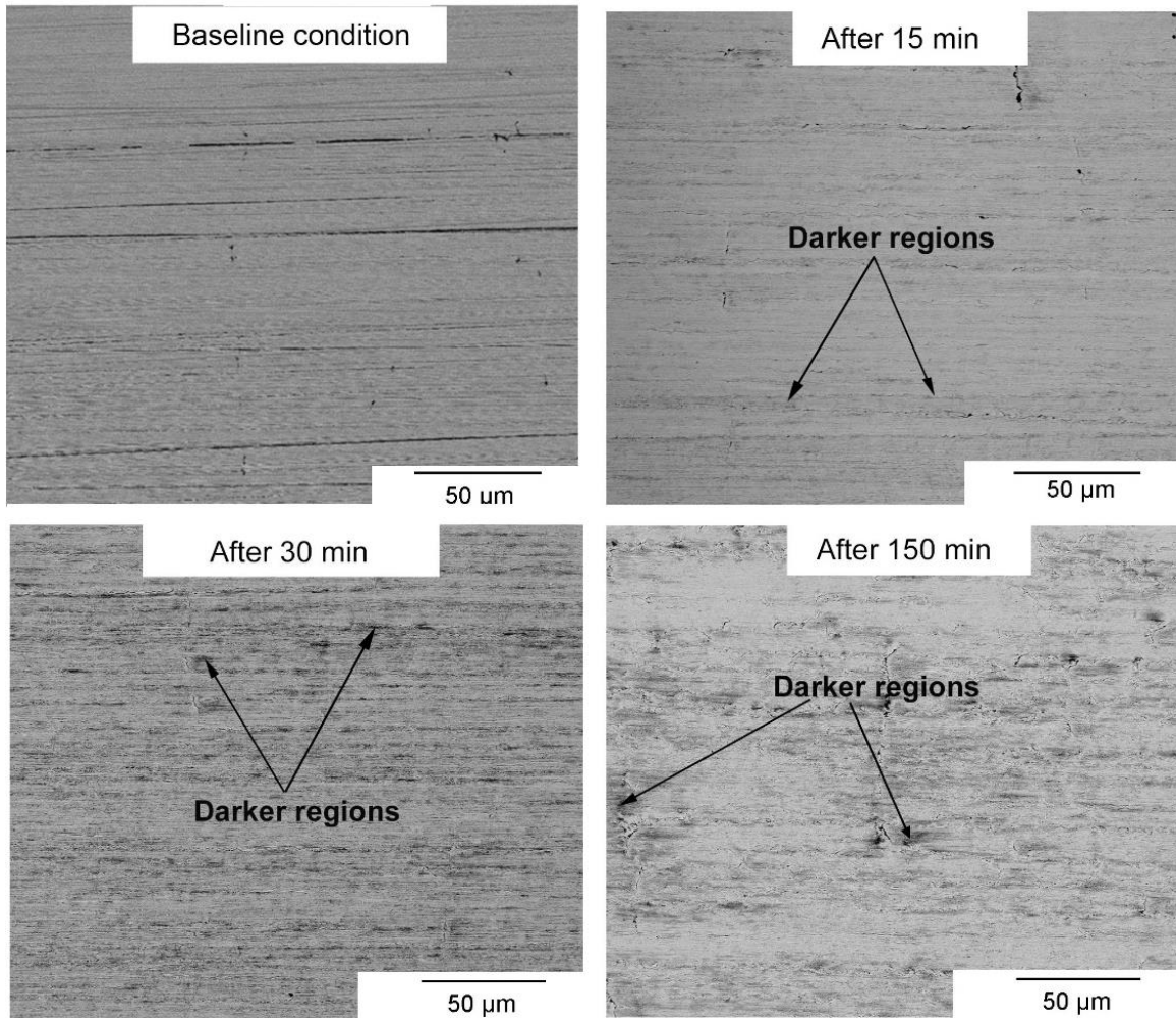
Figure 19. Backscatter image inside the wear track of roller throughout the evolution of tribofilm under condition C. Dark spots indicate regions of tribofilm formation.
