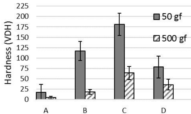
Figure 10. Relative hardness (hardness inside contact zone minus hardness outside contact zone) per test conditions A-D. Average of 36 values are shown along with a 90% confidence interval.
