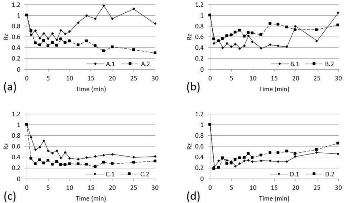
Figure 8. Evolution of normalized Rz, first 30 minutes of test, for complete test duration for (a) test A replicates, (b) test B replicates, (c) test C replicates, and (d) test D replicates.
