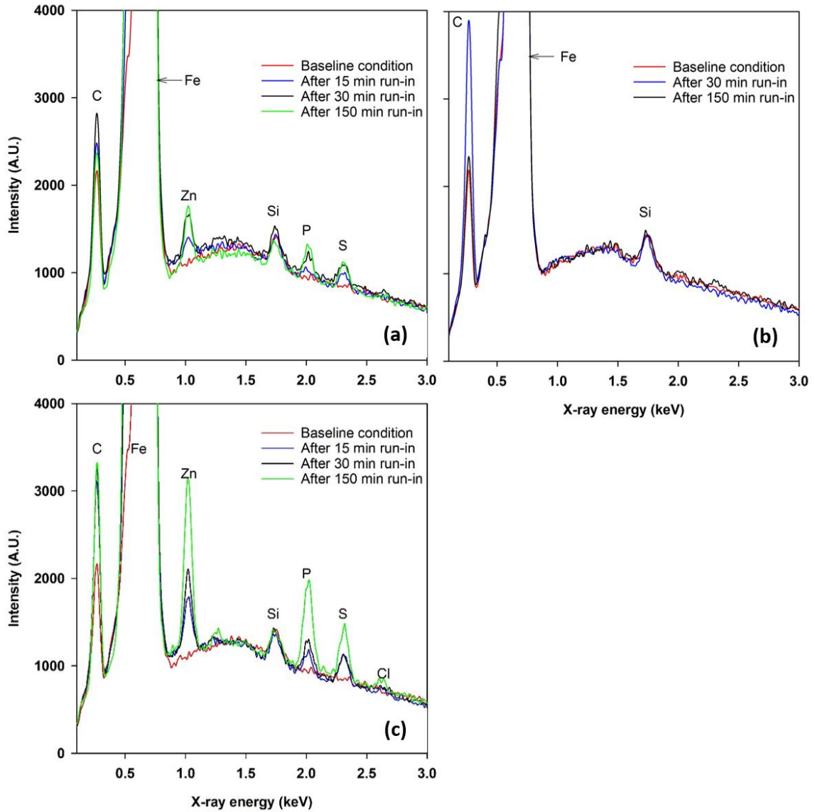
Figure 20. (a) EDS spectrum data measured inside the wear zone under condition C with ZDDP anti-wear additive. (b) EDS spectrum data measured inside the wear zone under condition E with Group II Base Oil (Absent ZDDP). (c) EDS spectrum data of dark regions/zones. Tribofilm formation increases with time in localized regions (c), but stabilizes after 30-min when averaged across wear track.
