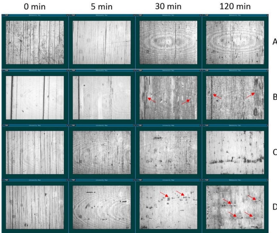
Figure 6. Illustrative surface images of the roller at 0, 5, 30, and 120 minutes for the various test conditions.
