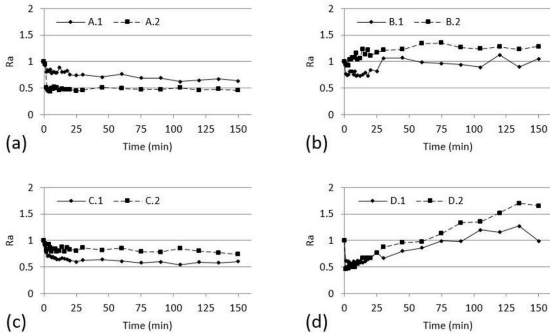
Figure 4. Evolution of normalized Ra for complete test duration for (a) test A replicates, (b) test B replicates, (c) test C replicates, and (d) test D replicates.
