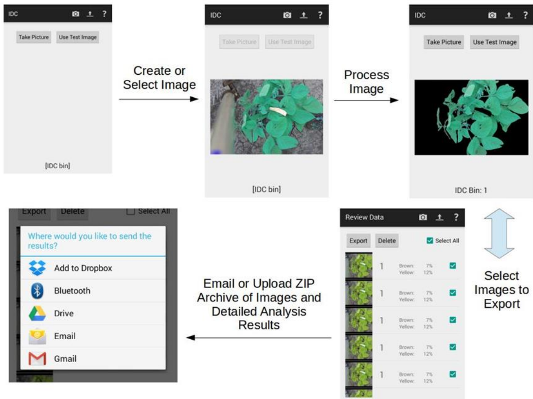
Figure 6: Smartphone app flowchart demonstrating the integration of pre-processing, machine learning enabled classification and iron deficiency chlorosis visual rating in real time.
