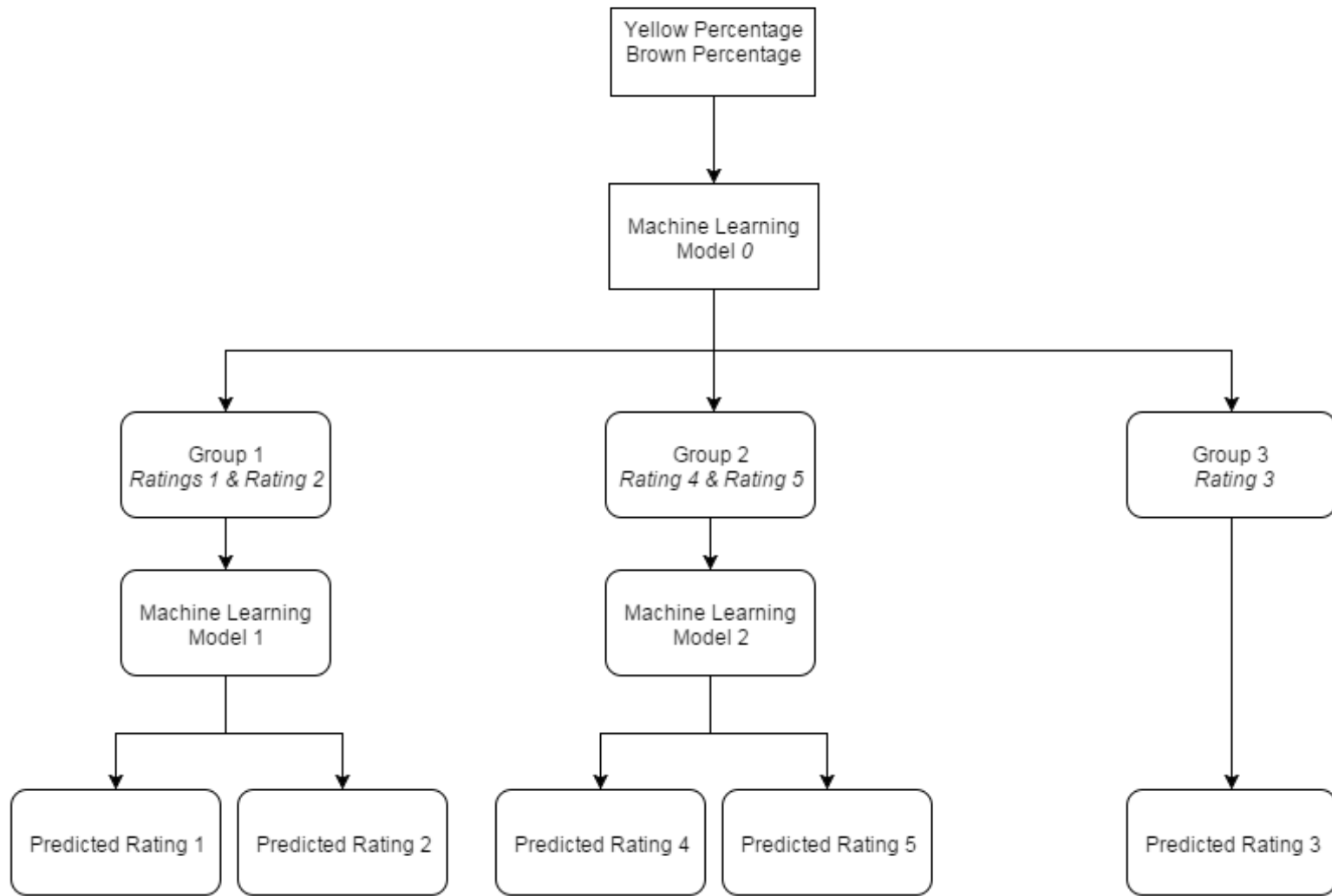
Figure 4. Hierarchical classification workflow
