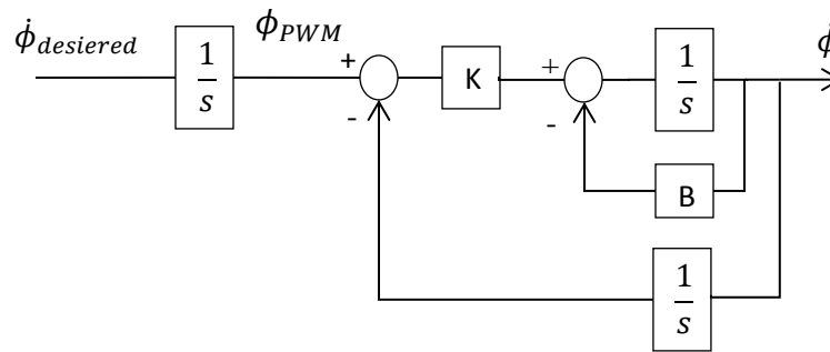
Figure 8. Velocity commanded servo system functional block diagram
