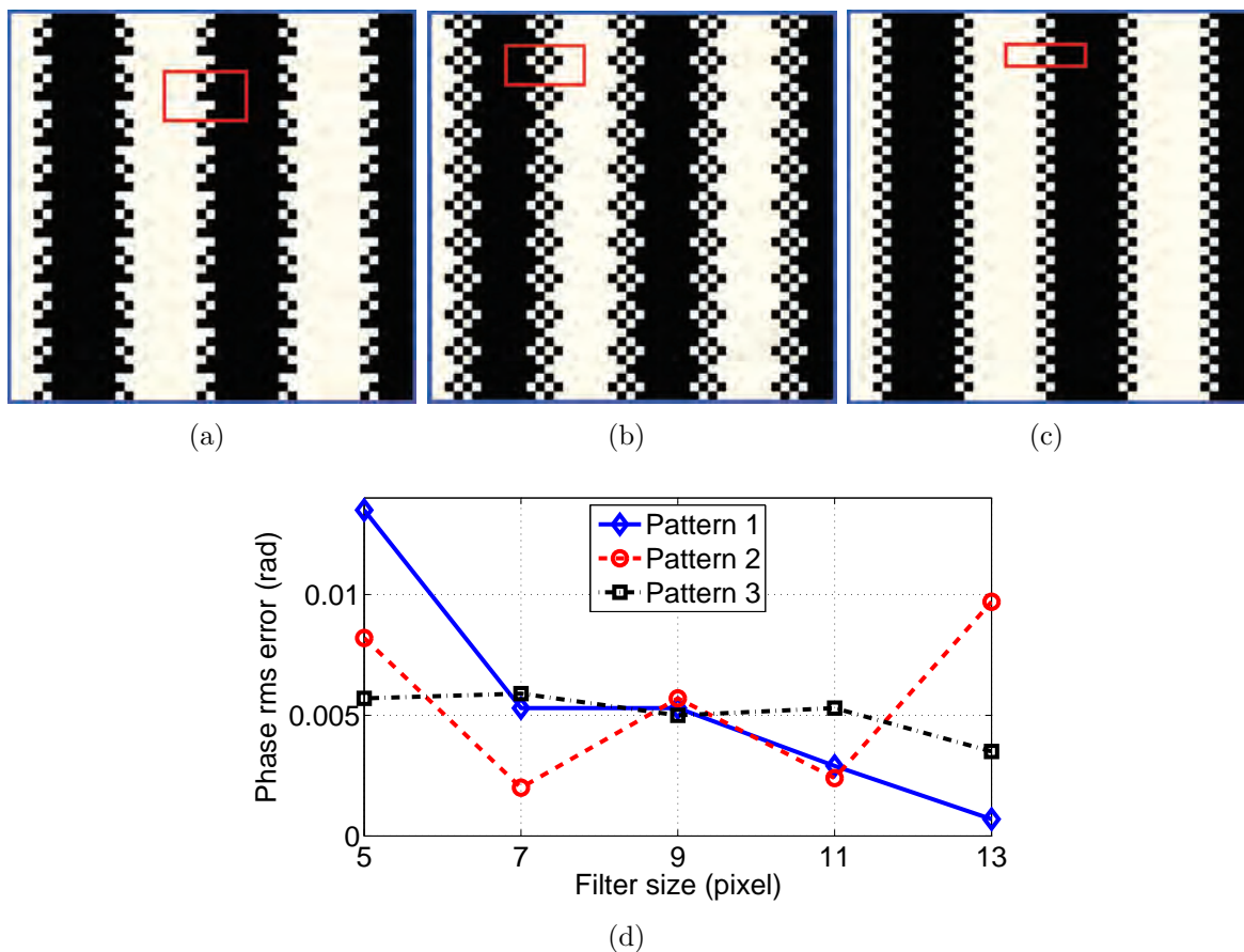
Figure 4.7 Example of selecting the pattern from the optimized binary patches. (a) Pattern 1: T = 18 , S_y = 5 ; (b) pattern 2: T = 18 , S_y = 4 ; (c) pattern 3: T = 18 , S_y = 2 ; (d) phase rms error with different amounts of defocusing.
