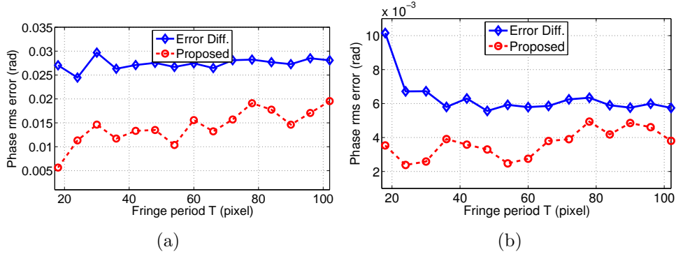
Figure 4.8 Comparing the phase quality between the proposed method and the Floyd-Steinberg error-diffusion technique. (a) Gaussian filter size of 5 \times 5 pixels and standard deviation of 5/3 pixels; (b) Gaussian filter size of 13 \times 13 pixels and standard deviation of 13/3 pixels.
