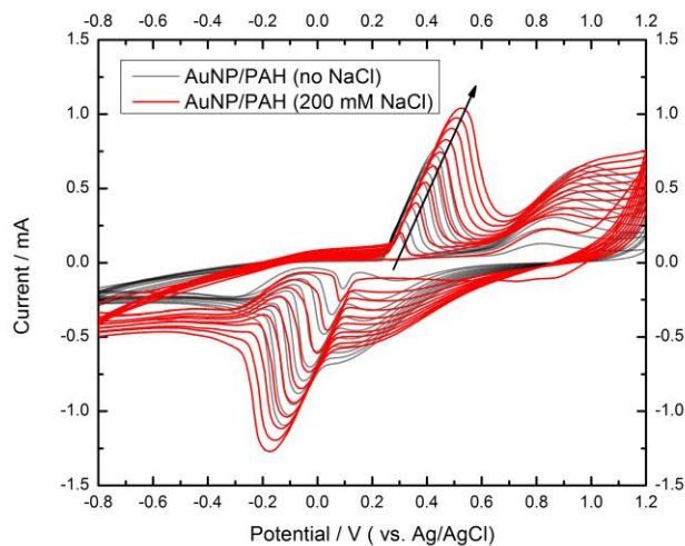
Fig. 4.4 Cyclic voltammograms of AuNPs/PAH thin-film taken at 10-100 mV/s scan rates (10 mV/s increments). Black lines represent CV result of thin-film with no NaCl in PAH solution while the red lines represent CV result of thin-film with 200 mM NaCl in PAH solution. Arrow indicates increasing scan rate.
