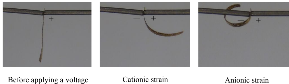
Fig. 2.8 Photographic images of an IPMC-based actuator with 30 bilayers of AuNPs/PAH in CNC; electrode on the right side is anode.
