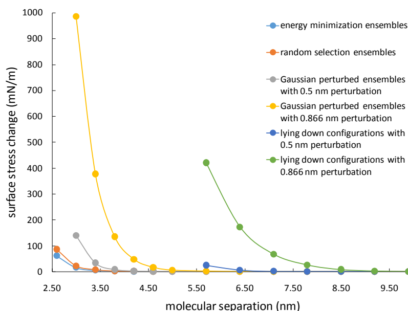
Figure 28. Modeling results of surface stress change with considerations of all molecular ensembles and configurations for single-thiolated approach
