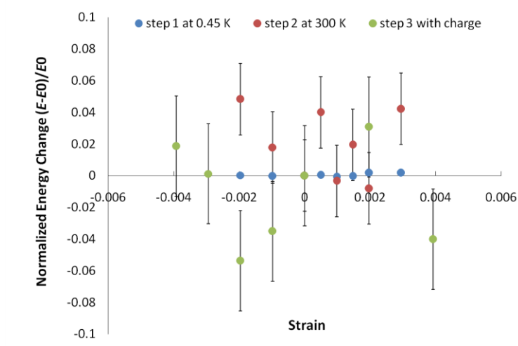
Figure 13. Normalized energy changes with respect to strain
