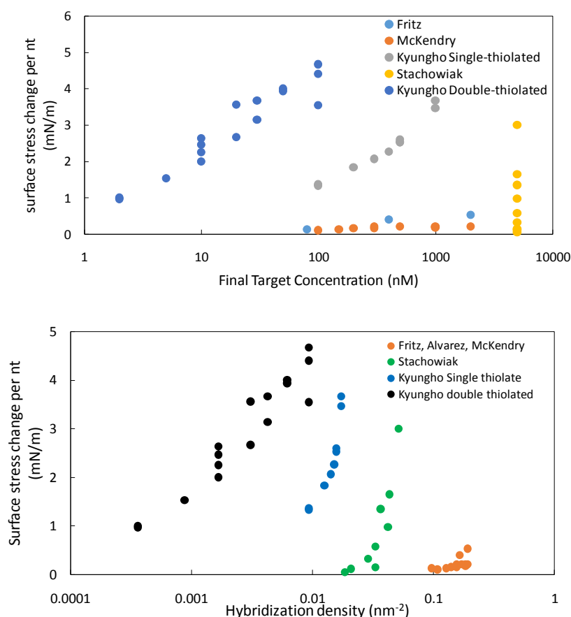
Figure 24. Collections of experimental observations: (a) surface stress change vs. final target concentration; (b) surface stress change vs. hybridization density.
