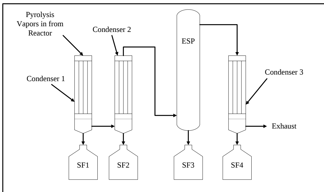
Figure 2: Conventional bio-oil recovery system diagram.
