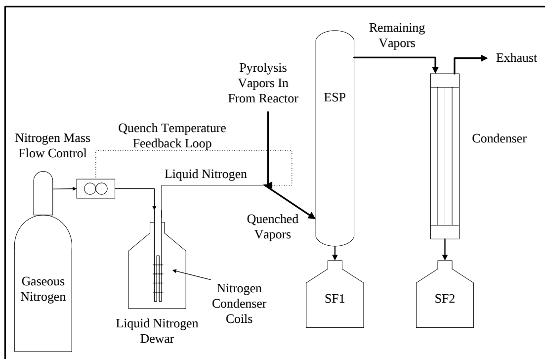
Figure 3: Cold-gas quench bio-oil recovery system diagram.
