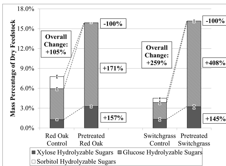
Figure 3: Total sugar yields from control and AAEM passivated feedstocks.
