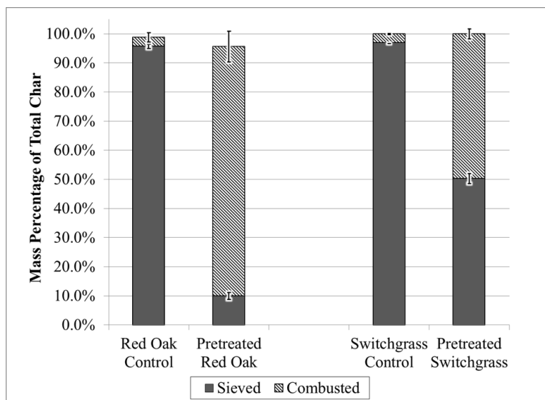
Figure 11: Char separation comparison for control and AAEM passivated feedstocks.
