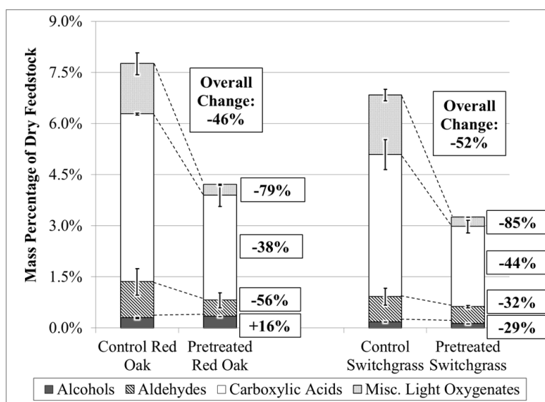
Figure 5: Light oxygenates yield from control and AAEM passivated feedstocks.
