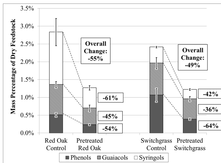
Figure 9: Volatile lignin product yields from control and AAEM passivated feedstocks.
