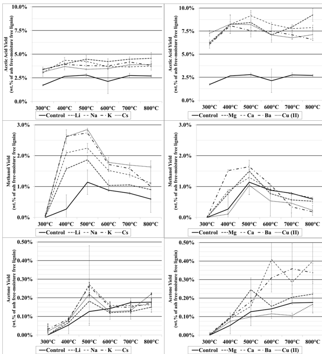
Figure 5: Light oxygenates mass yield; Acetic acid mass yield (Row 1), Methanol mass yield (Row 2), Acetone mass yield (Row 3)
