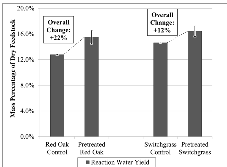
Figure 6: Reaction water yield from control and AAEM passivated feedstocks.
