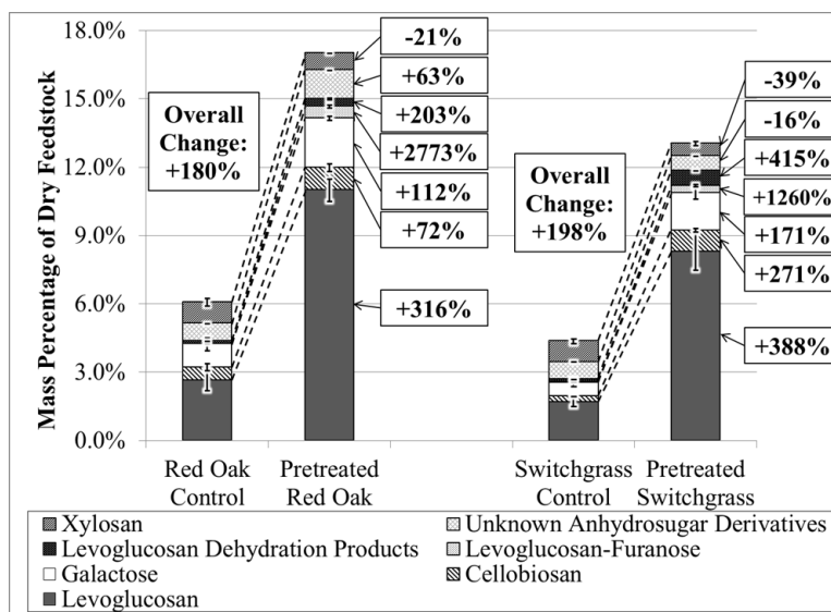
Figure 2: Sugar yield from control and AAEM passivated feedstocks.
