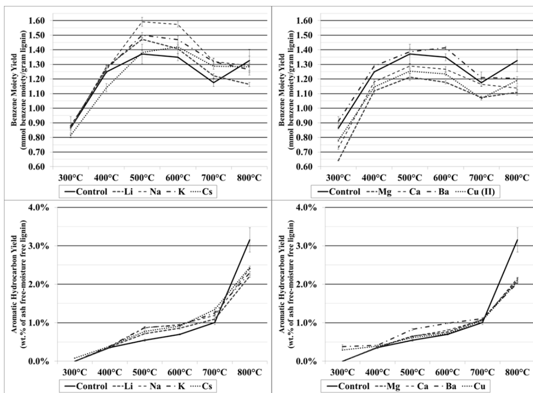
Figure 2: Benzene moiety molar yield (Row 1), Aromatic hydrocarbon mass yield (Row 2)
