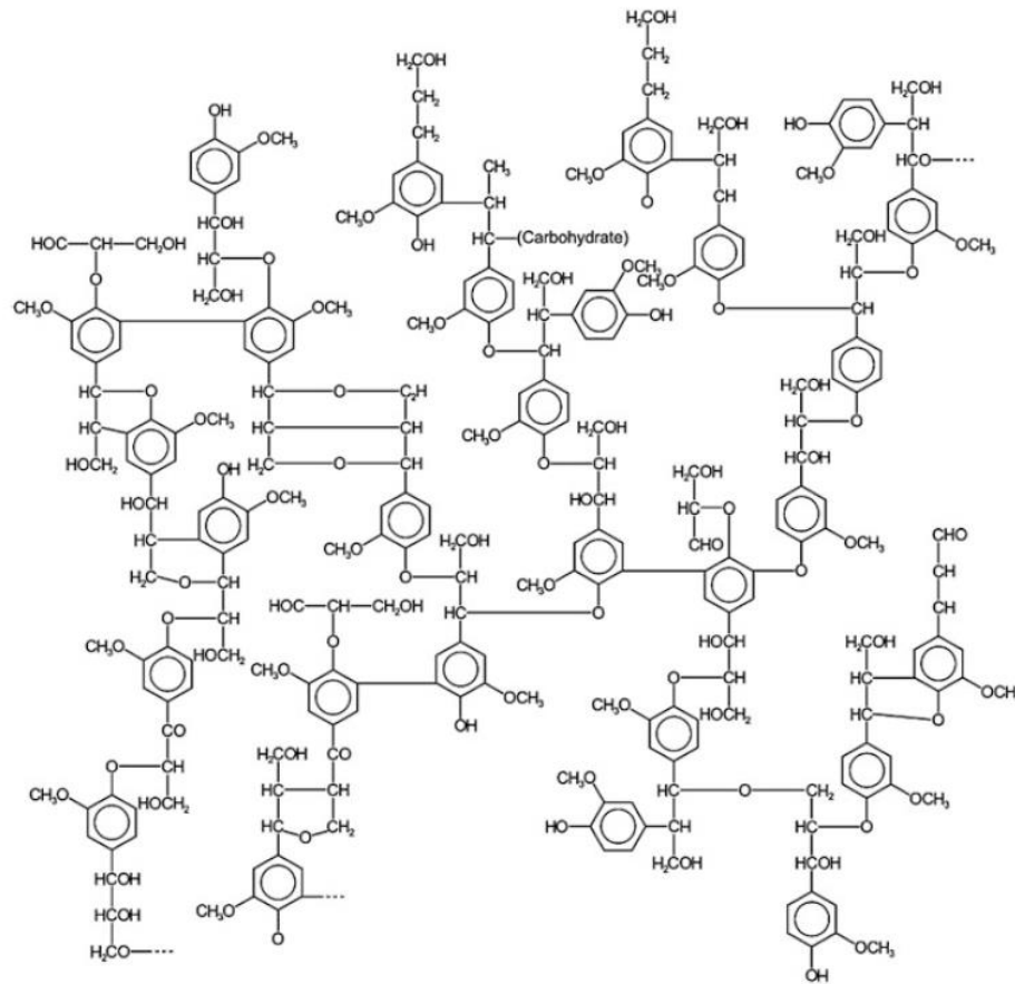
Figure 3: Typical Softwood Lignin Structure [24]
