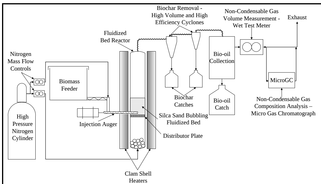
Figure 1: Fluidized bed reactor diagram.
