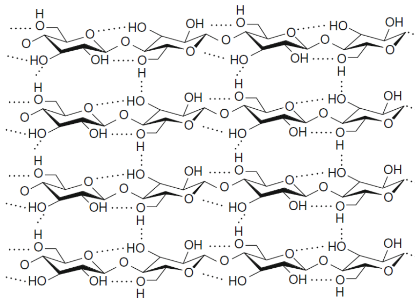
Figure 1: Cellulose structure [14]
