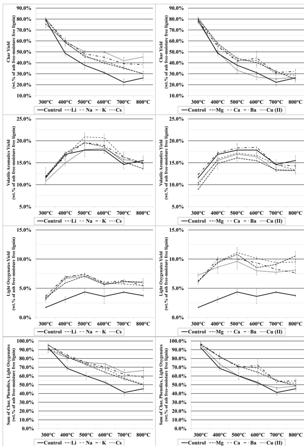
Figure 1: Char mass yield (Row 1), Volatile aromatics mass yield (Row 2), Light oxygenates mass yield (Row 3), Total mass balance (Row 4)
