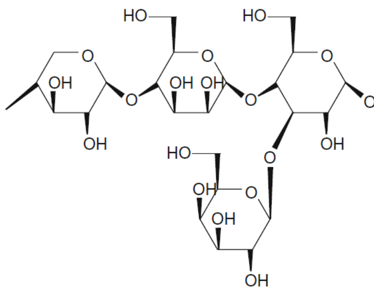
Figure 1: Cellulose structure [14]
