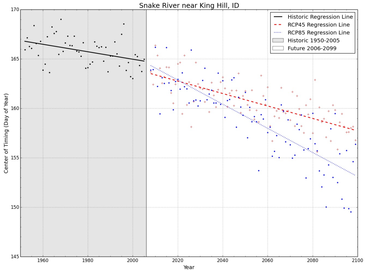
Figure C.10 Center of timing for Snake River at King Hill, showing shaded historic (1950-2005) and future (2006-2099)
