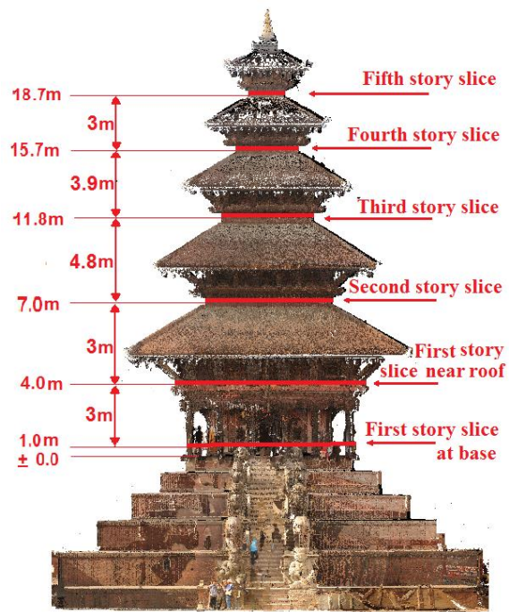
Figure 4.3: Elevation view highlight location of the point cloud slices for floor sections.
