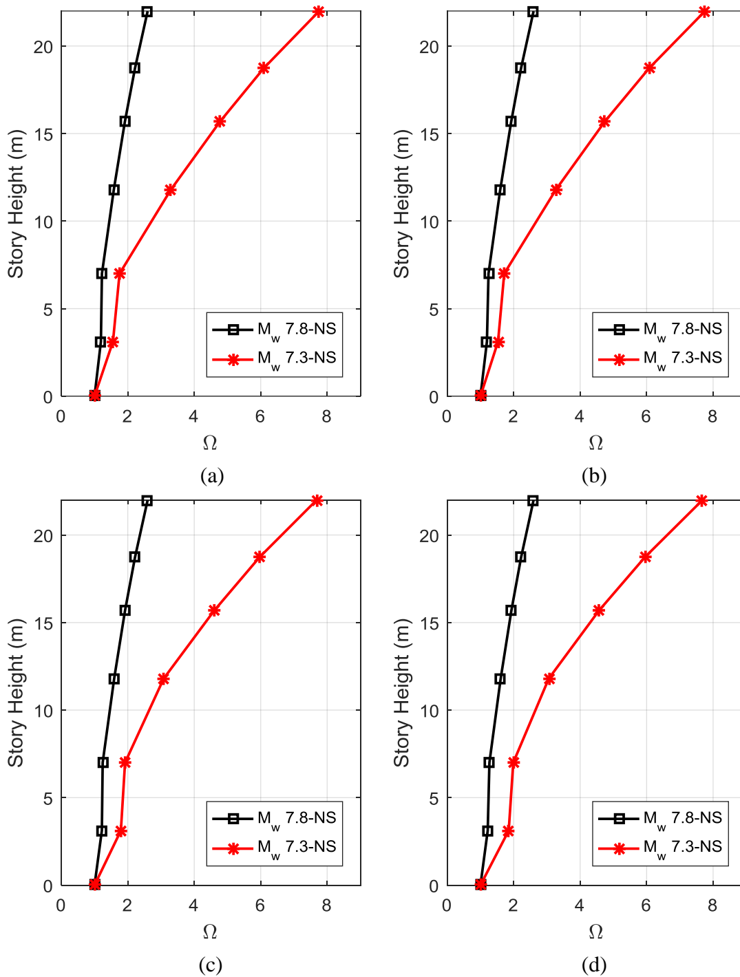
Figure C 1: Uncorrelated acceleration amplification ratio, \Omega , for the Nyatapola temple in the NS direction: (a) south-west corner, (b) north-west corner, (c) north-east corner, and (d) south-east corner.
