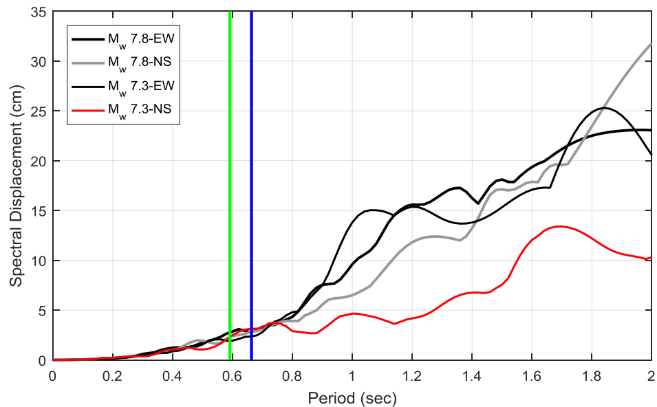
Figure 5.8: Elastic 5% damped spectral displacement curves of Gorkha earthquake (unscaled). Mainshock ( M_w 7.8) and aftershock ( M_w 7.3) ground motions are recorded at THM station in both NS and EW directions. The green and blue vertical lines identify the fundamental periods of the pre-and post-earthquake FEM, respectively.
