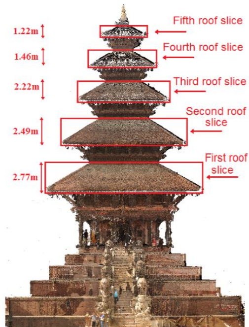
Figure 4.4: Elevation view highlight location and thickness of the point cloud slices for roof sections.
