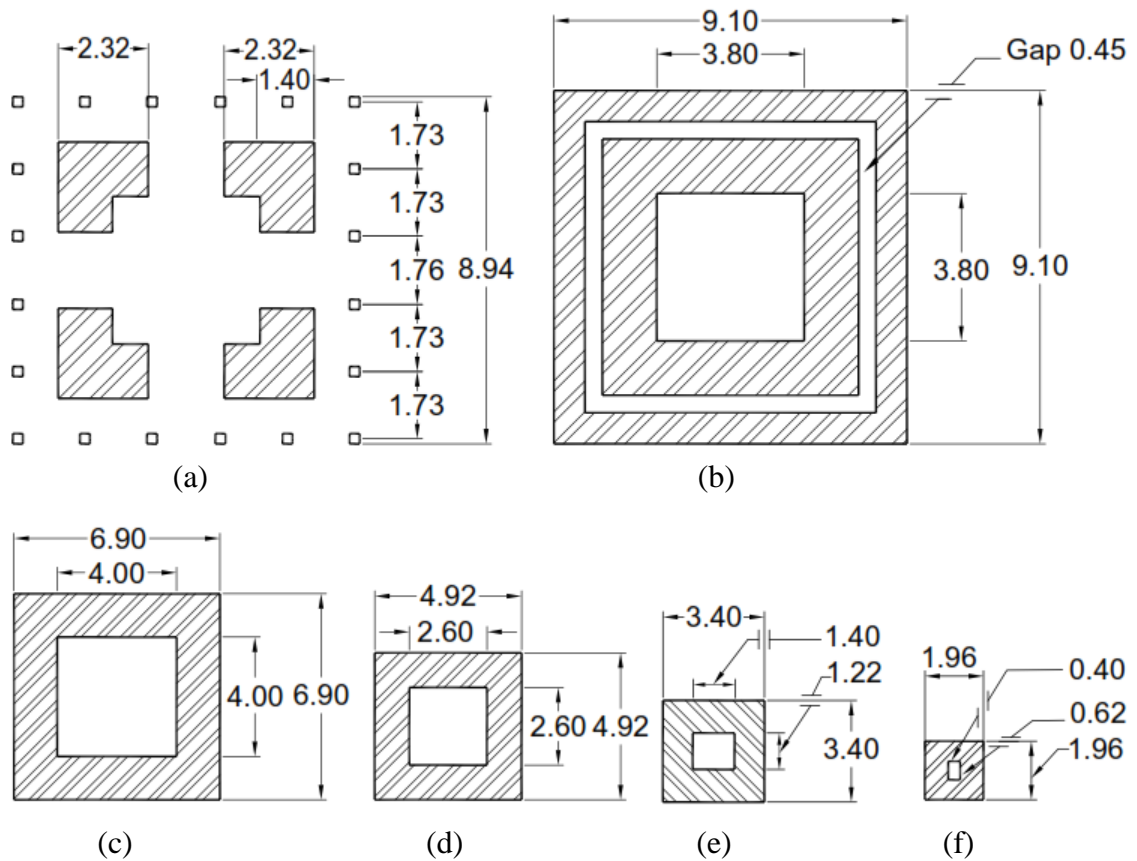
Figure 4.9: Typical FEM cross-section floor of Nyatapola temple, all dimensions in (m): (a) first floor at base [L1a], (b) first floor at 3.12 m [L1b], (c) second floor [L2], (d) third floor [L3], (e) fourth floor [L4], and (f) fifth floor [L5].
