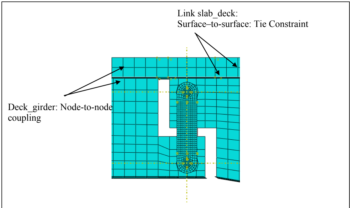
Figure 5.5 Link slab
