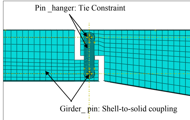
Figure 5.4 Pin and hanger assembly model
