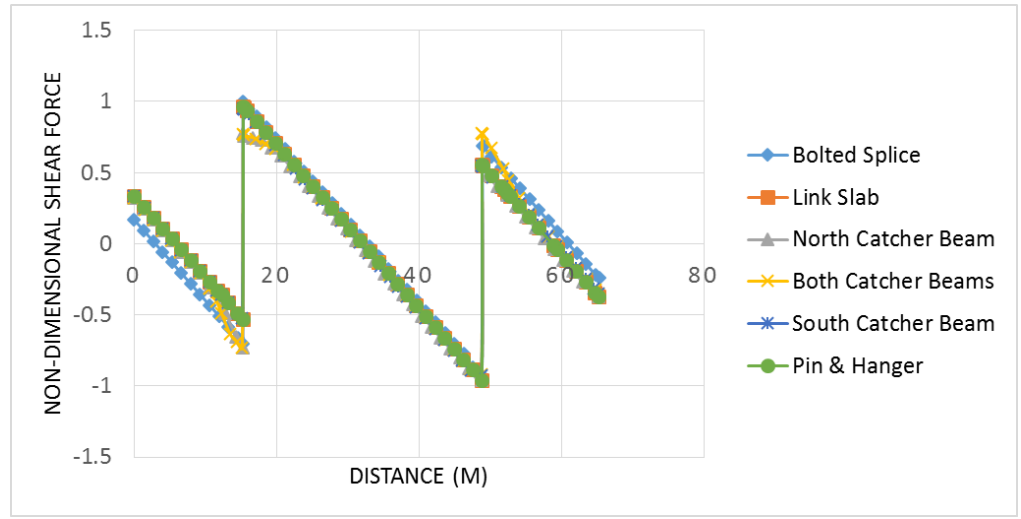
Figure E.2 Non-dimensionalized DC1 shear diagrams at pier 1
