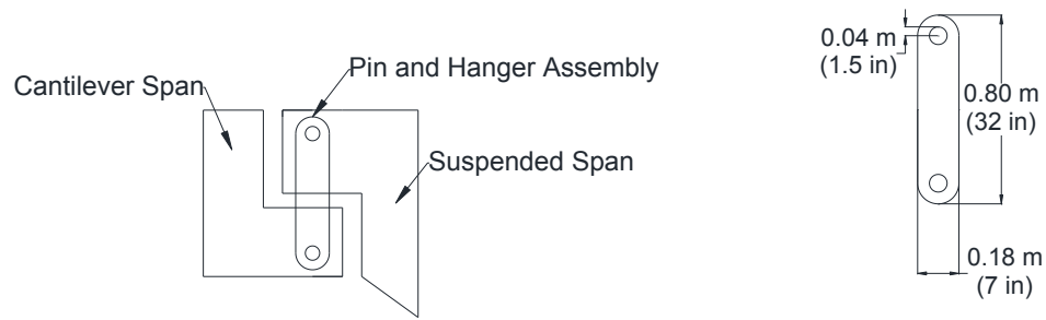
Figure 5.3 Pin and hanger assembly
