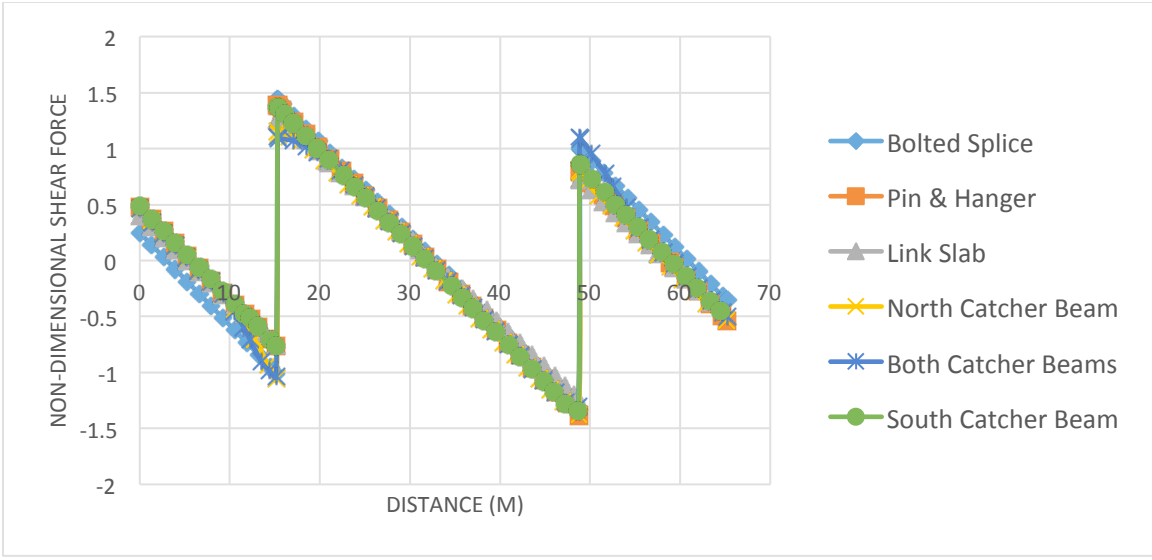
Figure 5.12 Non-dimensionalized shear diagrams for dead loads at Pier 2
