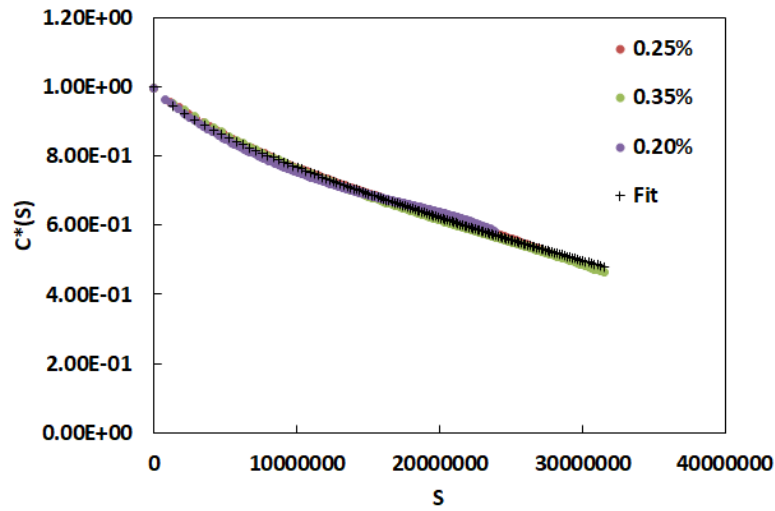
Figure 5.30 Damage characteristic curve for unaged sand asphalt
