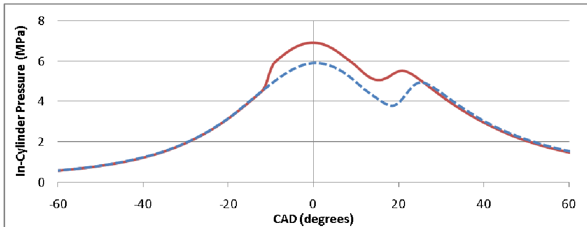
Figure 4.56: In-cylinder pressure versus crank angle degrees ATDC for 30% EGR, double injection pilot SOI at -30 degrees ATDC
