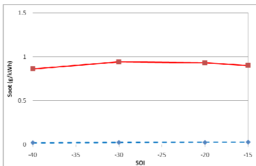
Figure 4.28: Soot versus SOI for 0% EGR, double injection
