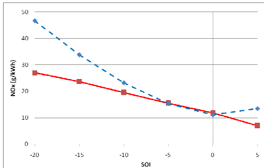
Figure 4.23: NO x versus SOI for 0% EGR, single injection
