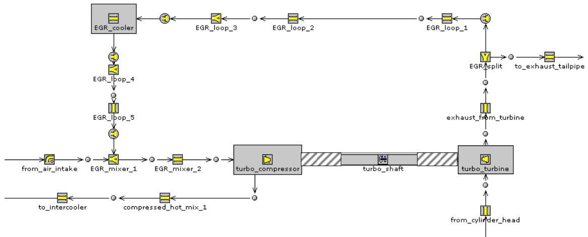
Figure 5.2: Low pressure EGR loop
