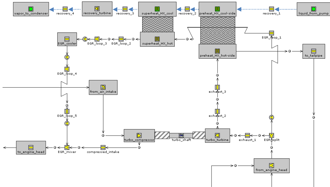
Figure 5.9: Design 3 coupled to high pressure EGR loop
