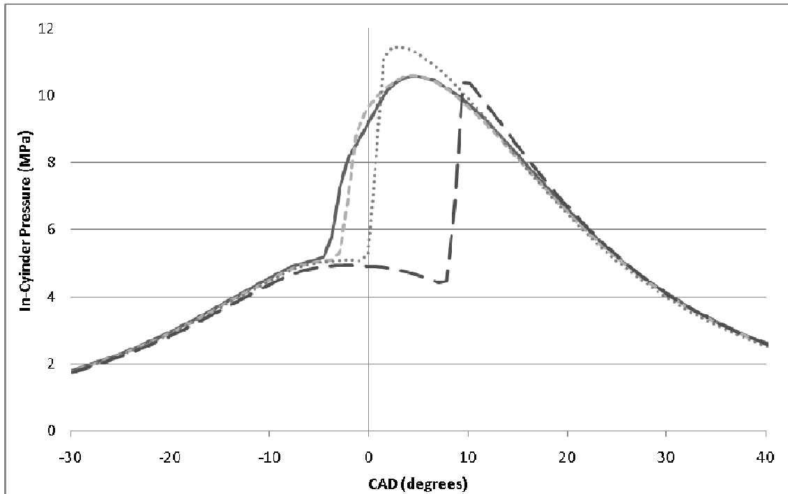
Figure 4.67: In-cylinder pressure versus crank angle degrees ATDC for 30% (solid line), 40% (line with short dashes), 50% (dotted line), 60% EGR (line with long dashes); single injection at -10 degrees ATDC
