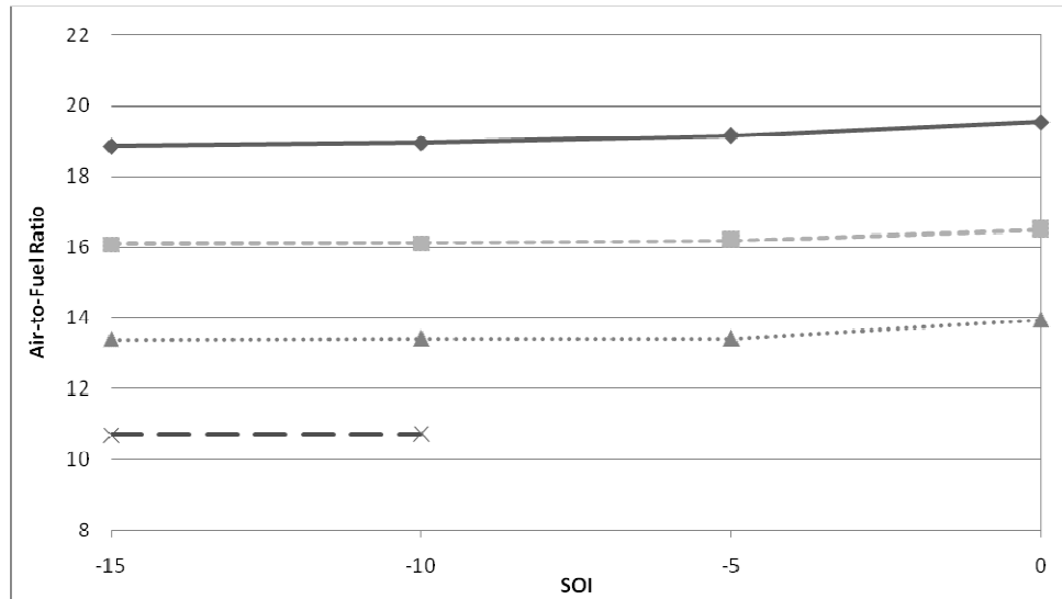
Figure 4.61: GT-Power air-to-fuel ratio versus SOI for 30% (solid line), 40% (line with short dashes), 50% (dotted line), 60% EGR (line with long dashes); single injection
