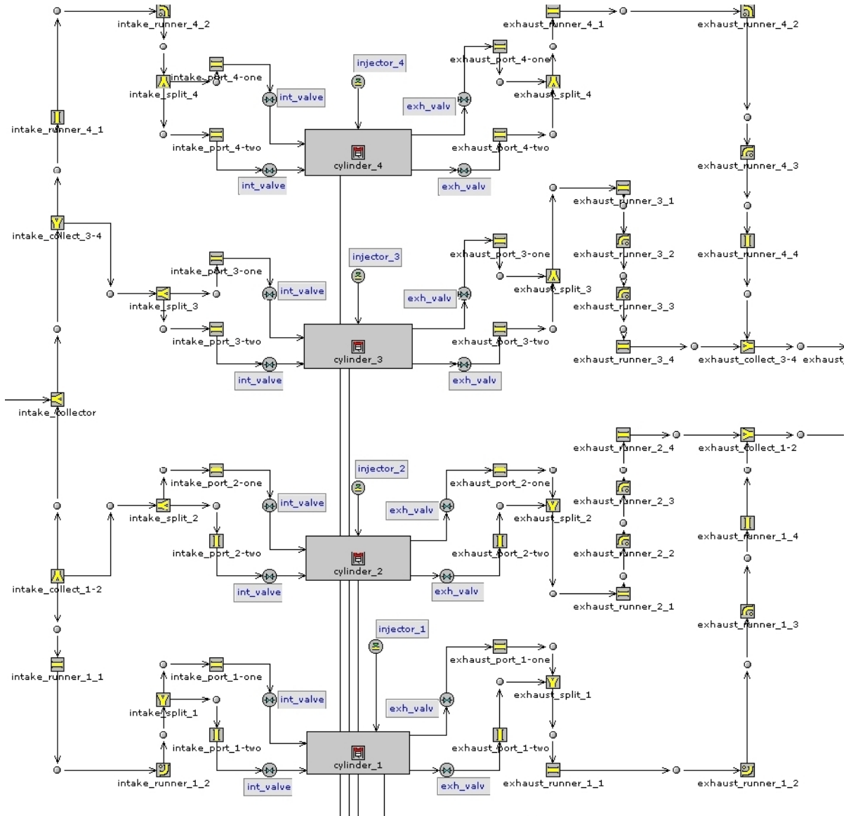
Figure 3.12: GT-Power part assembly page, close-up of engine cylinders and adjacent intake and exhaust piping
