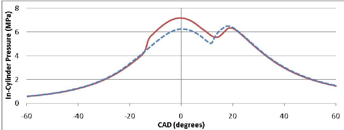
Figure 4.47: In-cylinder pressure versus crank angle degrees ATDC for 0% EGR, double injection pilot SOI at -40 Degrees ATDC
