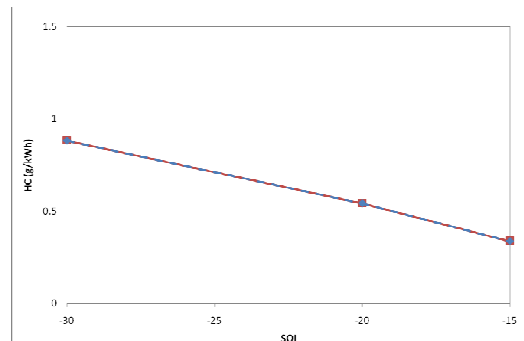
Figure 4.38: HC versus SOI for 30% EGR, double injection; GT-Power results shown after application of correction multipliers
