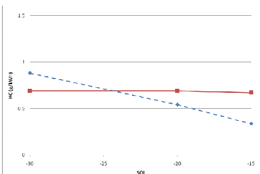
Figure 4.37: HC versus SOI for 30% EGR, double injection; GT-Power results shown before application of correction multipliers
