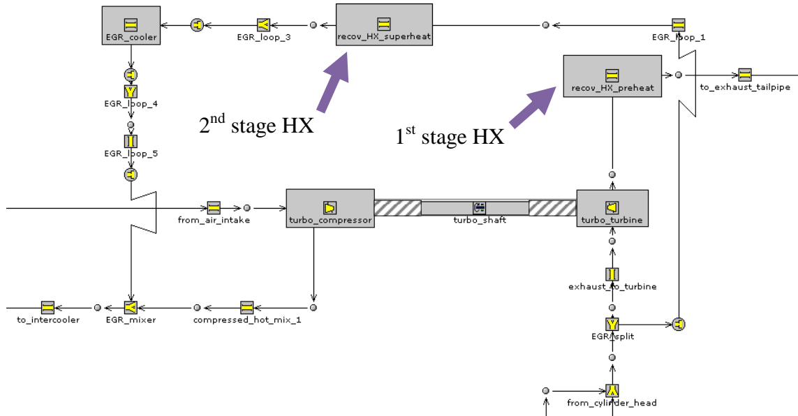
Figure 5.5: High pressure EGR loop with both energy recovery heat exchangers (HX)
