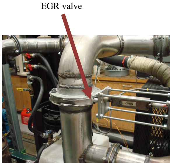
Figure 4.2: Laboratory engine EGR valve, directly upstream of EGR cooler
