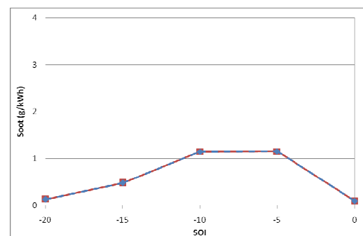
Figure 4.34: Soot versus SOI for 30% EGR, single injection; GT-Power results shown after application of correction multipliers
