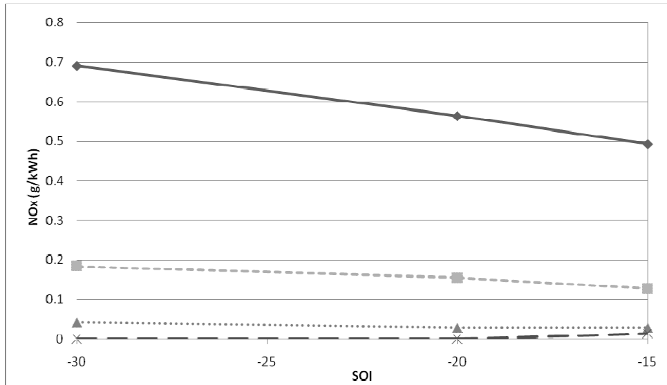
Figure 4.74: GT-Power NO x versus SOI for 30% (solid line), 40% (line with short dashes), 50% (dotted line), 60% EGR (line with long dashes); double injection
