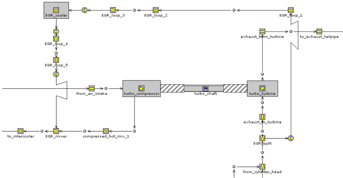
Figure 5.3: High pressure EGR loop
