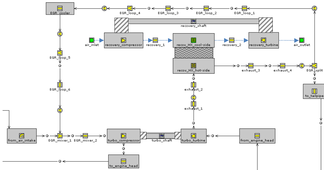
Figure 5.6: Design 1 for energy recovery system
