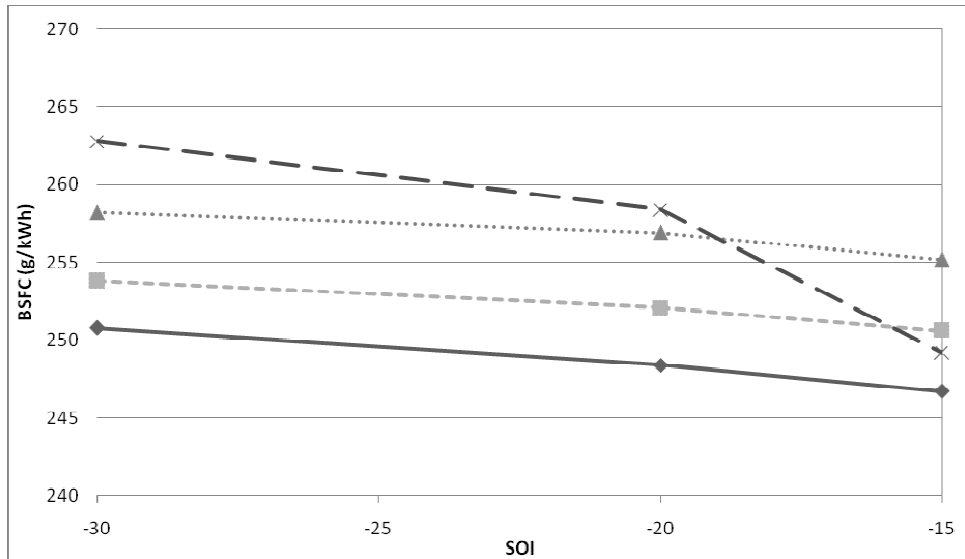
Figure 4.73: GT-Power BSFC versus SOI for 30% (solid line), 40% (line with short dashes), 50% (dotted line), 60% EGR (line with long dashes); double injection
