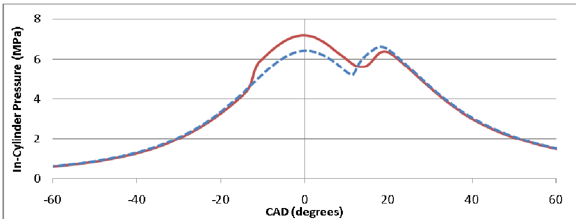
Figure 4.48: In-cylinder pressure versus crank angle degrees ATDC for 0% EGR, double injection pilot SOI at -30 Degrees ATDC
