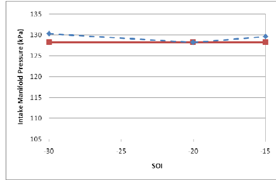
Figure 4.12: Intake manifold pressure versus SOI for 30% EGR, double injection
