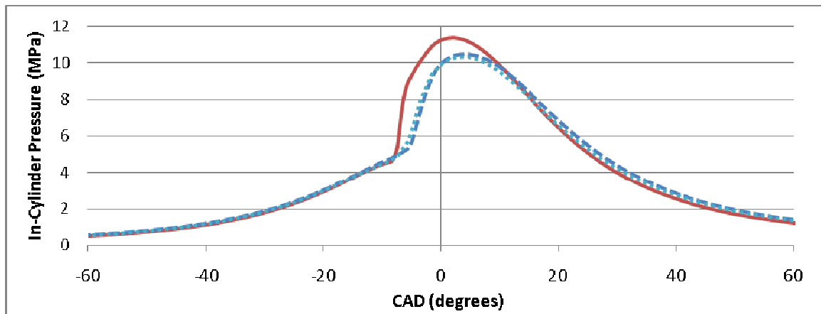
Figure 4.52: In-cylinder pressure versus crank angle degrees ATDC for 30% EGR, single injection at -15 degrees ATDC
