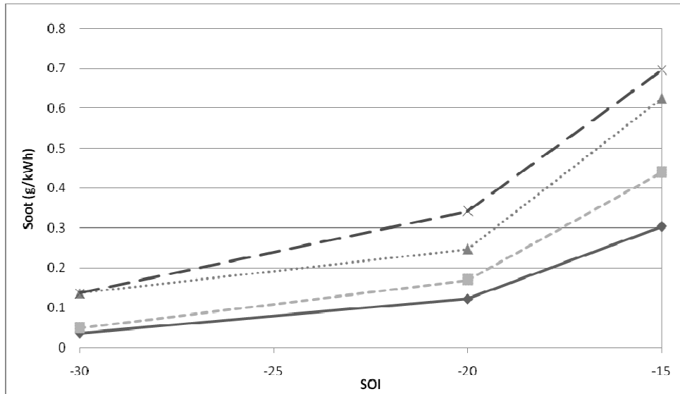
Figure 4.76: GT-Power soot versus SOI for 30% (solid line), 40% (line with short dashes), 50% (dotted line), 60% EGR (line with long dashes); double injection
