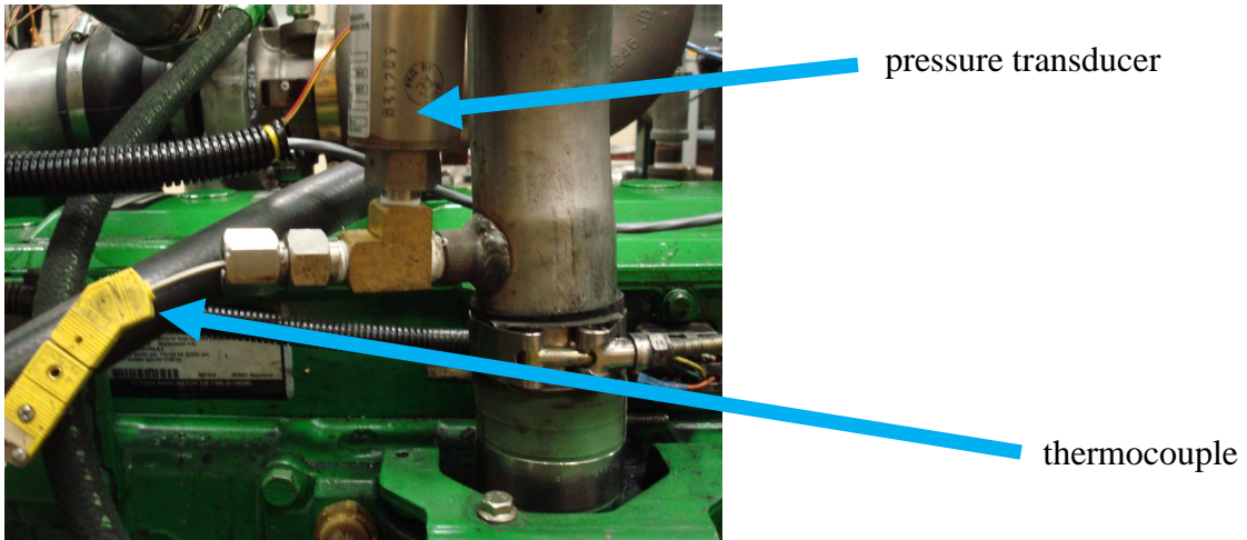
Figure 4.1: Thermocouple and pressure transducer attached to intake manifold via T-fitting
