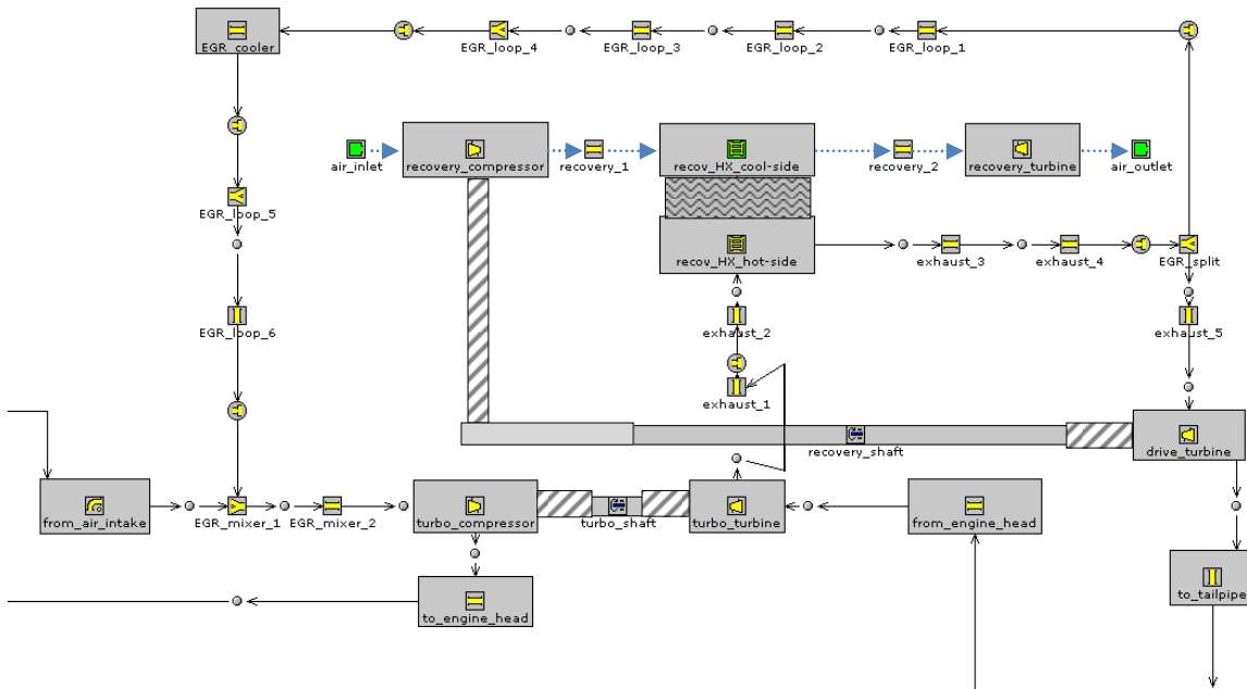
Figure 5.7: Design 2 for energy recovery system
