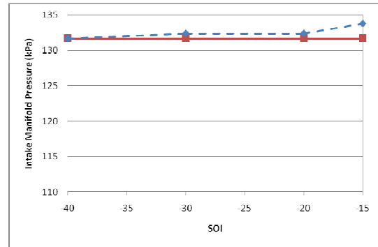
Figure 4.10: Intake manifold pressure versus SOI for 0% EGR, double injection
