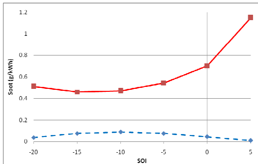
Figure 4.25: Soot versus SOI for 0% EGR, single injection
