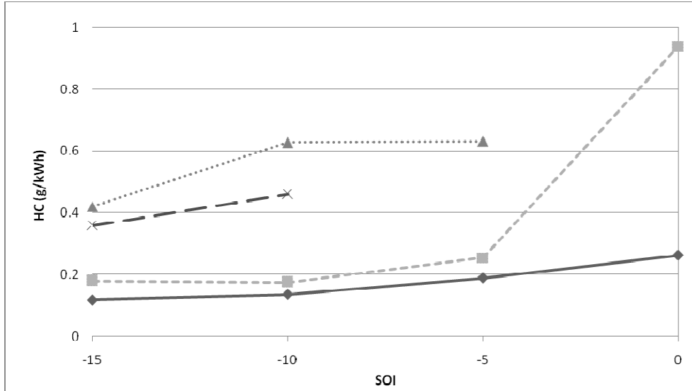
Figure 4.64: GT-Power HC versus SOI for 30% (solid line), 40% (line with short dashes), 50% (dotted line), 60% EGR (line with long dashes); single injection
