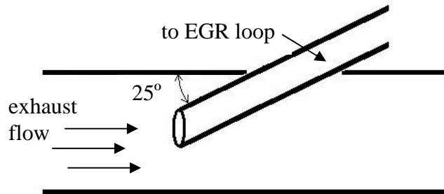
Figure 3.10: EGR-split showing inlet to EGR loop
