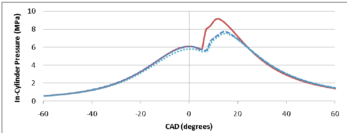
Figure 4.45: In-cylinder pressure versus crank angle degrees ATDC for 0% EGR, single injection at 0 degrees ATDC
