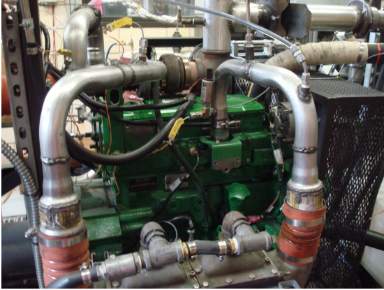
Figure 3.1: John Deere 4.5L diesel engine
