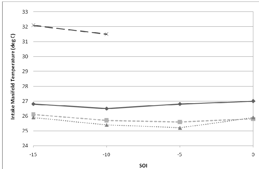
Figure 4.59: GT-Power intake manifold temperature versus SOI for 30% (solid line), 40% (line with short dashes), 50% (dotted line), 60% EGR (line with long dashes); single injection
