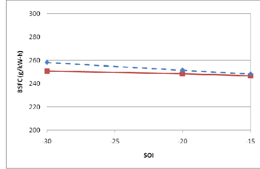
Figure 4.22: BSFC versus SOI for 30% EGR, double injection
