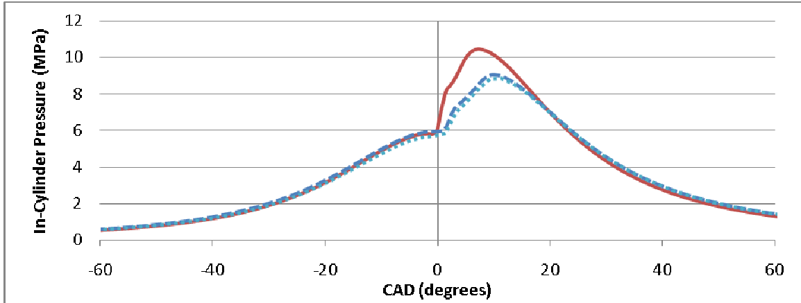
Figure 4.44: In-cylinder pressure versus crank angle degrees ATDC for 0% EGR, single injection at -5 degrees ATDC
