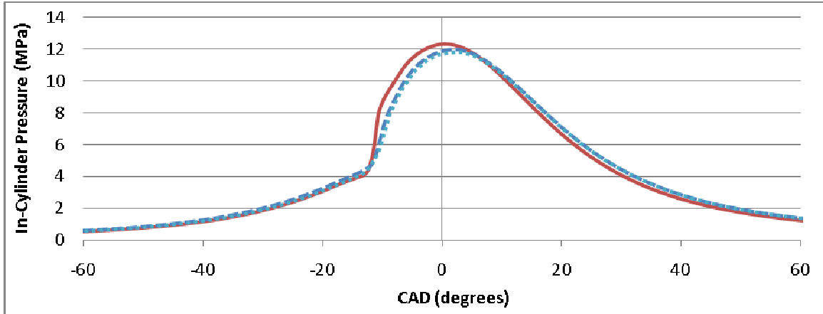
Figure 4.41: In-cylinder pressure versus crank angle degrees ATDC for 0% EGR, single injection at -20 degrees ATDC
