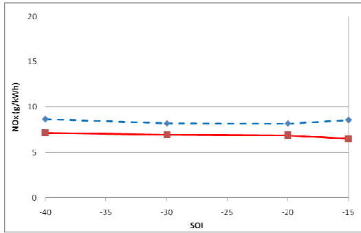
Figure 4.26: NO x versus SOI for 0% EGR, double injection
