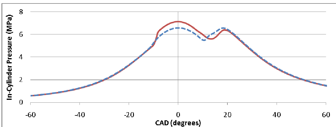
Figure 4.49: In-cylinder pressure versus crank angle degrees ATDC for 0% EGR, double injection pilot SOI at -20 Degrees ATDC
