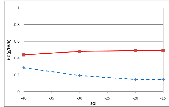
Figure 4.27: HC versus SOI for 0% EGR, double injection
