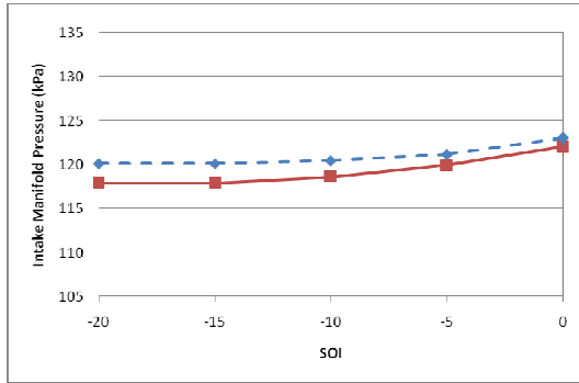
Figure 4.11: Intake manifold pressure versus SOI for 30% EGR, single injection
