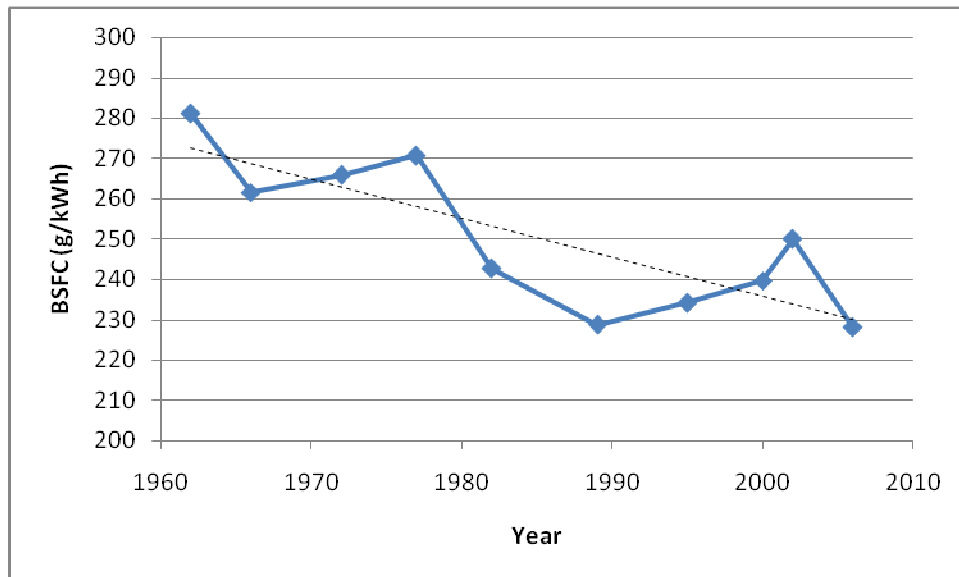
Figure 2.1: BSFC (at rated engine speed) achieved by diesel engine in most powerful John Deere gear-drive row-crop tractor versus tractor model year (solid line); linear trend in average BSFC reduction versus model year (dashed line)
