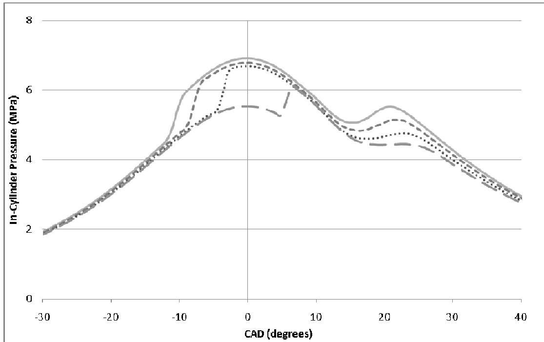
Figure 4.77: In-cylinder pressure versus crank angle degrees ATDC for 30% (solid line), 40% (line with short dashes), 50% (dotted line), 60% EGR (line with long dashes); double injection pilot SOI at -30 degrees ATDC
