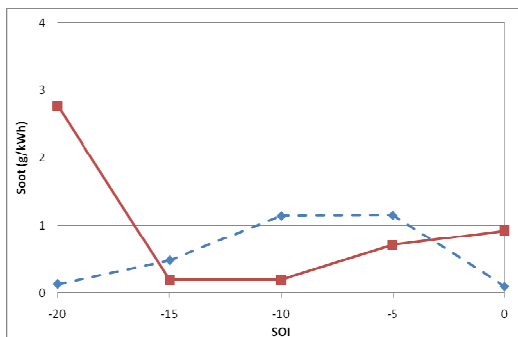
Figure 4.33: Soot versus SOI for 30% EGR, single injection; GT-Power results shown before application of correction multipliers
