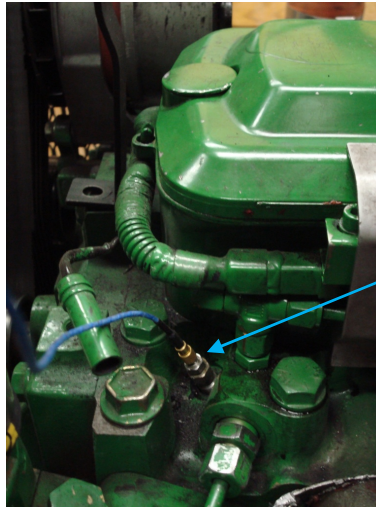
Figure 4.18: Pressure transducer for in-cylinder pressure, fit into glow plug socket of front-most cylinder
