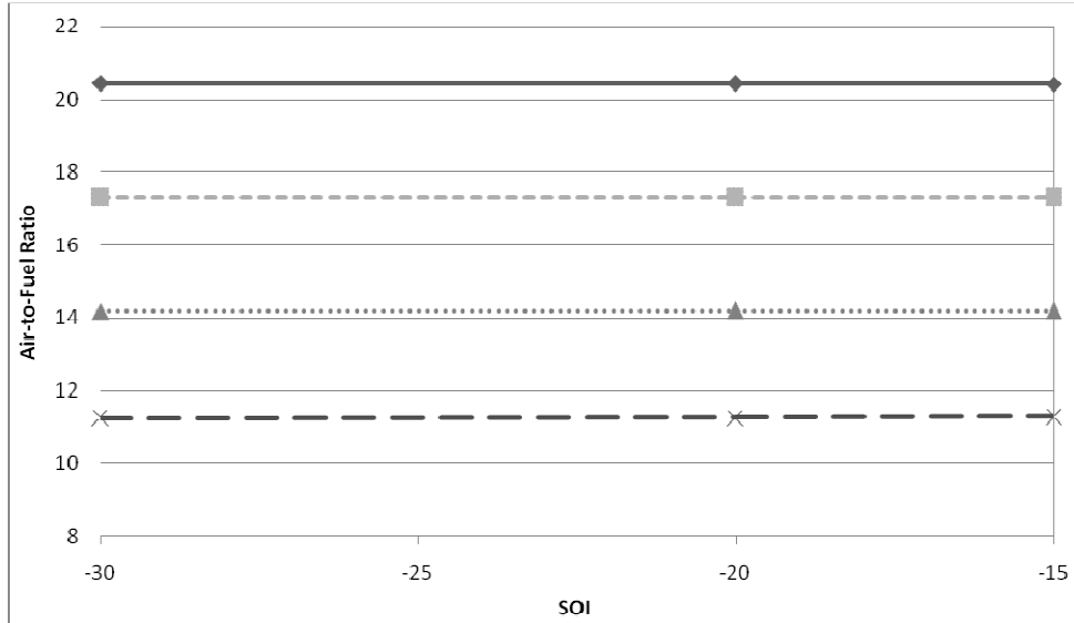
Figure 4.72: GT-Power air-to-fuel ratio versus SOI for 30% (solid line), 40% (line with short dashes), 50% (dotted line), 60% EGR (line with long dashes); double injection
