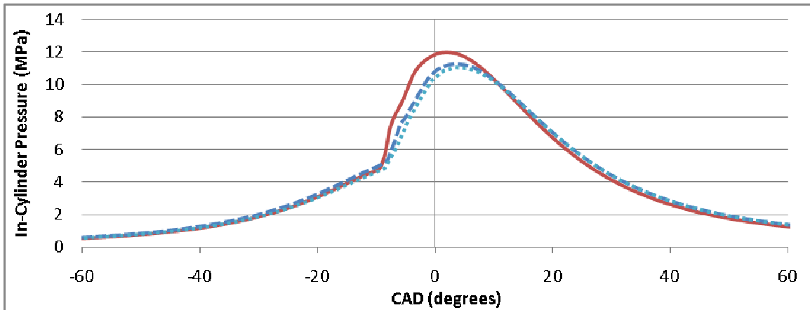
Figure 4.42: In-cylinder pressure versus crank angle degrees ATDC for 0% EGR, single injection at -15 degrees ATDC
