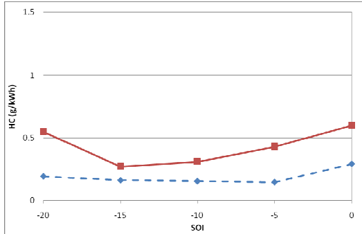
Figure 4.31: HC versus SOI for 30% EGR, single injection; GT-Power results shown before application of correction multiplier
