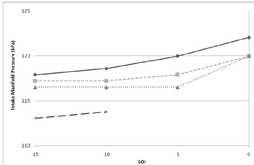
Figure 4.60: GT-Power intake manifold pressure versus SOI for 30% (solid line), 40% (line with short dashes), 50% (dotted line), 60% EGR (line with long dashes); single injection
