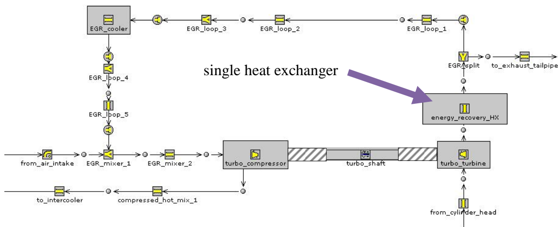
Figure 5.4: Low pressure EGR loop with energy recovery heat exchanger
