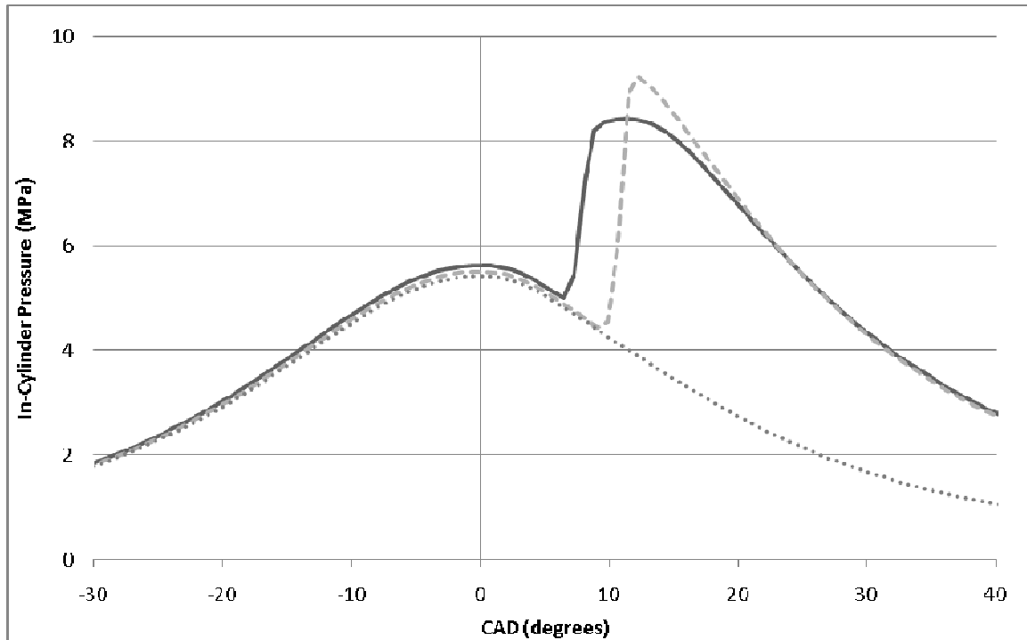
Figure 4.69: In-cylinder pressure versus crank angle degrees ATDC for 30% (solid line), 40% (line with short dashes), 50% EGR (dotted line); single injection at 0 degrees ATDC
