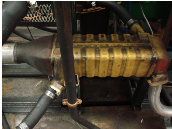
Figure 5.1: Water cooled heat exchanger used to cool EGR gases in laboratory engine setup
