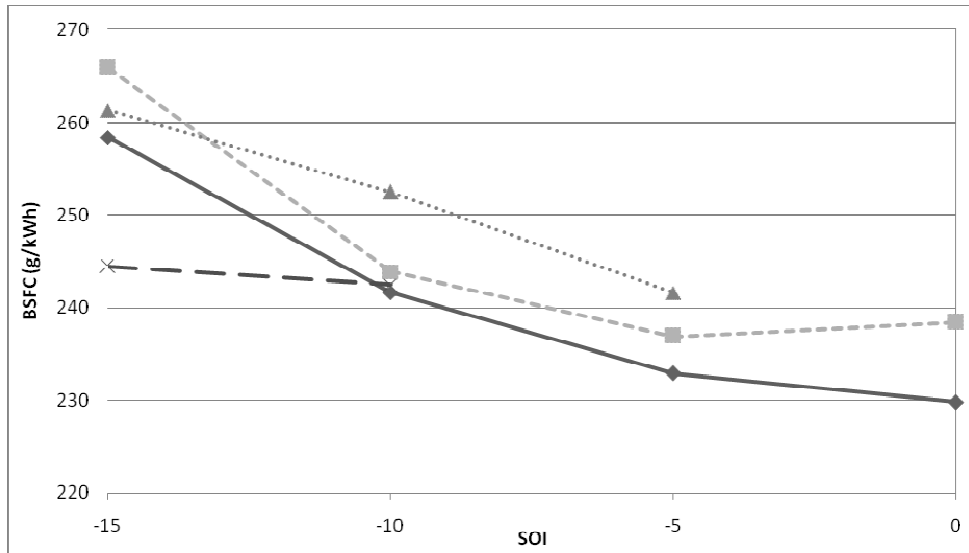
Figure 4.62: GT-Power BSFC versus SOI for 30% (solid line), 40% (line with short dashes), 50% (dotted line), 60% EGR (line with long dashes); single injection
