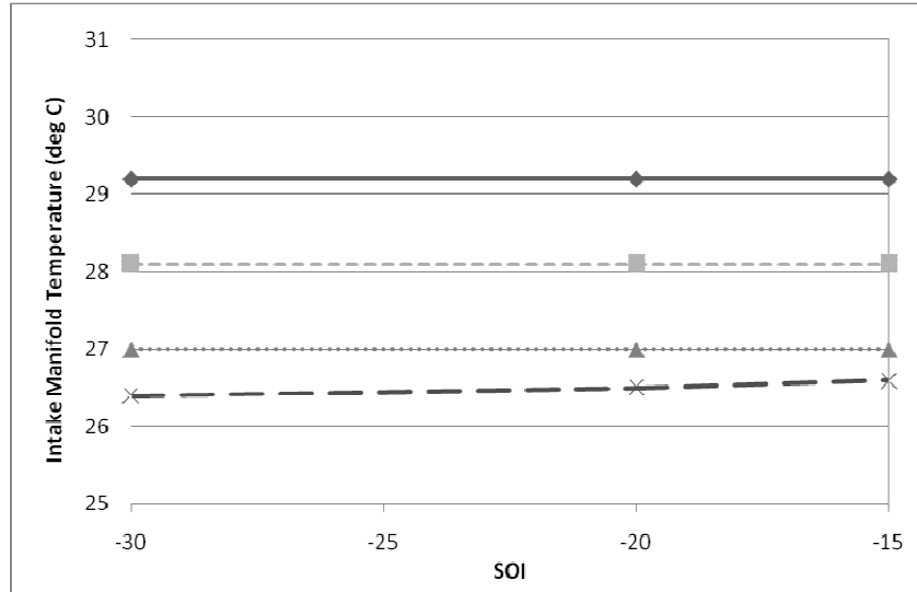
Figure 4.70: GT-Power intake manifold temperature versus SOI for 30% (solid line), 40% (line with short dashes), 50% (dotted line), 60% EGR (line with long dashes); double injection
