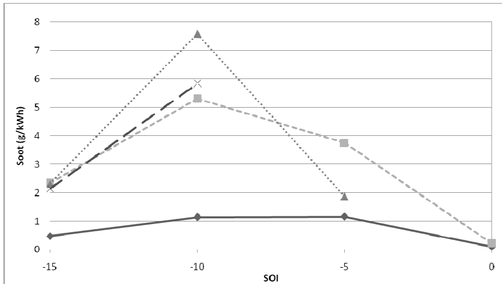
Figure 4.65: GT-Power soot versus SOI for 30% (solid line), 40% (line with short dashes), 50% (dotted line), 60% EGR (line with long dashes); single injection
