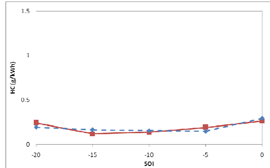
Figure 4.32: HC versus SOI for 30% EGR, single injection; GT-Power results shown after application of correction multiplier
