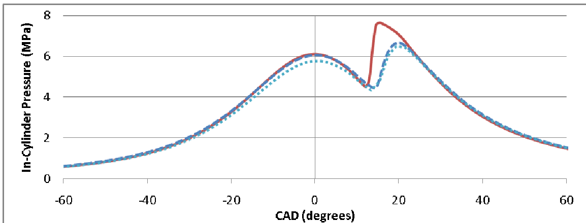
Figure 4.46: In-cylinder pressure versus crank angle degrees ATDC for 0% EGR, single injection at 5 degrees ATDC
