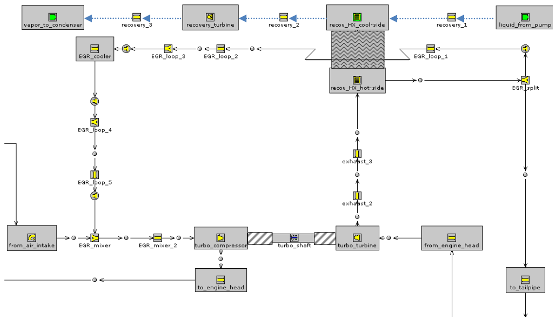
Figure 5.8: Design 3 coupled to low pressure EGR loop
