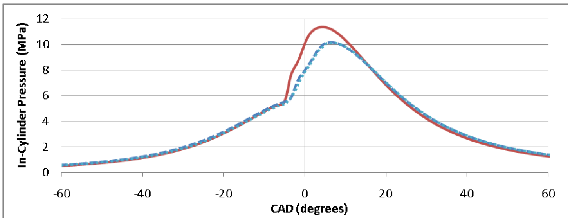
Figure 4.43: In-cylinder pressure versus crank angle degrees ATDC for 0% EGR, single injection at -10 degrees ATDC
