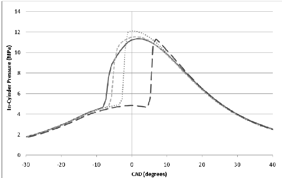
Figure 4.66: In-cylinder pressure versus crank angle degrees ATDC for 30% (solid line), 40% (line with short dashes), 50% (dotted line), 60% EGR (line with long dashes); single injection at -15 degrees ATDC
