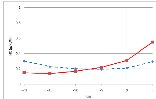
Figure 4.24: HC versus SOI for 0% EGR, single injection
