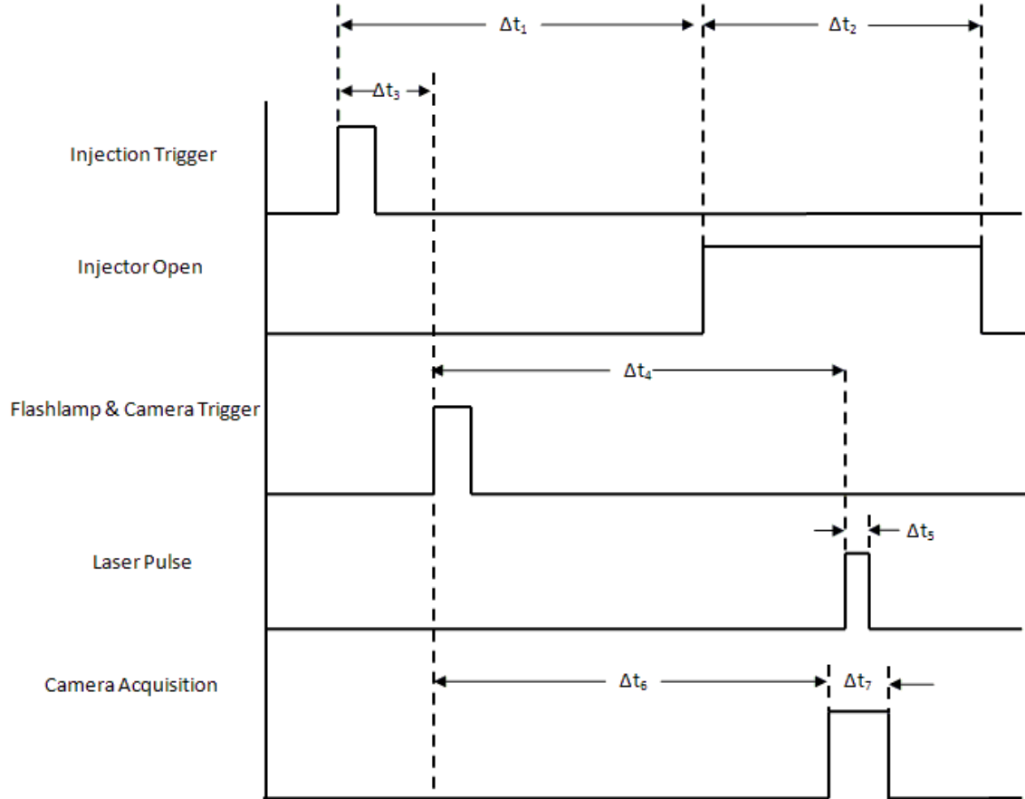
Figure 5: Timing scheme used for the synchronization of events.
