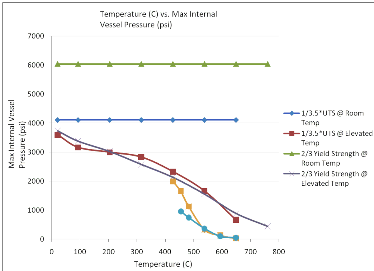
Figure A2: Maximum allowable vessel pressures as a function of temperature
