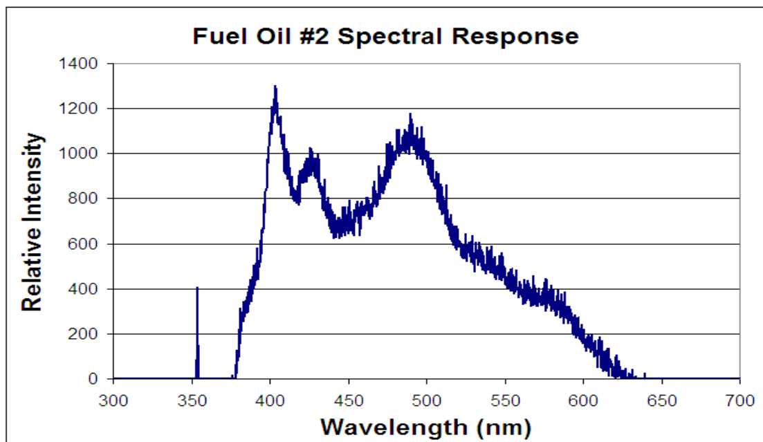
Figure 18: Unfiltered Spectral Response of Fuel Oil #2 with 355nm excitation.
