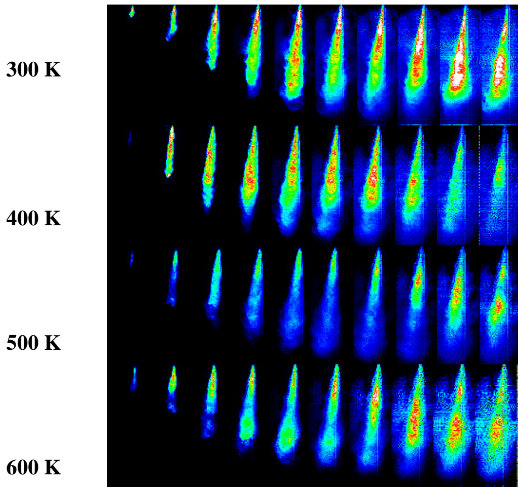
Figure 26: 100 MPa injection sequence into N2 @ 3550 kPa
