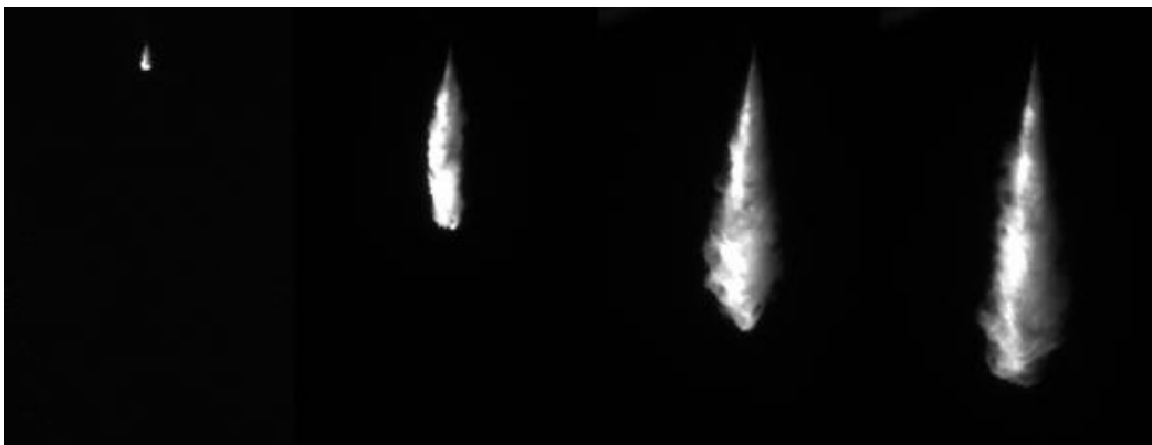
Figure 11: Sequence of injection events at 50, 250, 450, and 650 us ASOI
