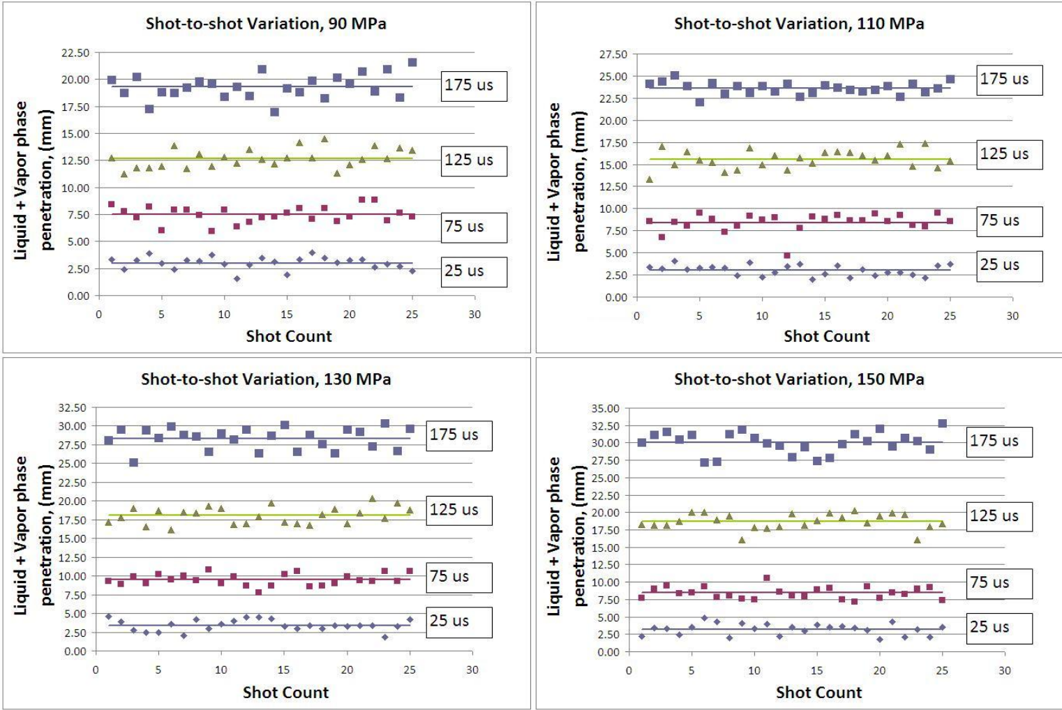
Figure 13: Shot-to-shot variation in penetration distance for the manual injection experimental setup
