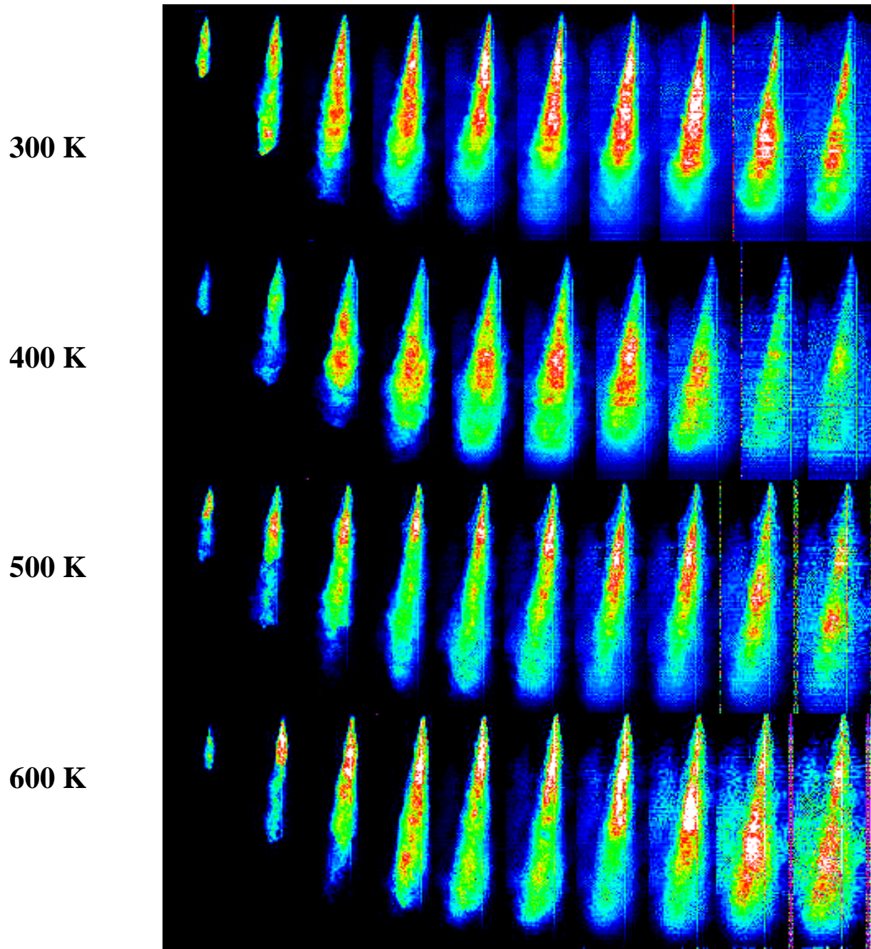
Figure 27: 125 MPa injection sequence into N 2 @ 3550 kPa
