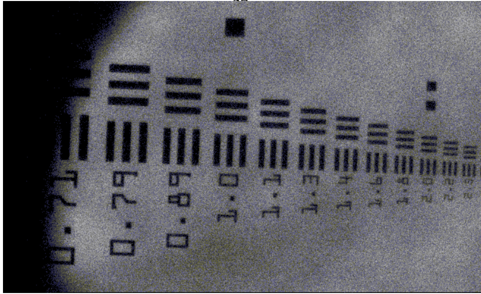
Figure 7: Resolution Grid used for determination of penetration distances.
