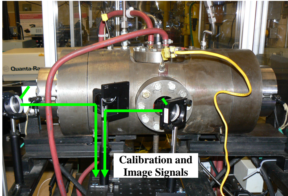
Figure 9: Optical setup for simultaneous imaging of calibration signal and spray image.
