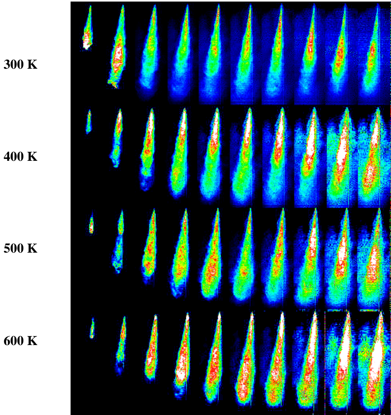
Figure 28: 150 MPa injection sequence into N 2 @ 3550 kPa
