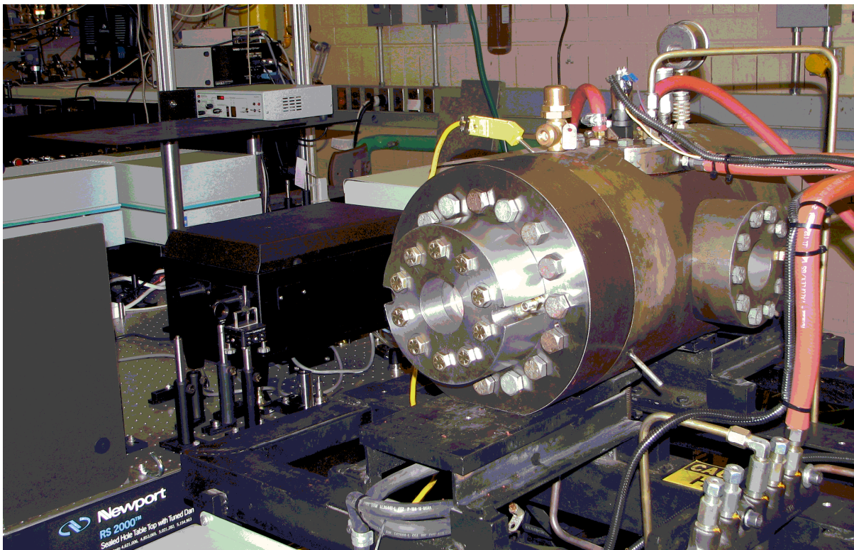
Figure 4: Constant Volume Combustion Vessel at Iowa State University.
