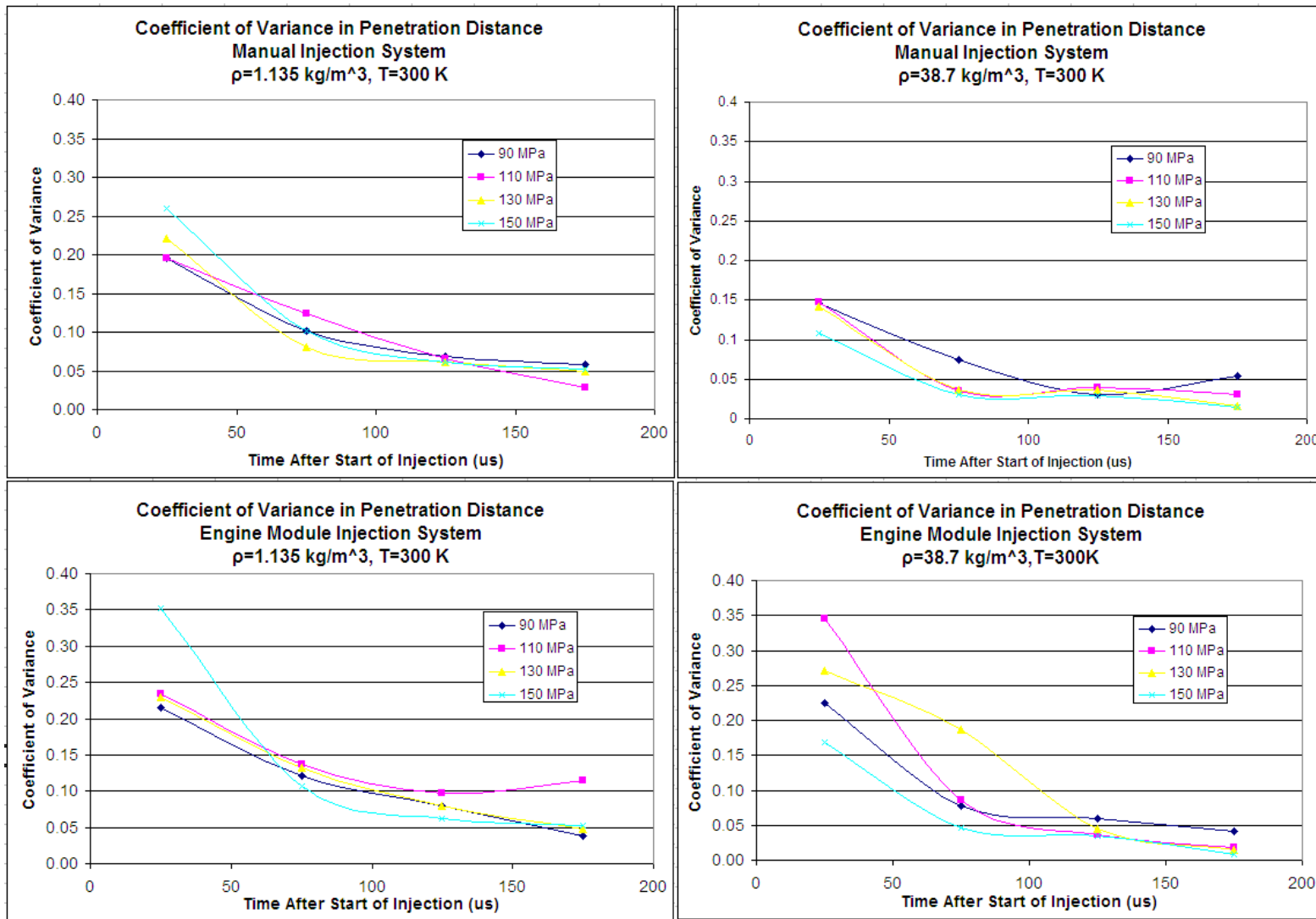
Figure 14: Coefficient of Variance in Penetration Distance for 90, 110, 130, and 150 MPa Fuel Injection Pressures, and Nitrogen Gas Densities of 1.135 and 38.7 kg/m 3 .
