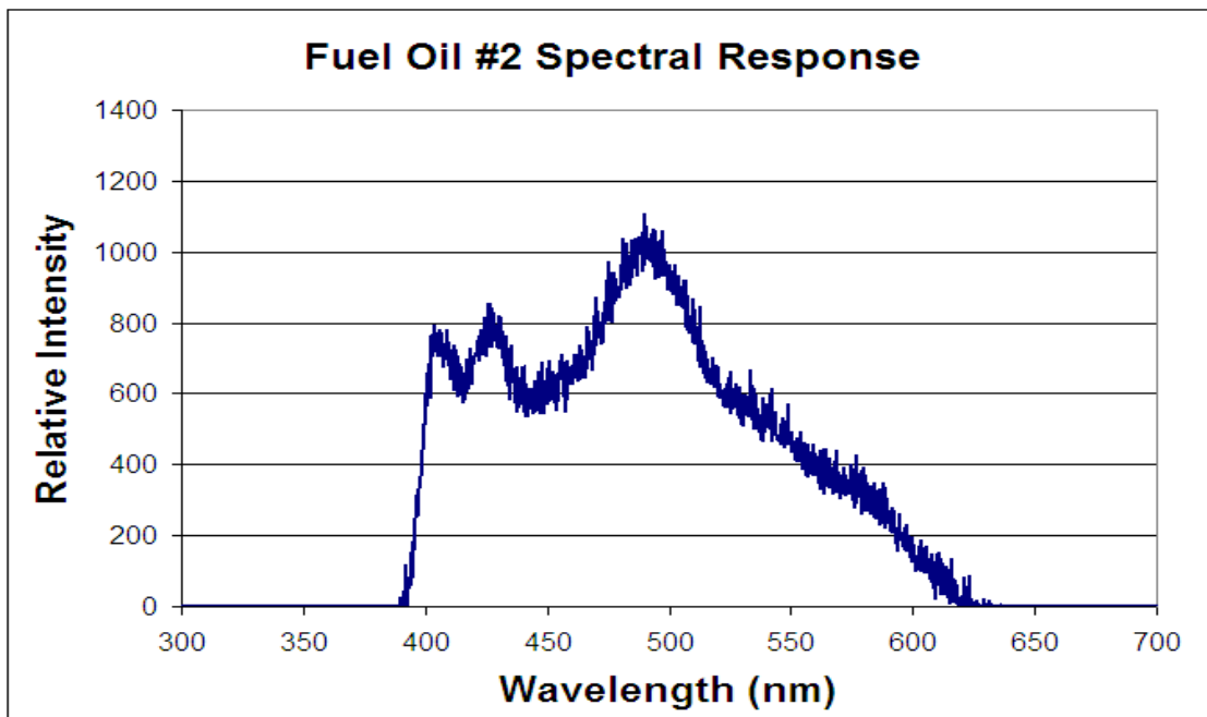
Figure 19: Spectral Response of Fuel Oil #2 with 355nm excitation and 400nm long-pass filter installed.
