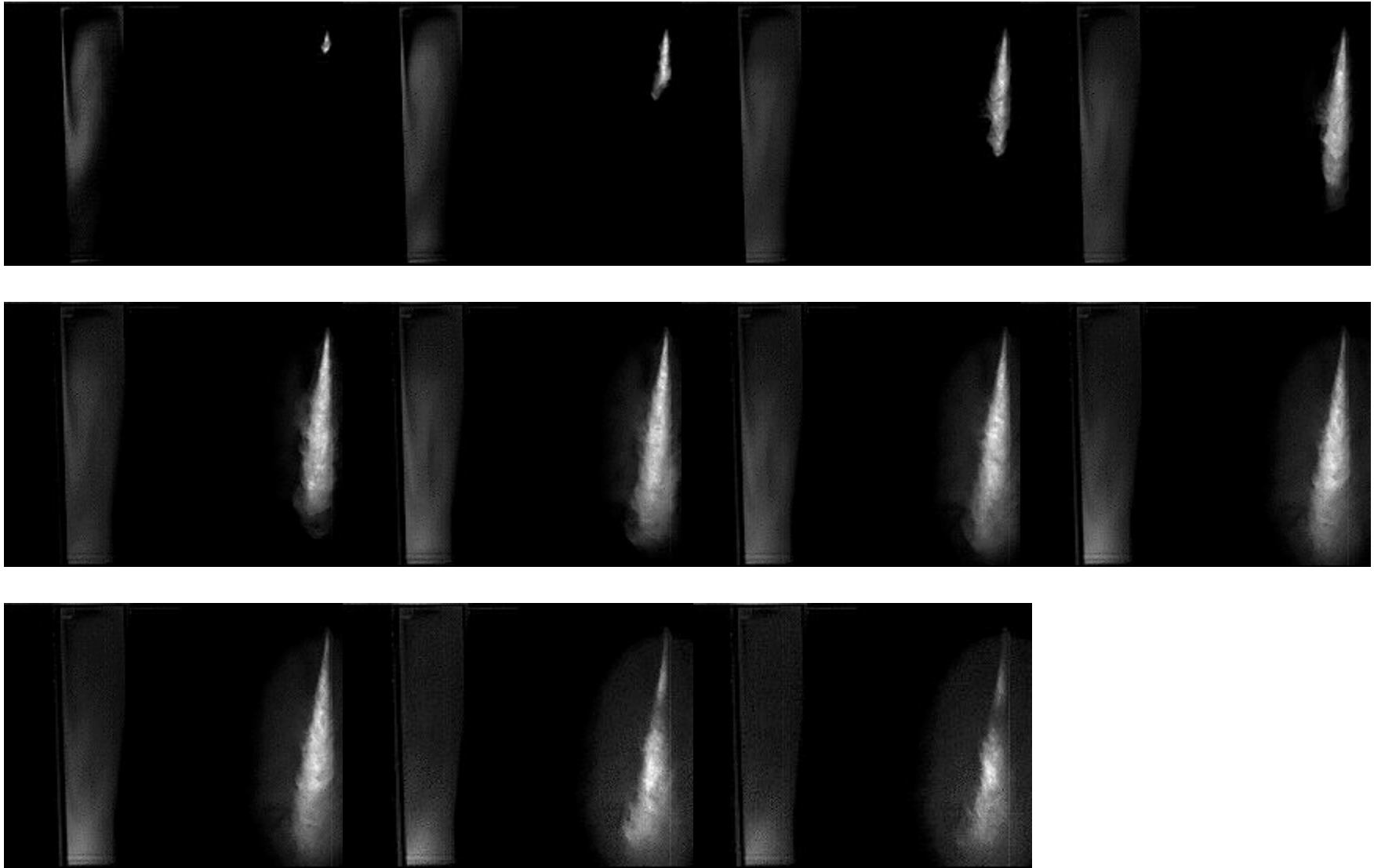
Figure 23: 100 MPa injection pressure into Nitrogen @ 3550 kPa for laser excitation at 10 kHz.
