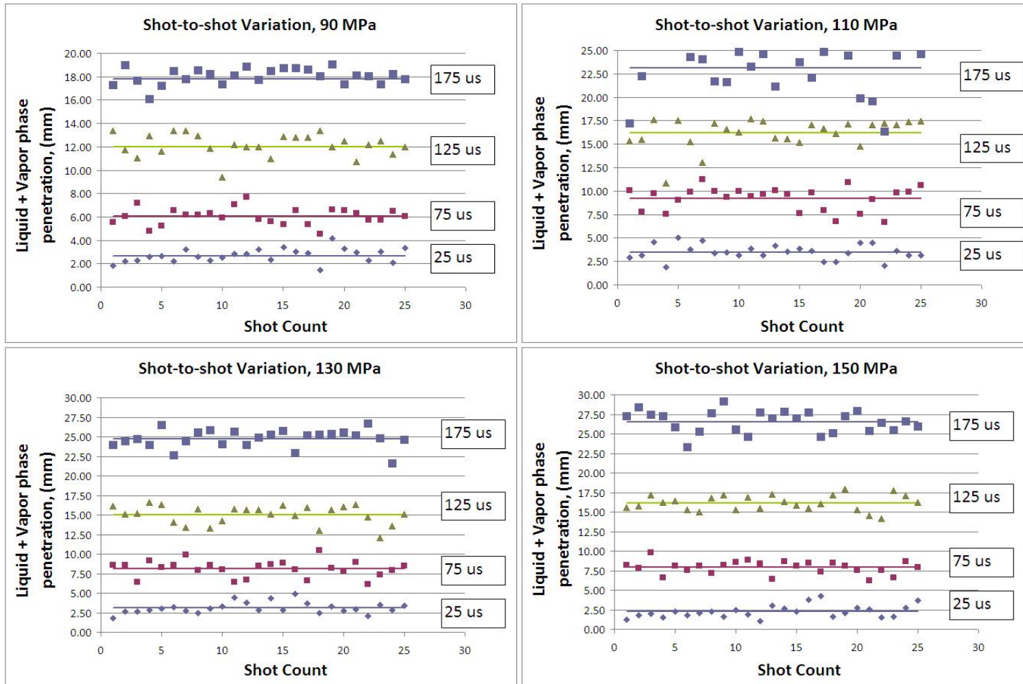
Figure 12: Shot-to-shot variation in penetration distance for the engine control module experimental setup
