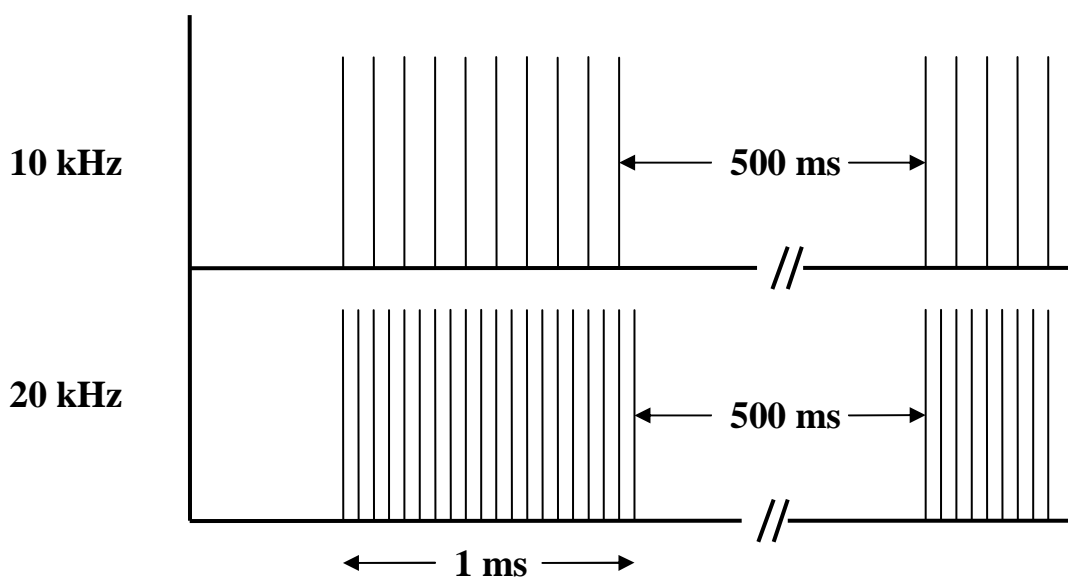
Figure 8: Pulse-Burst train timing configuration for 10 kHz and 20 kHz rates.
