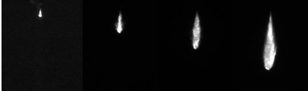
Figure 10: Sequence of Injection events at 25, 75, 125, and 175 us ASOI into nitrogen @ 1 atm
