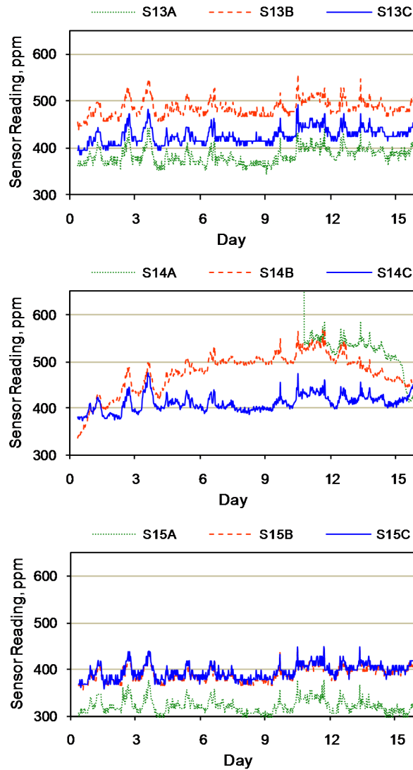
Figure 7. Power-up and conditioning of single-lamp dual-wavelength sensors.
