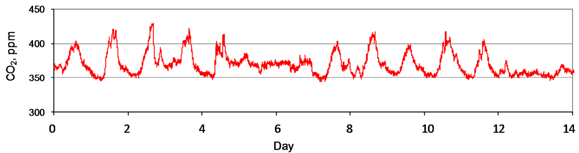
Figure 5. CO 2 concentration in the laboratory for two weeks prior to commencing the performance test.
