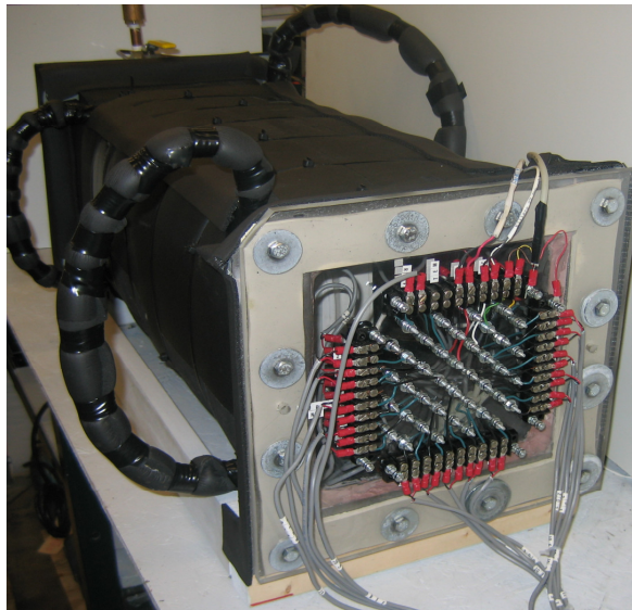
Figure 5. Photograph of the Lexan® end plate with connectors mounted on the test chamber.
