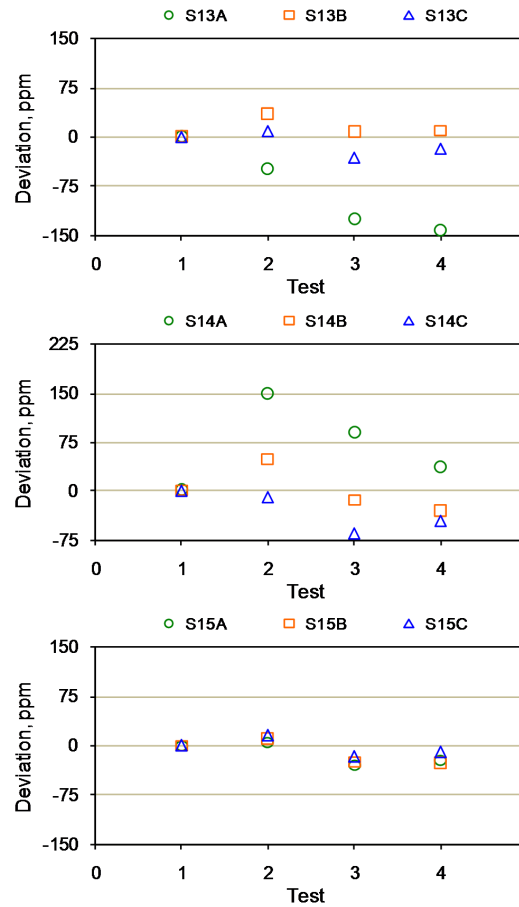
Figure 11. Deviation from the reading from the first test for single-lamp, dual-wavelength sensors.
