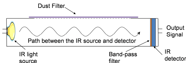
Figure 1. Schematic of a NDIR CO 2 sensor.
