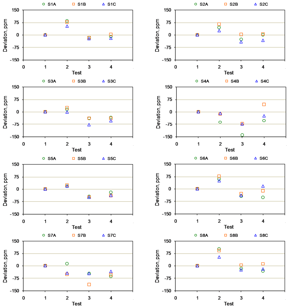
Figure 9. Deviation from the reading from the first test for single-lamp, single-wavelength sensors.
