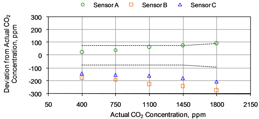
Figure 9. Comparison of mean deviation from actual CO 2 for three sensors of the same model.
