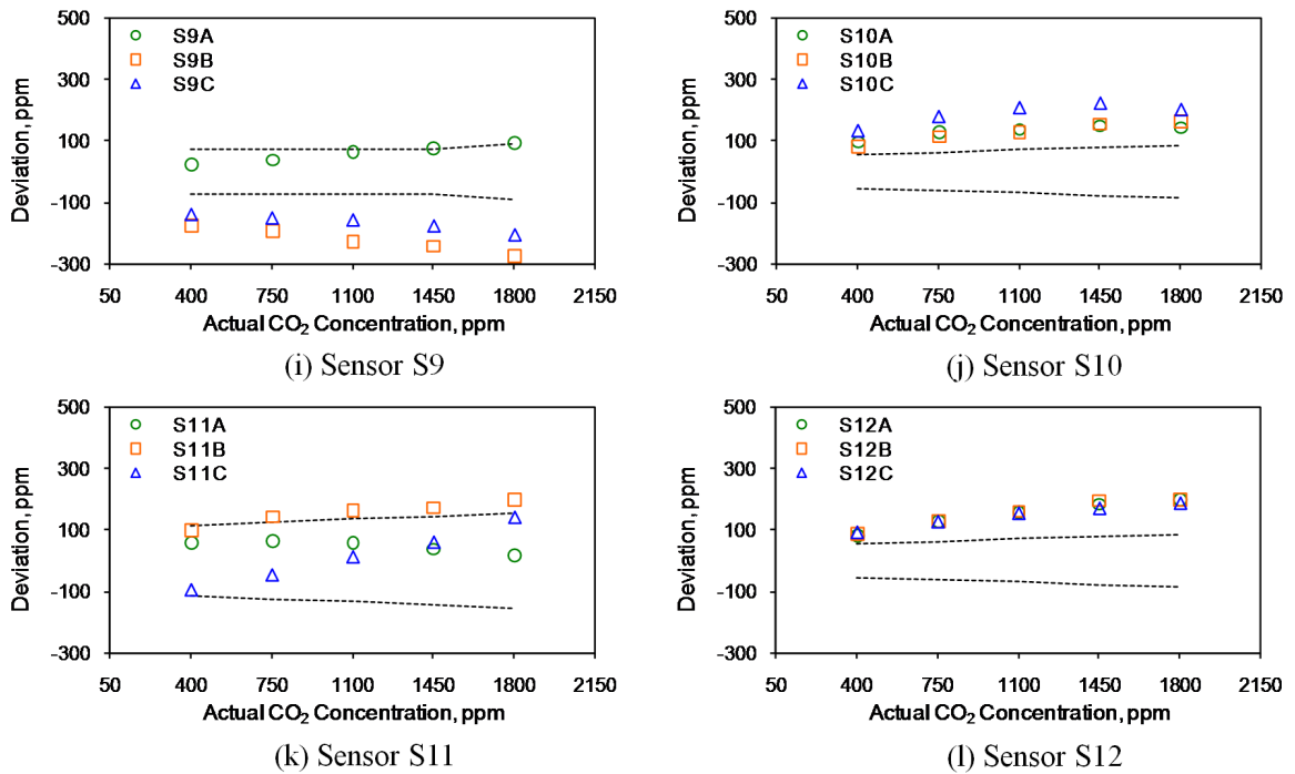
Figure 6. Comparison of deviation from actual CO 2 concentration of dual-lamp, single-wavelength sensors.
