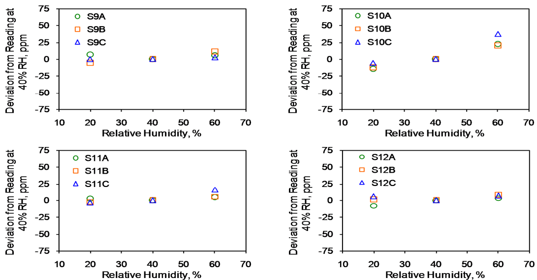
Figure 2. Humidity sensitivity test results of dual-lamp, single-wavelength sensors.
