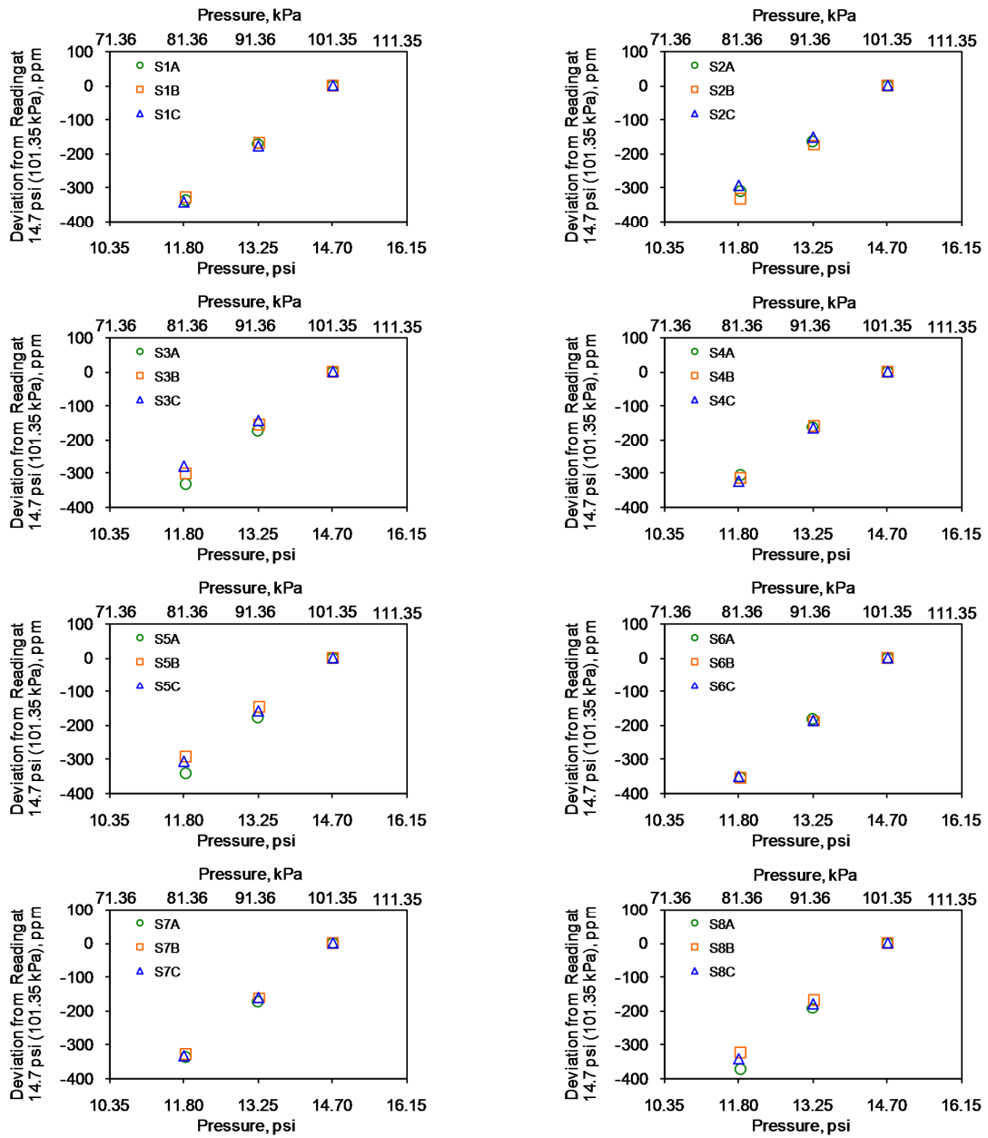
Figure 7. Pressure sensitivity test results of single-lamp, single-wavelength sensors.
