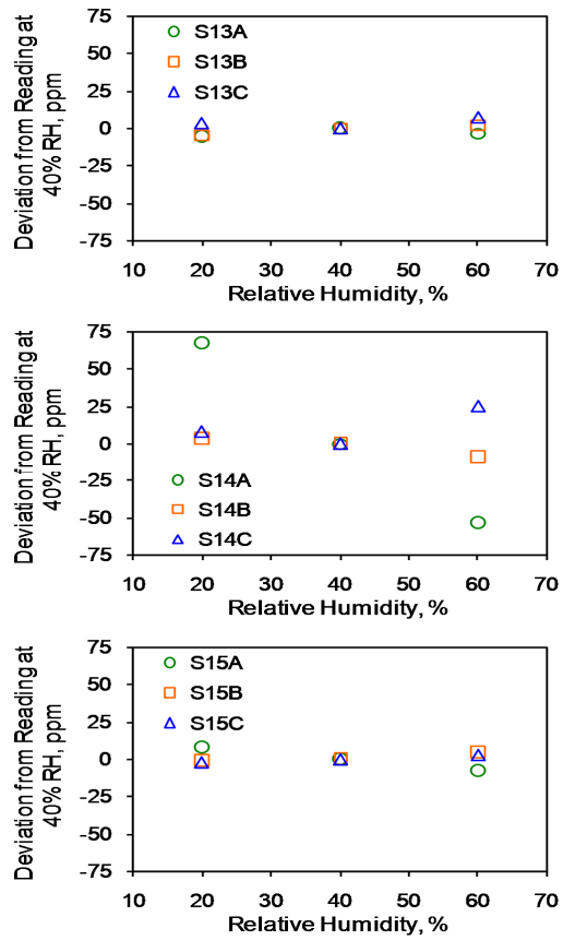
Figure 3. Humidity sensitivity test results of single-lamp, dual-wavelength sensors.
