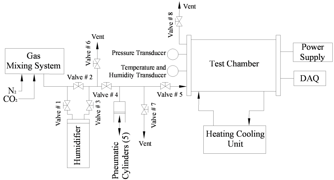
Figure 2. Schematic of the test system.
