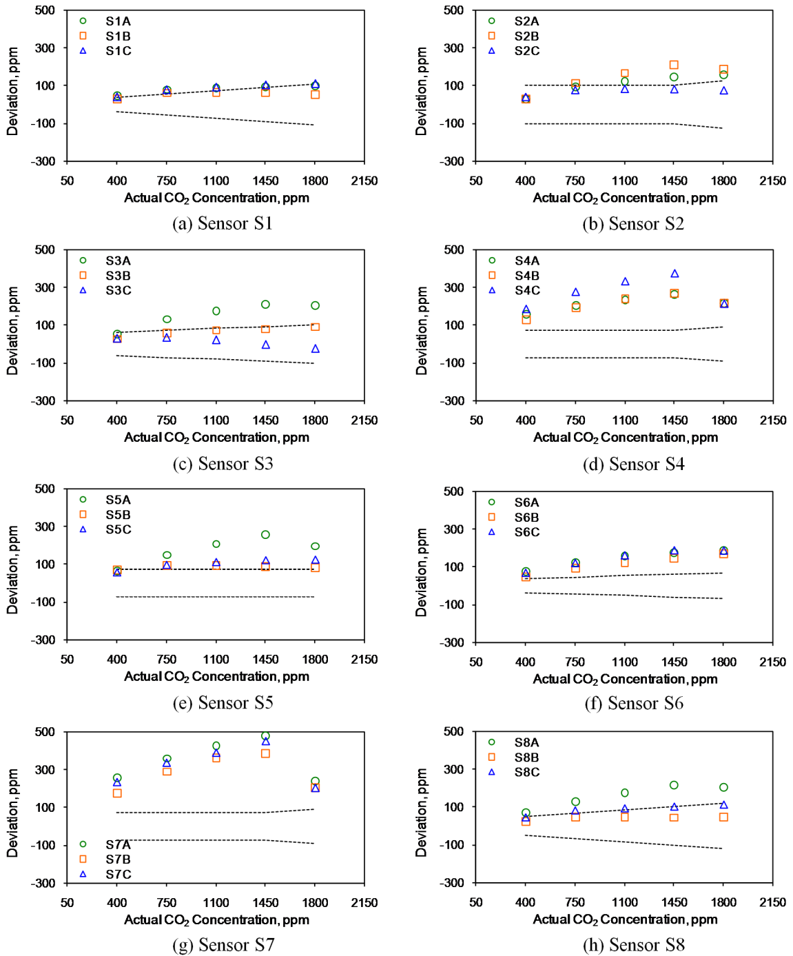
Figure 4. Comparison of deviation from actual CO 2 concentration of single-lamp, single-wavelength sensors.
