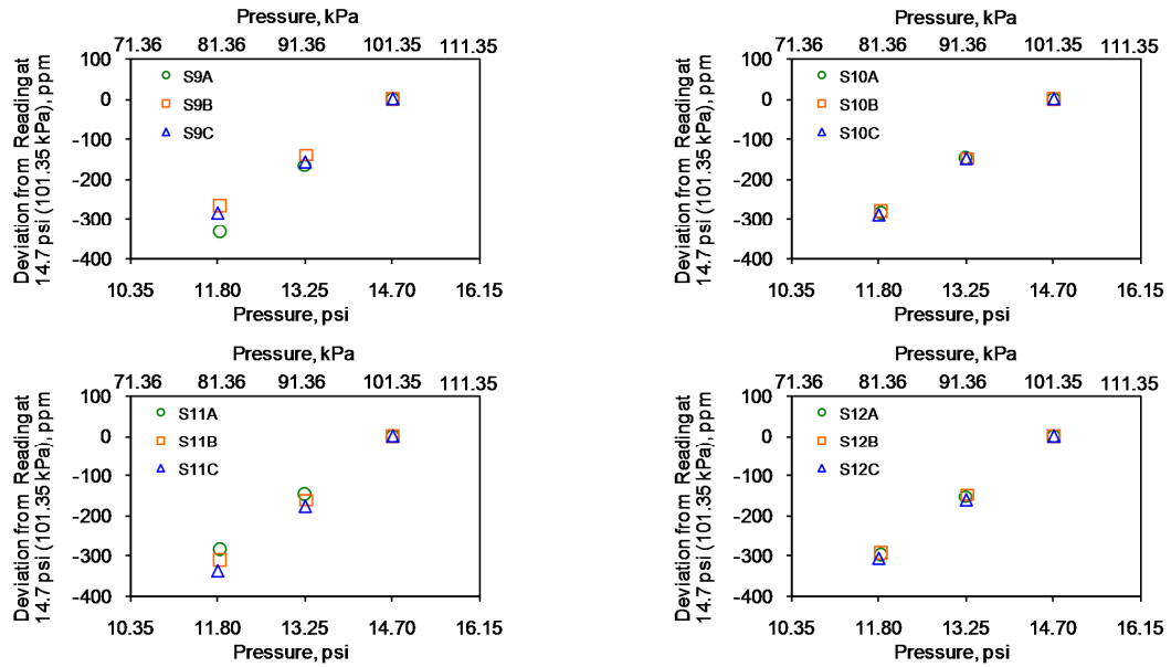
Figure 8. Pressure sensitivity test results of dual-lamp, single-wavelength sensors.
