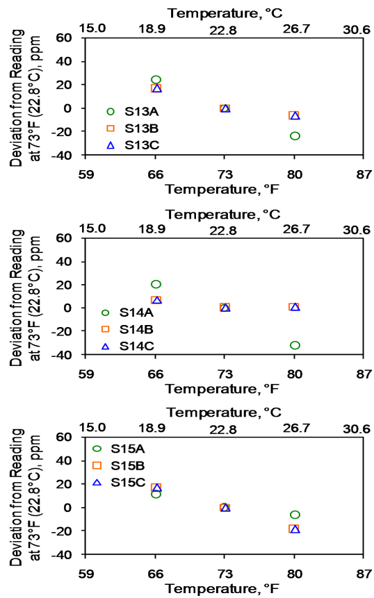
Figure 6. Temperature sensitivity test results of single-lamp, dual-wavelength sensors.
