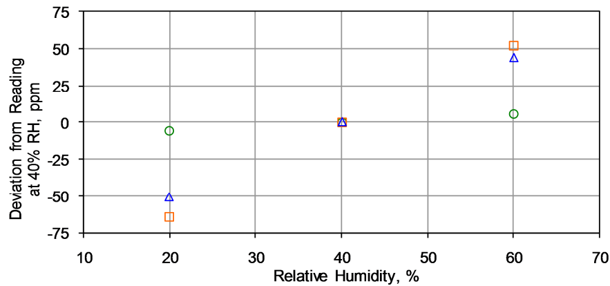
Figure 10. Humidity sensitivity of three different sensor models.
