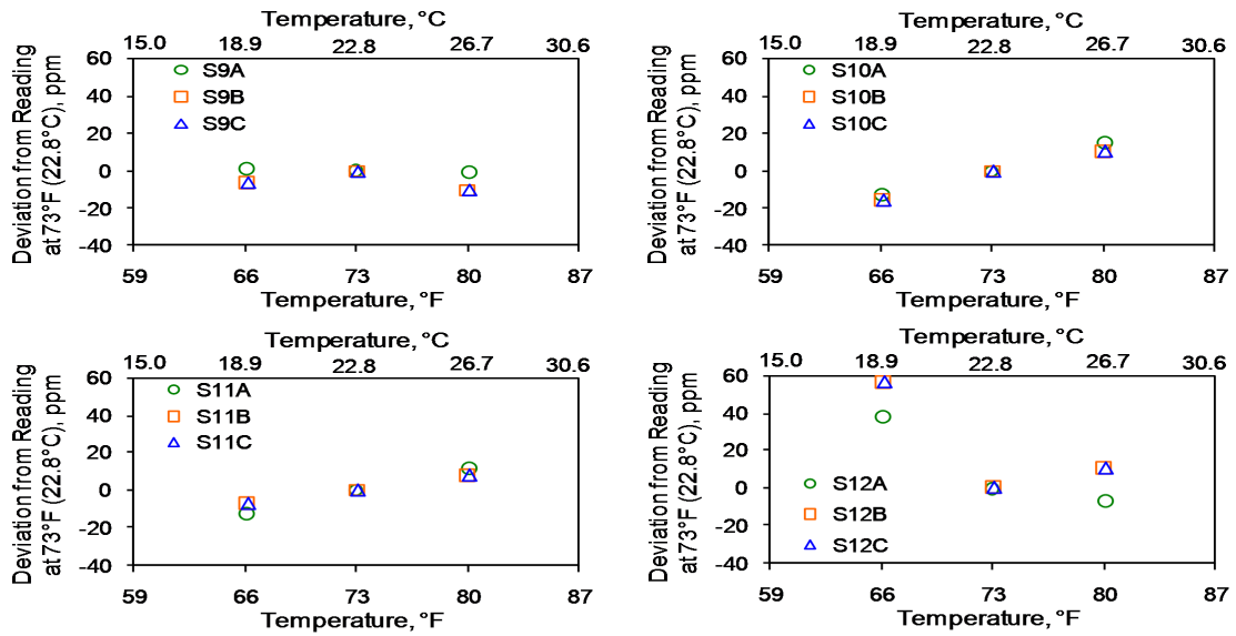
Figure 5. Temperature sensitivity test results of dual-lamp, single-wavelength sensors.
