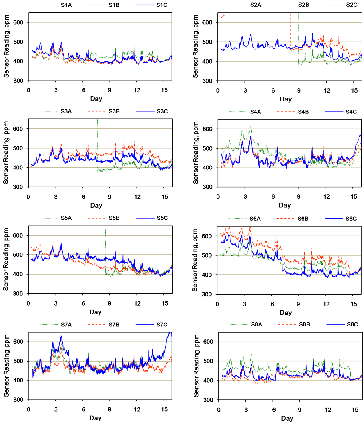
Figure 5. Power-up and conditioning of single-lamp, single-wavelength sensors.
