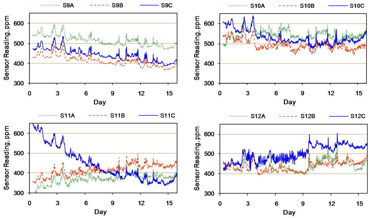
Figure 6. Power-up and conditioning of dual-lamp, single-wavelength sensors.
