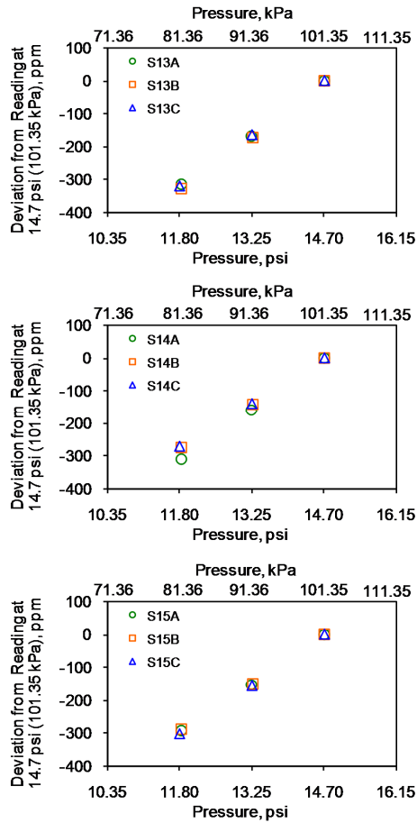
Figure 9. Pressure sensitivity test results of single-lamp, dual-wavelength sensors.
