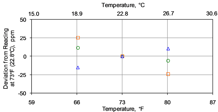
Figure 11. Temperature sensitivity of three different sensor models.
