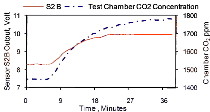
Figure 3. Saturated reading of S2B sensor at 1800 ppm.
