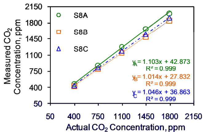
Figure 8. Example of a linearity plot.
