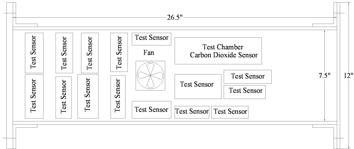
Figure 3. Test chamber interior.
