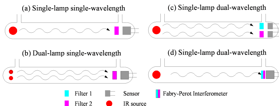
Figure 1. NDIR sensor configurations.
