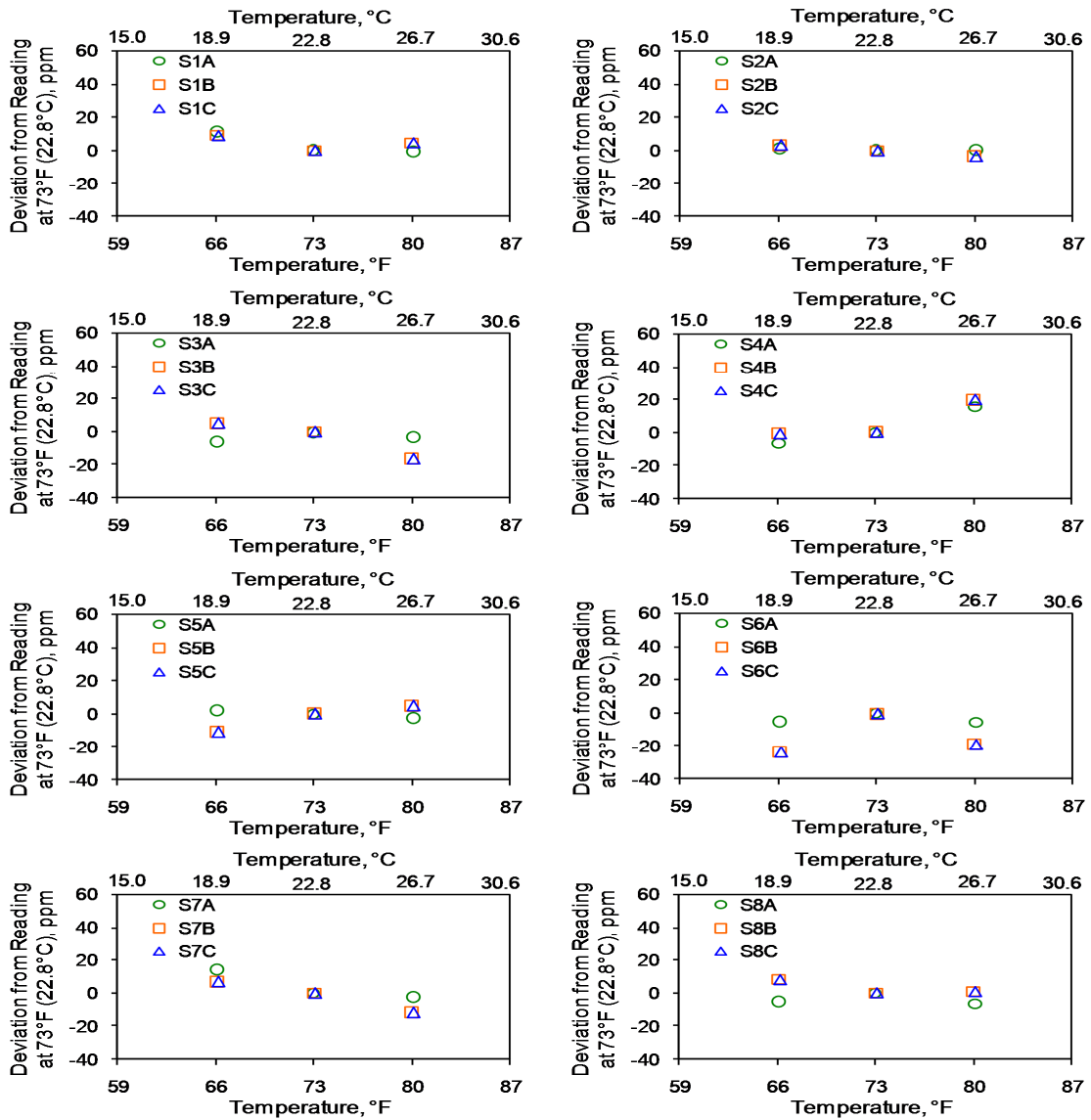
Figure 4. Temperature sensitivity test results of single-lamp, single-wavelength sensors.
