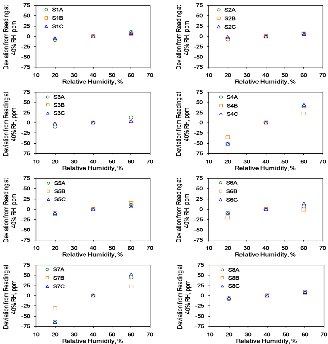
Figure 1. Humidity sensitivity test results of single-lamp, single-wavelength sensors.
