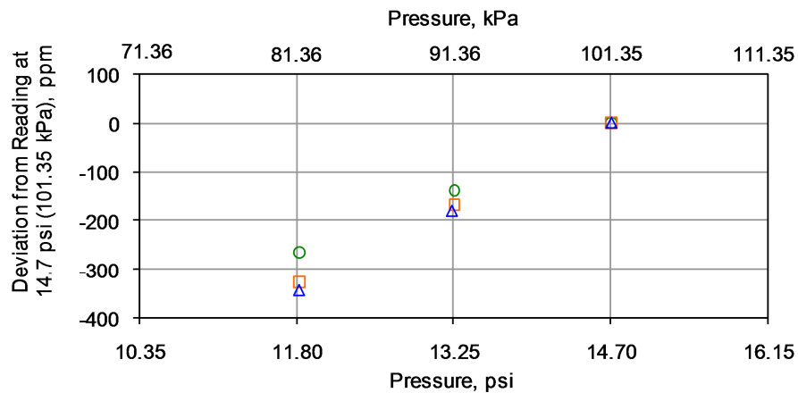
Figure 12. Pressure sensitivity of three different sensor models.
