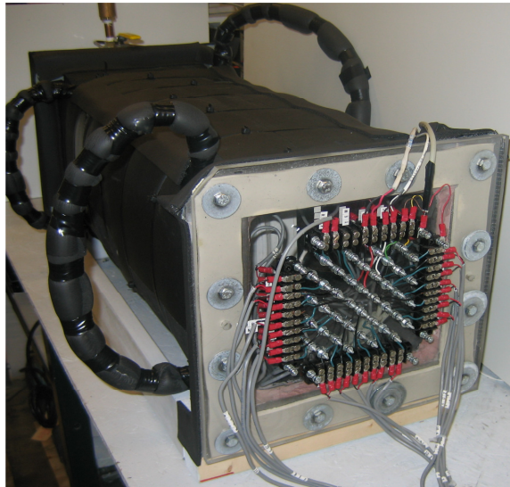
Figure 1. Test chamber.
