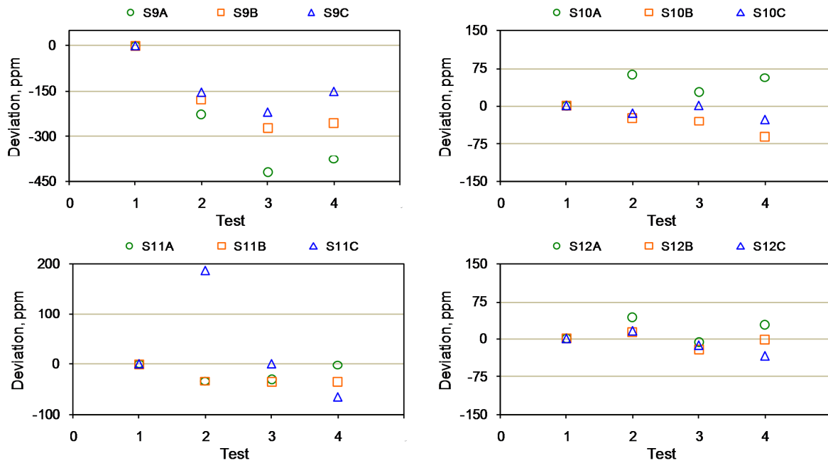
Figure 10. Deviation from the reading from the first test for dual-lamp, single-wavelength sensors.
