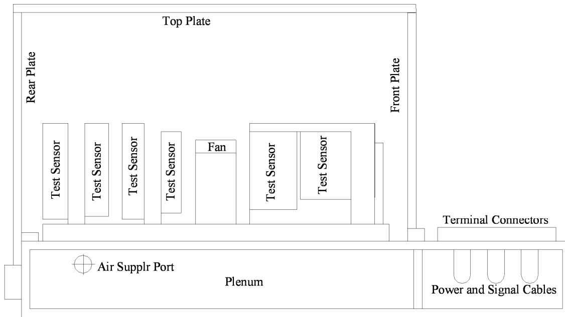
Figure 8. Schematic of the lab station.
