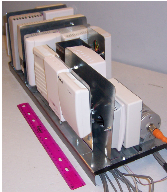
Figure 4. CO 2 sensors mounted on tray.
