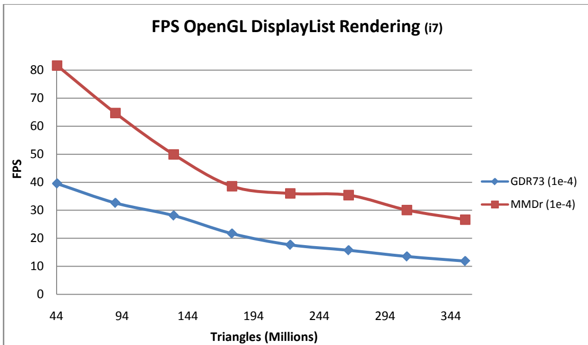
Figure 19: Render performance with a moderate amount of screen coverage culling
