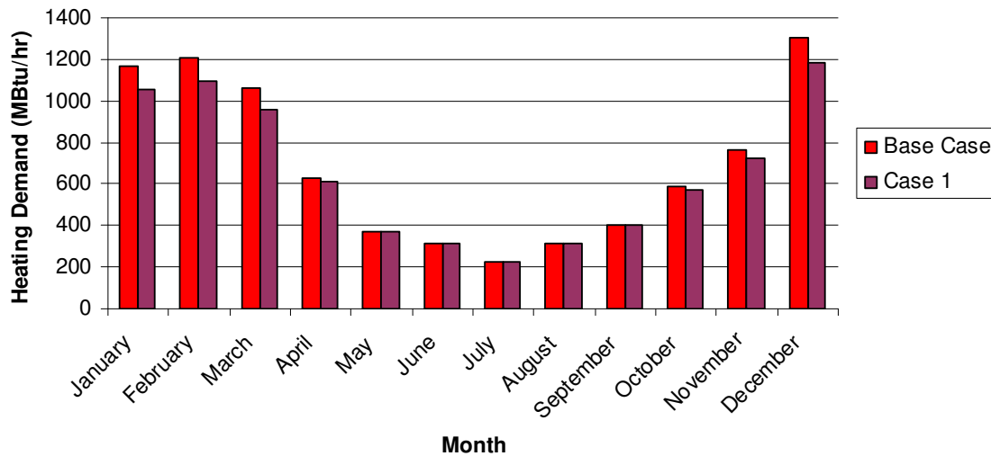
Figure 4.1 Average Monthly Heating Demand for Case 1 and the Base Case
