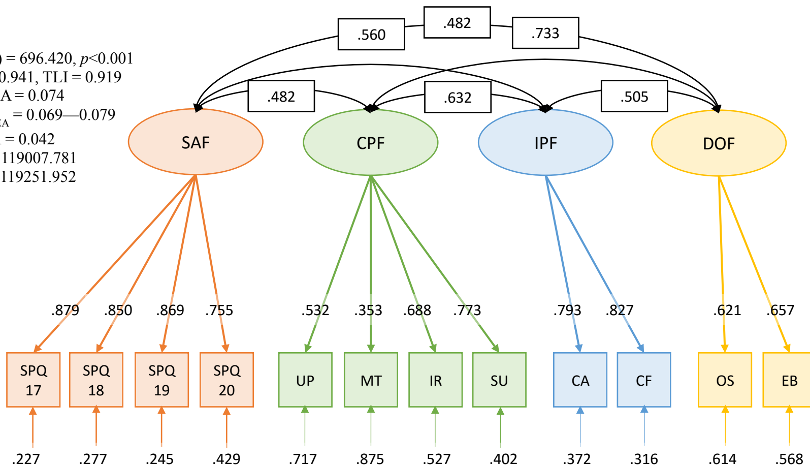
Figure 2b. Replication of Final CFA Solution of Latent Schizotypy (Parceled) with Standardized Factor Loadings (Aim 1).
