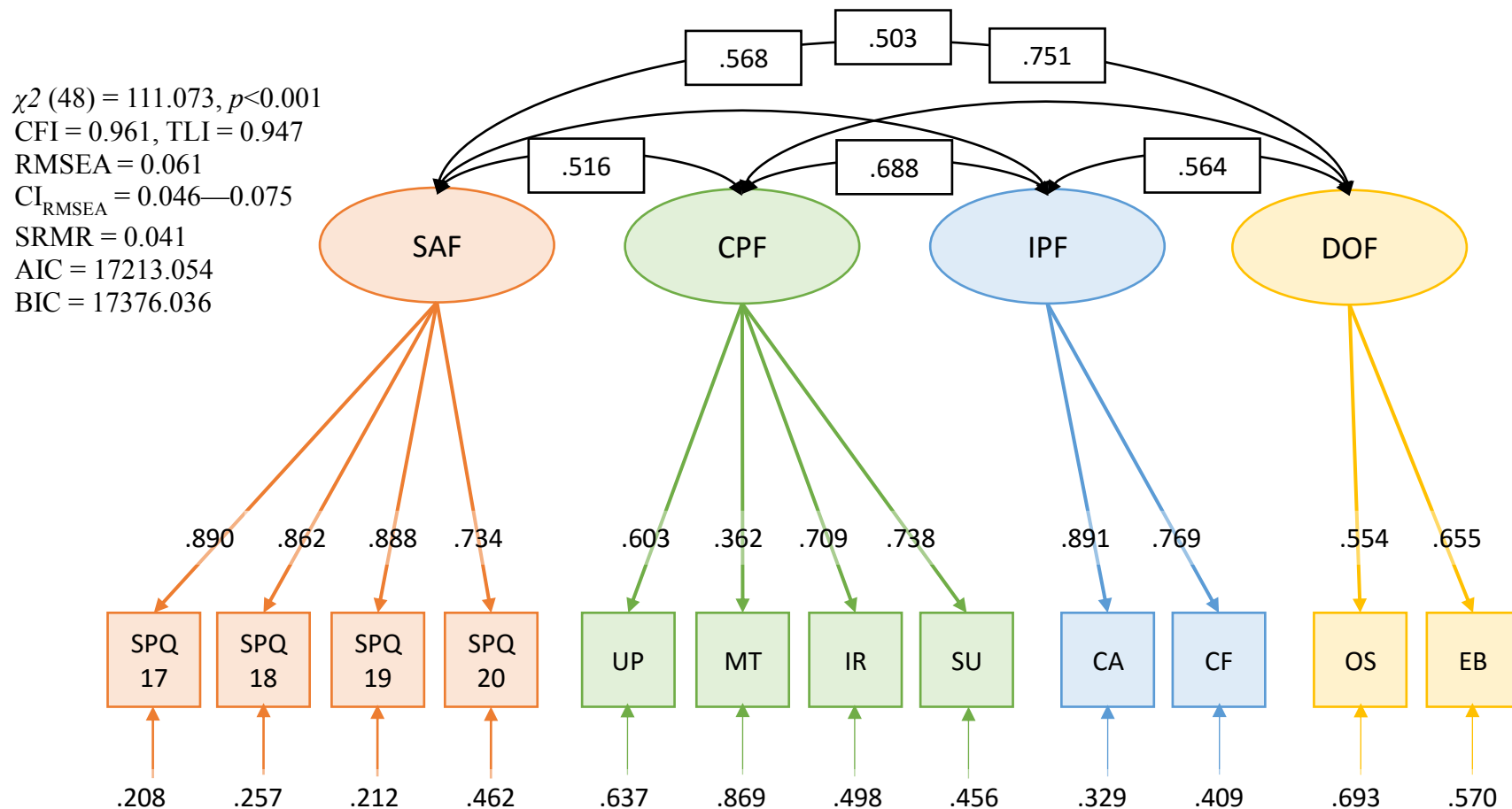
Figure 3. Replication of Final CFA Solution of Latent Schizotypy (Parceled) with Standardized Factor Loadings (Aim 2).
