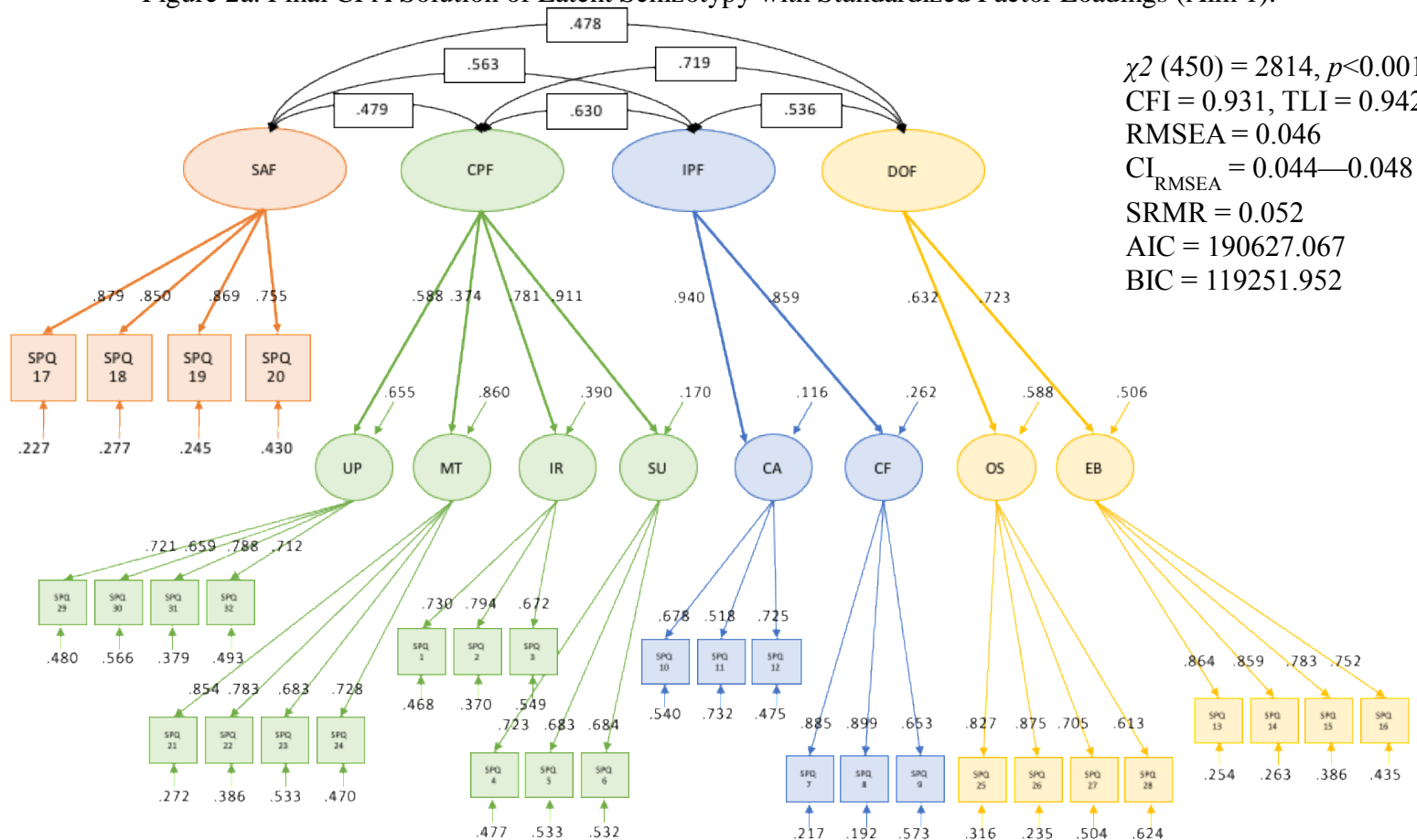
Figure 2a. Final CFA Solution of Latent Schizotypy with Standardized Factor Loadings (Aim 1).
