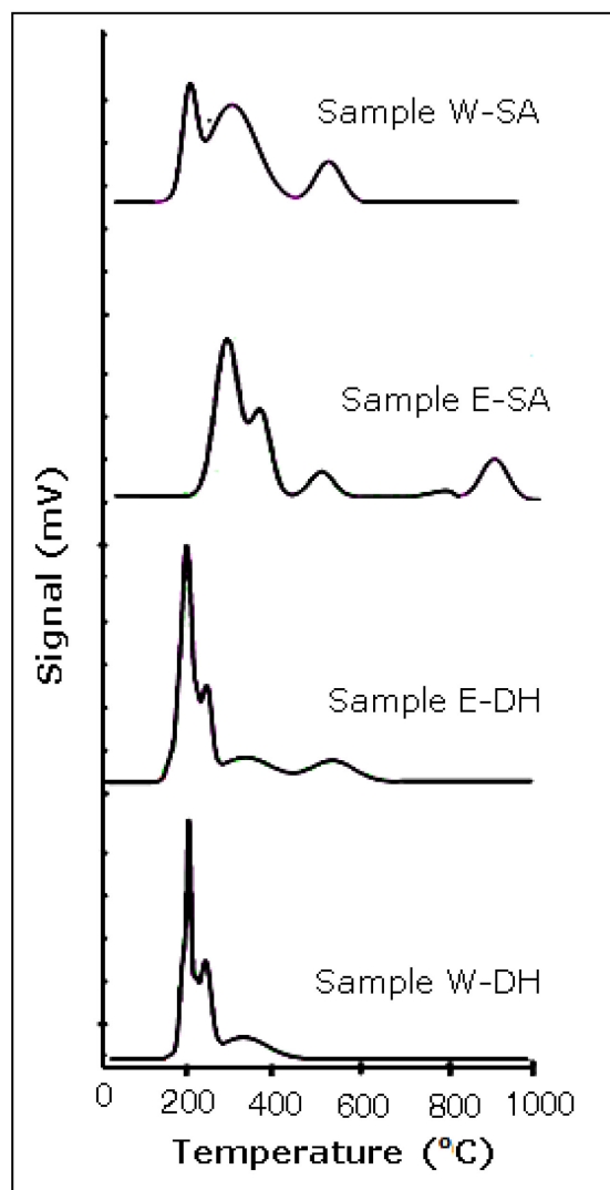
Figure 2.06. Smoothened TPR profile of all catalyst samples, ramp rate = 5K/min
