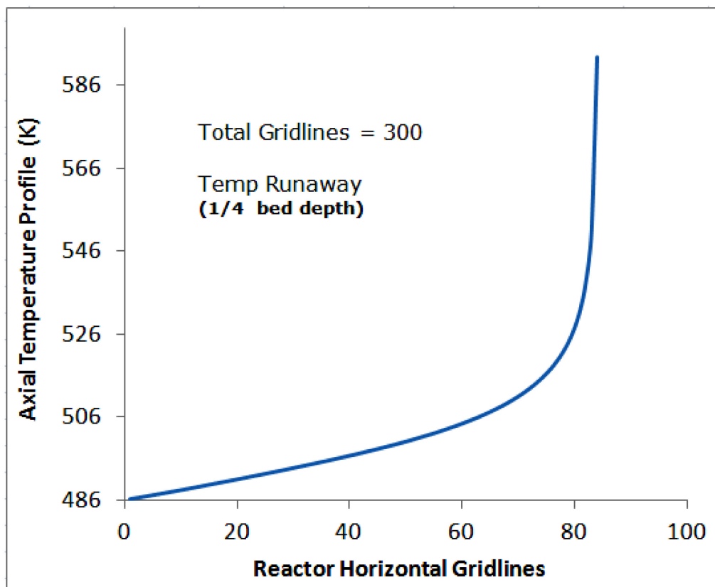
Figure 4.23. Temperature profile of reactor centerline during the startup. Catalyst pores are empty and gas inlet temperature, T_{\text{inlet}} = 486 K. This profile clearly indicates temperature runaway at approximately quarter bed length
