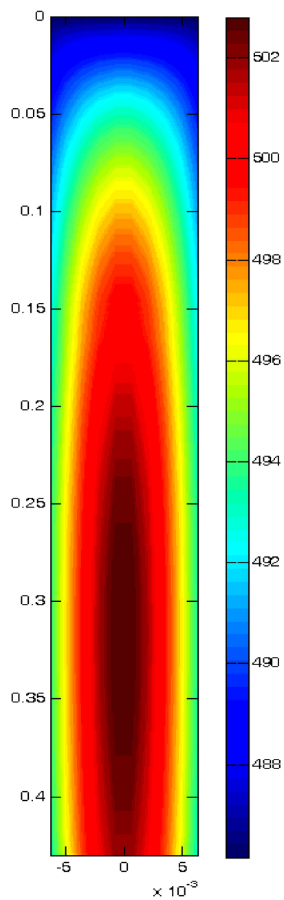
Figure 4.22. The contour plot of temperature in a fixed bed reactor. T_{\text{in}} = T_{\text{cool}} = 486\text{K} . As expected from the results in Figure 4.14 a-d, temperature increases down the bed and hot spot is located at the bottom half of the reactor
