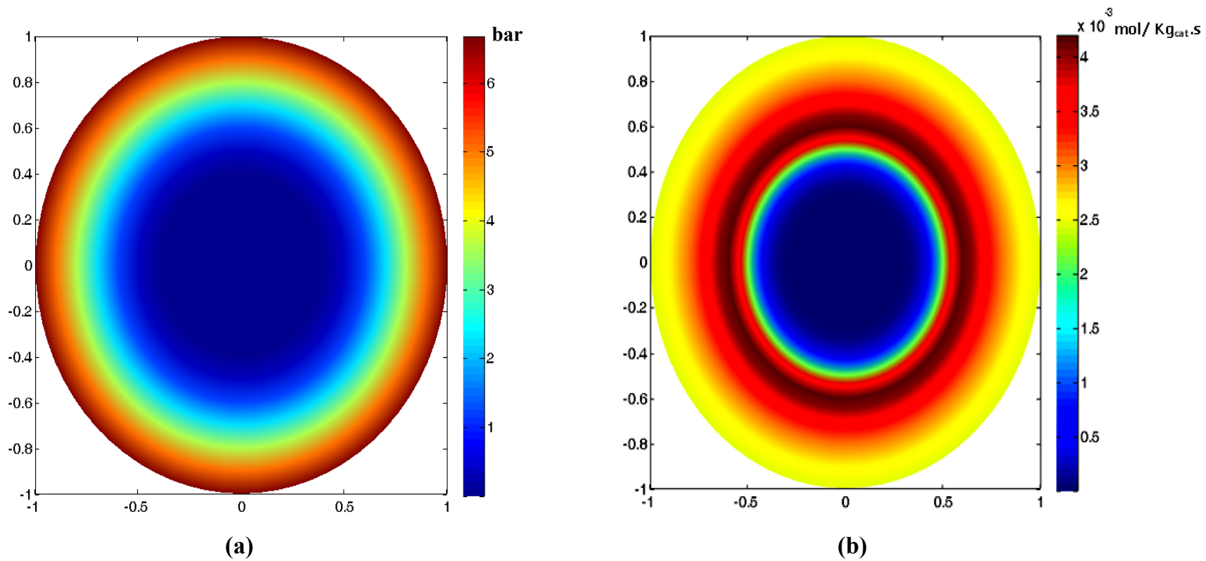
Figure 4.06. (a) Cutaway slice of a spherical catalyst showing concentration profile from its surface to the center of pellet (b) same slice showing the rate of consumption of CO. Process conditions at the surface are; pellet dia = 2 mm, T = 490 \text{ K} , P = 20 \text{ bar} , \text{H}_2/\text{CO} ratio = 2
