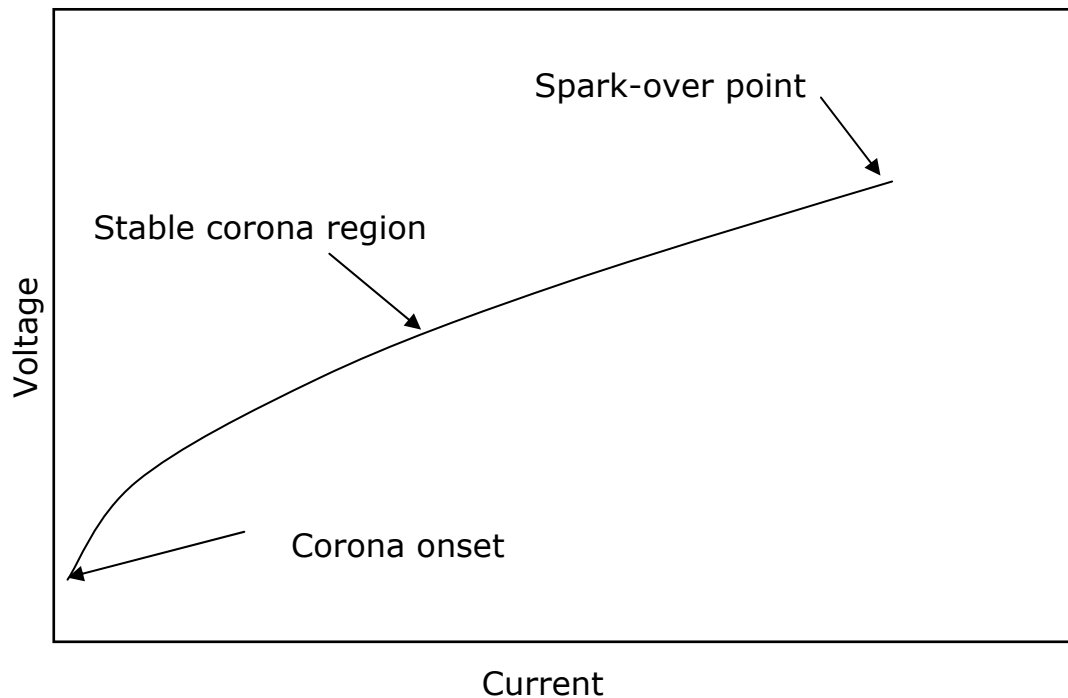
Figure 1.2: Typical voltage-current curve for a DC corona discharge [58].
