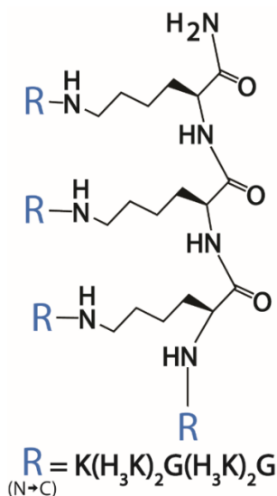
Figure 1.1 Structure of HK peptide , showing a three lysine core and the amino acid sequence of each branch.
