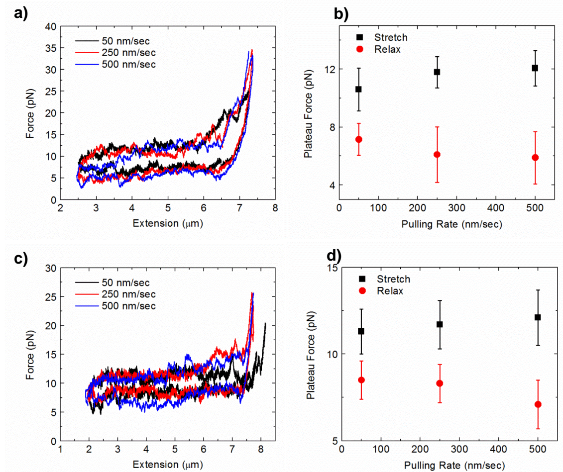
Figure 2.4 The effect of a pulling speed on a plateau force. (a) For DNA:HK complexes, variation of the pulling rate from 50 nm/sec to 500 nm/sec showed a decrease in the relax plateau force and an increase in the stretch plateau force. (b) Stretch plateau forces for 50 nm/sec, 250 nm/sec, and 500 nm/sec are 10.60 \pm 1.47 pN, 11.78 \pm 1.08 pN, and 12.05 \pm 1.22 pN respectively. Relaxation plateau forces for 50 nm/sec, 250 nm/sec, and 500 nm/sec are 7.15 \pm 1.11 pN, 6.10 \pm 1.91 pN, and 5.88 \pm 1.81 pN respectively. (c) For DNA:PLL complexes, variation of the pulling rate from 50 nm/sec to 500 nm/sec showed a decrease in the relax plateau force and an increase in the stretch plateau force. (d) Stretch plateau forces for 50 nm/sec, 250 nm/sec, and 500 nm/sec are 11.29 \pm 1.27 pN, 11.66 \pm 1.38 pN, and 12.06 \pm 1.59 pN respectively. Relaxation plateau forces for 50 nm/sec, 250 nm/sec, and 500 nm/sec are 8.50 \pm 1.10 pN, 8.32 \pm 1.08 pN, and 7.10 \pm 1.41 pN respectively.
