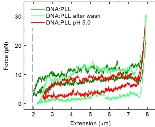
Figure 2.6 The effect of pH on the force profiles of DNA:PLL complex. DNA is condensed with 1 \mu\text{M} PLL (dark green) in tris buffer (pH 7.4). After washing with peptide free buffer (light green), the force profile for this particular experiment exhibits a single plateau in the relax curve. The overall features of the PLL force profile remained similar in the presence of acetate buffer (pH 5) with a decreased hysteresis, showing no significant effect of low pH on their force profiles as observed in HK.
