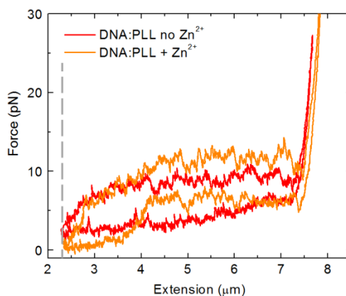
Figure 2.8 The effect of \text{Zn}^{2+} on the mechanical properties of DNA:PLL complex. Addition of 1 mM \text{Zn}^{2+} did not result in shortening of contour length for a DNA:PLL complex. The stretch plateau in the presence of \text{Zn}^{2+} is at 11.1 \pm 0.3 pN, and the relax plateau is 6.3 \pm 0.5 pN ( n = 3 ).
