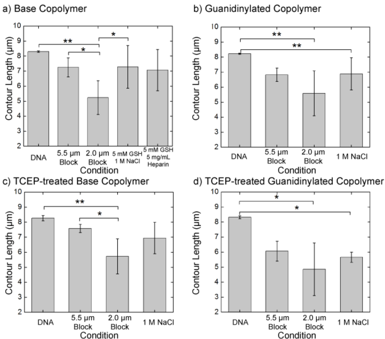
Figure 4.9 Contour length as a function of condensing agent and condition. (Tukey honest significance difference test, * p < 0.05 , ** p < 0.01 )
